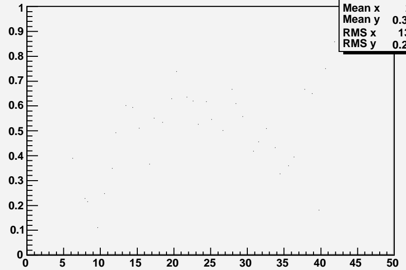
Efficiencies per detector of V2 Right
