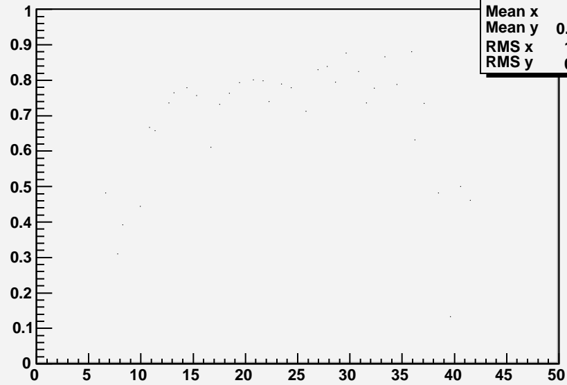
Efficiencies per detector of V2 Left
