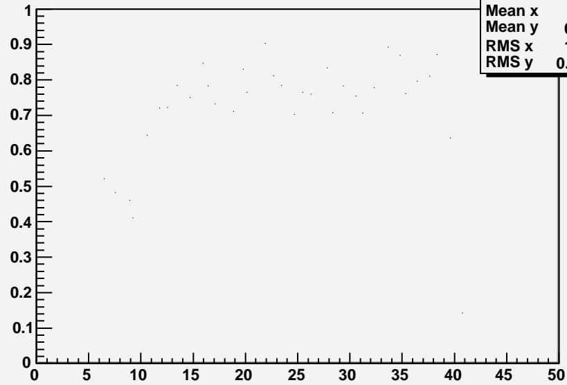
Efficiencies per detector of V1 Left
