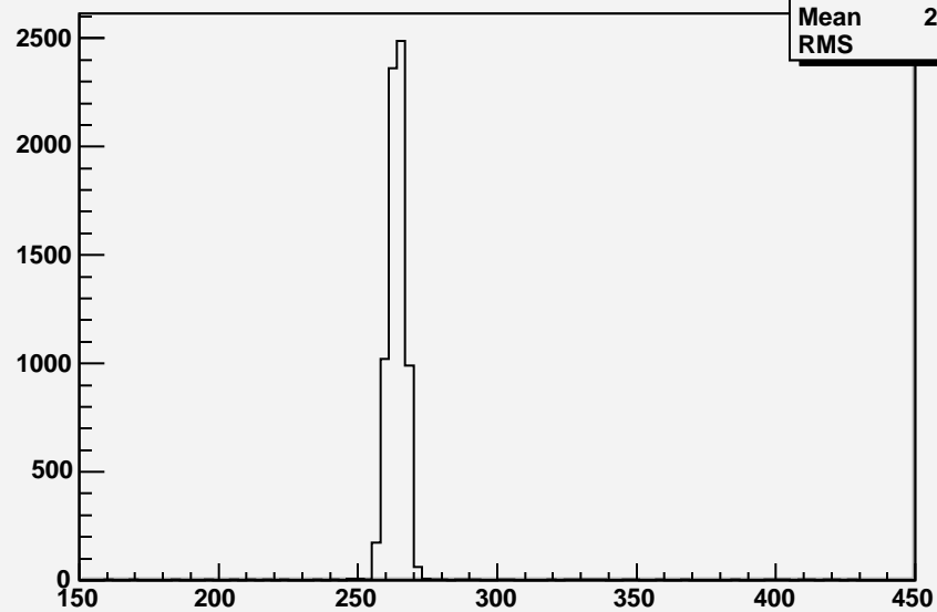
V1 at V2 peak
