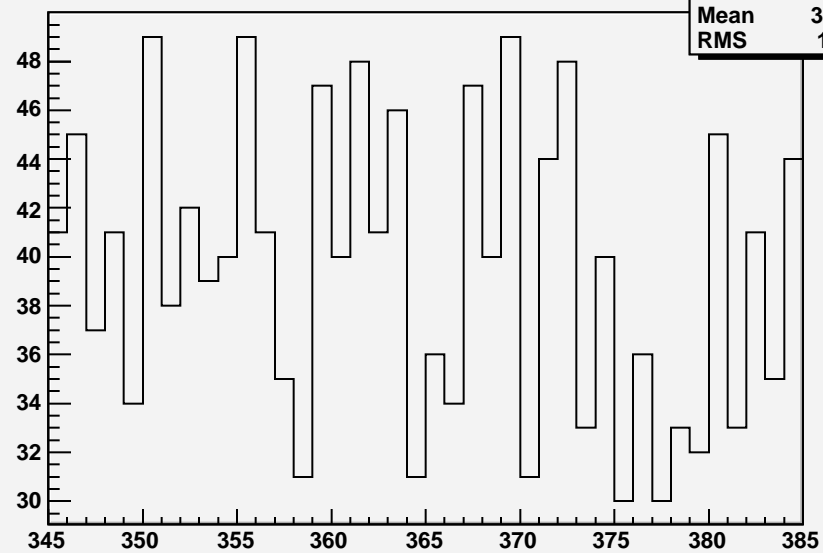
V1 Background with V2 Coinc
