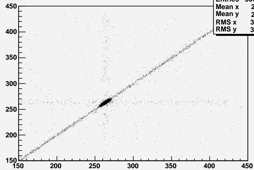
Corrected V2 vs Corrected V1
