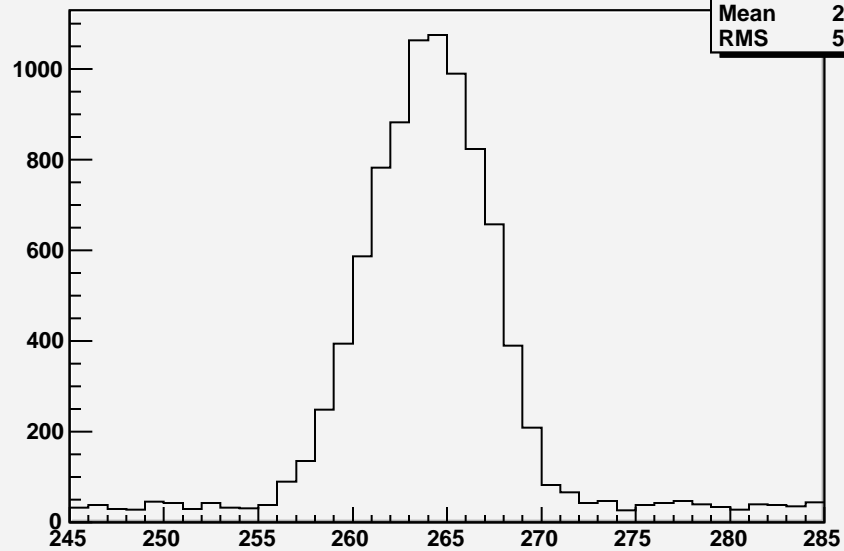
V2 about Peak
