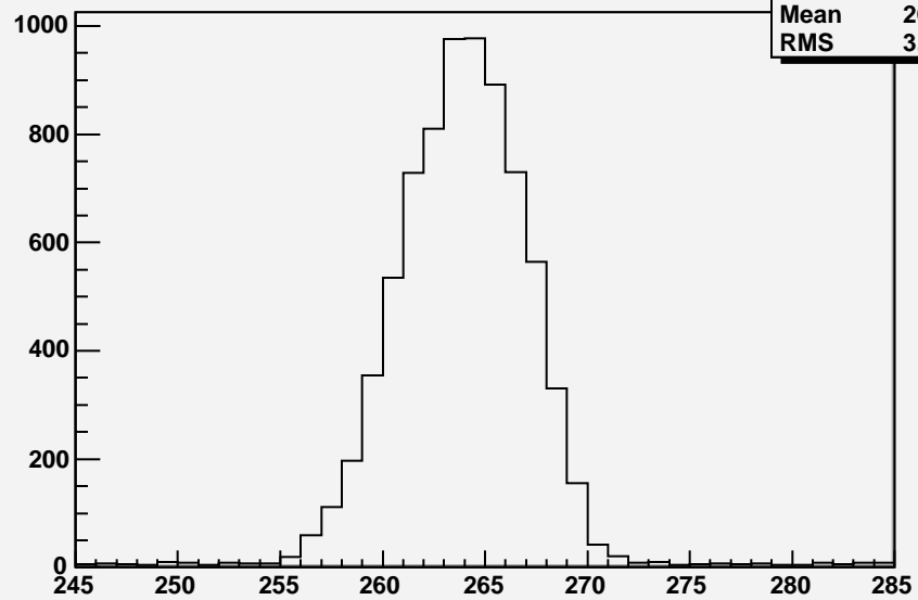
V2 about Peak with V1 Coinc
