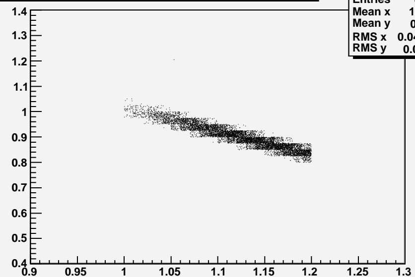
Measured Electron Momentum vs Virtual Photon Angle
