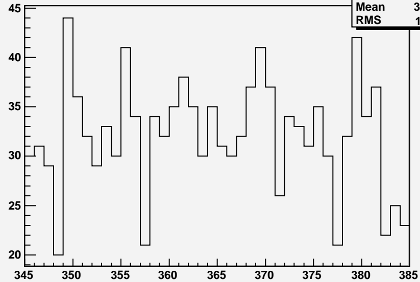
V2 Background with V1 Coinc
