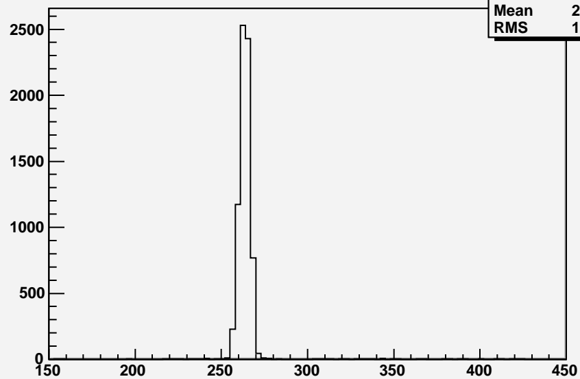
V2 at V1 peak
