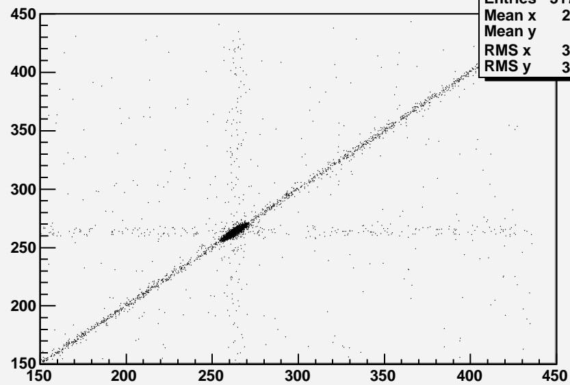
Corrected V1 vs Corrected V2
