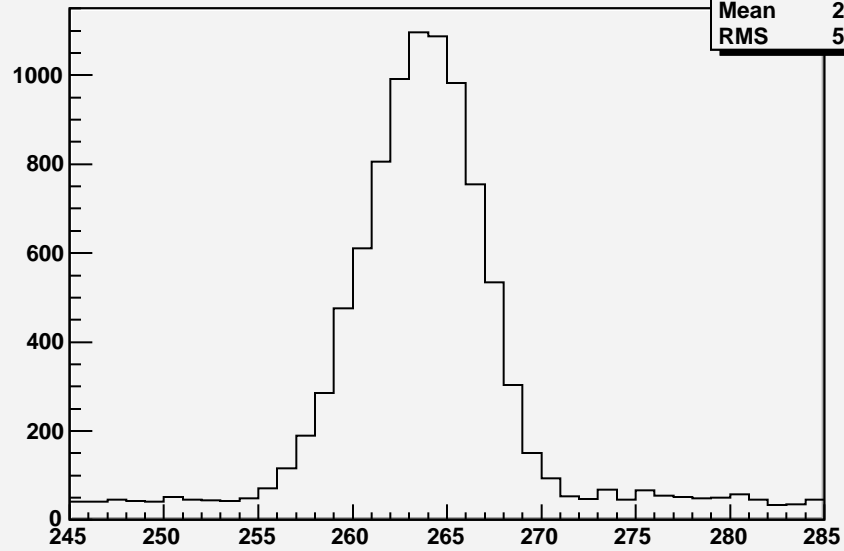
V1 about Peak
