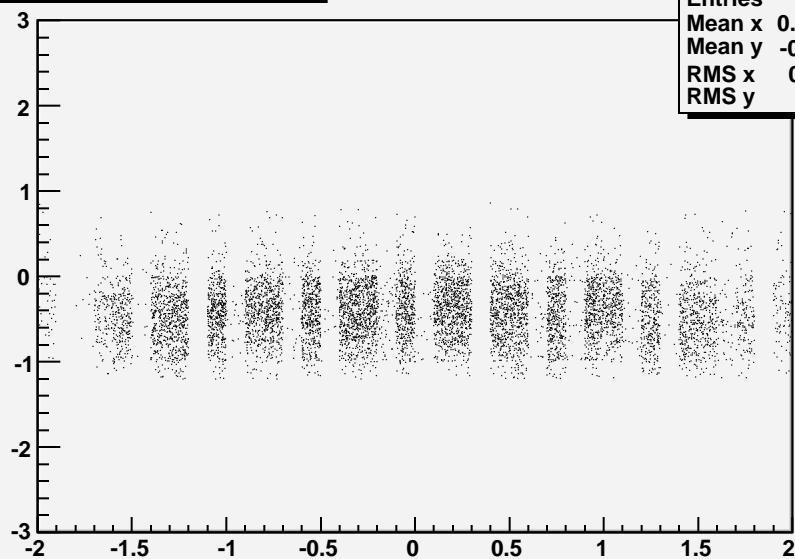
X position vs Y position
