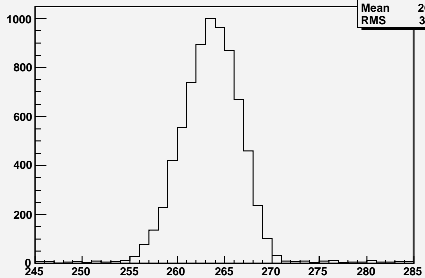
V1 about Peak with V2 Coinc
