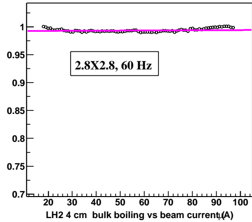
Figure 14: Bulk effect: relative ADC peak values (Lumi 1, normalized to beam current) vs. Beam Current for various configurations. Simple linear fits are shown, normalized to 1 at 20 \mu A. Data shown are for Lumi 1. The raster settings and fan speeds are indicated.
