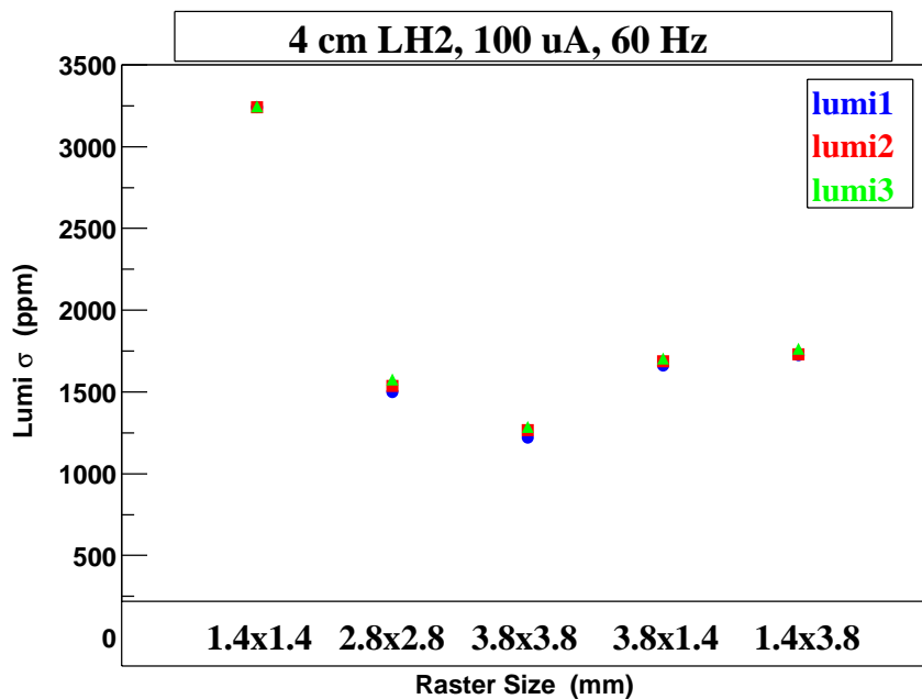
Figure 26: 4 cm LH_2 Lumi Sigma vs. Raster Size.
