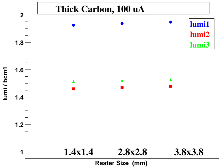
Figure 22: Carbon target Lumi Bulk Effect vs. Raster Size.
