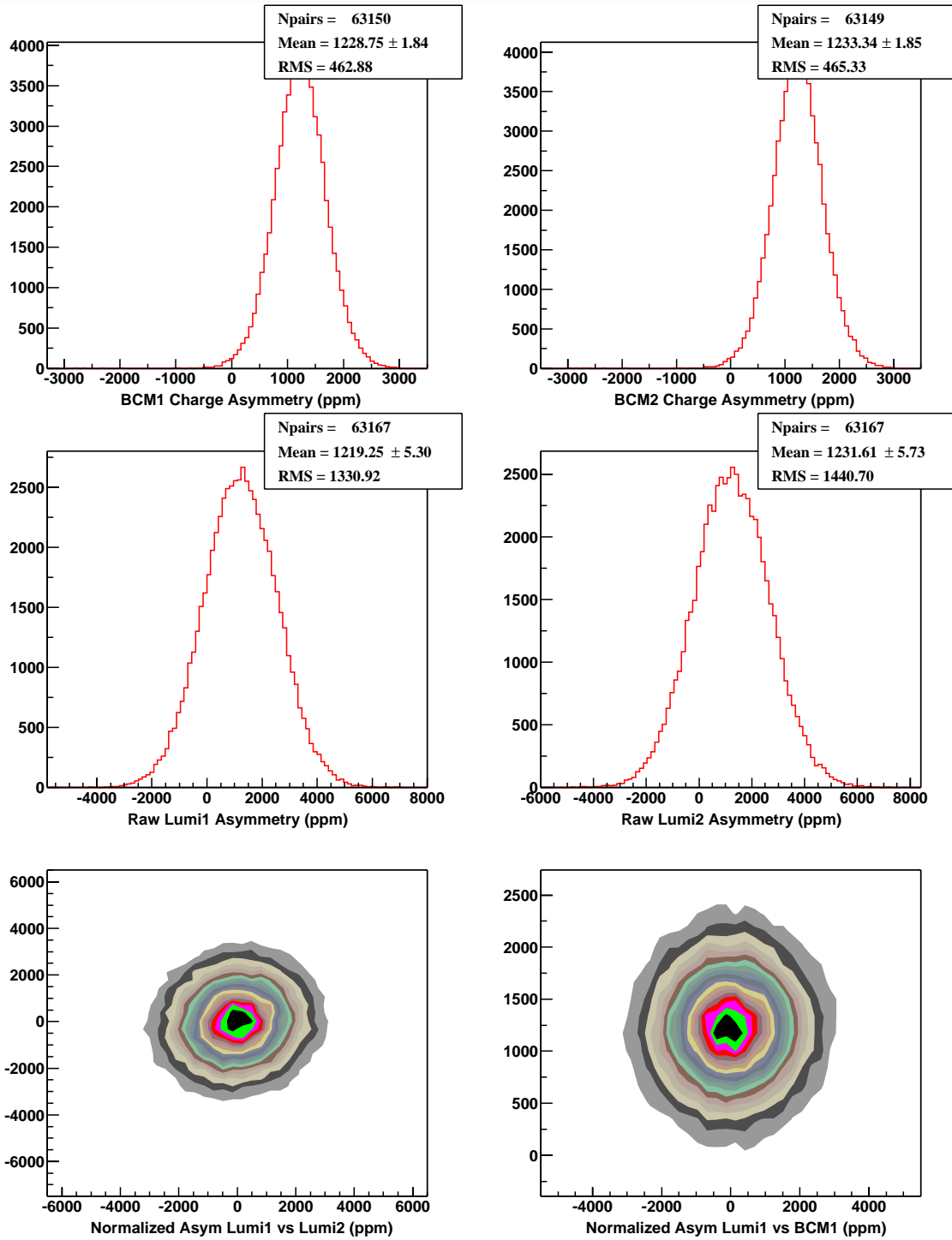
Figure 5: Typical Carbon target data. Window-pair asymmetry distributions for beam current (upper row), and for Lumi 1 and Lumi 2 (middle row) are shown. Normalizing the Lumi data to the BCM data on a pair-by-pair basis eliminates the effect of the non-zero beam current asymmetry (lower row), and one sees that the two Lumis provide statistically independent measurements.
