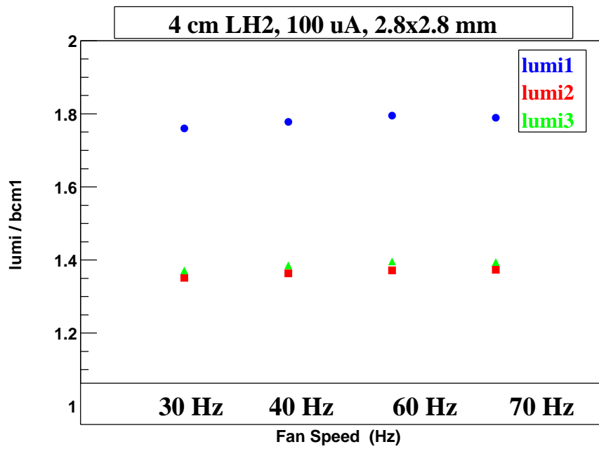
Figure 18: 4 cm LH 2 Lumi Bulk Effect vs. Fan Speed.
