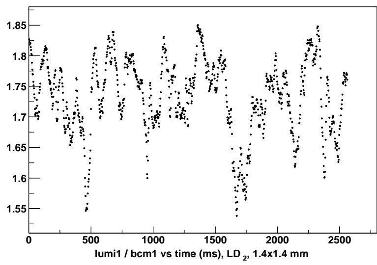
Figure 34: Lumi 1 signal, normalized by beam current, vs. time, for 100 \mu\text{A} , OS=13, carbon target (upper plot) and 15 cm LD_2 (lower plot). The characteristic fluctuation time scale for the LD_2 is clearly seen to be of order 100 ms.
