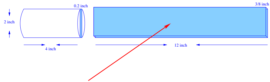
Figure 2: Lumi detector schematic.
