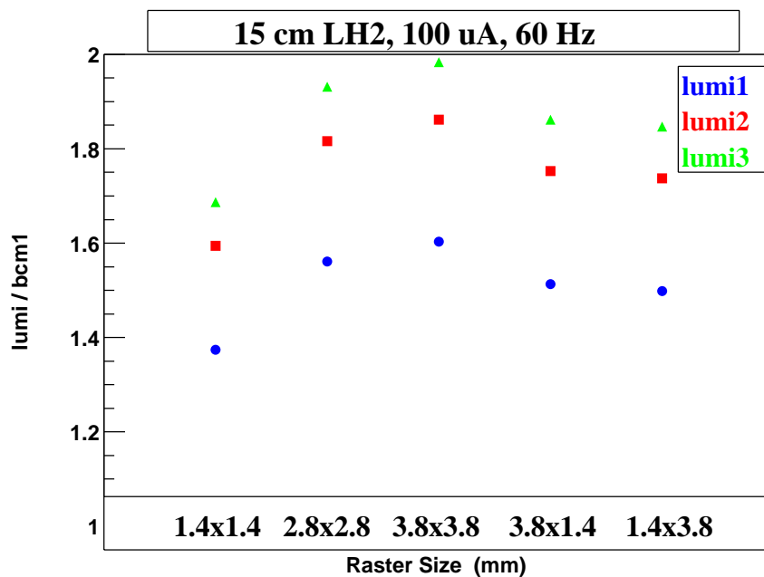
Figure 25: 15 cm LH_2 Lumi Bulk Effect vs. Raster Size.
