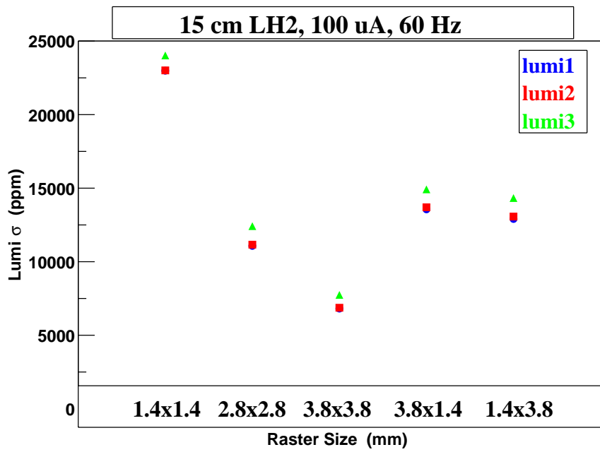
Figure 23: 15 cm LH_2 Lumi Sigma vs. Raster Size.
