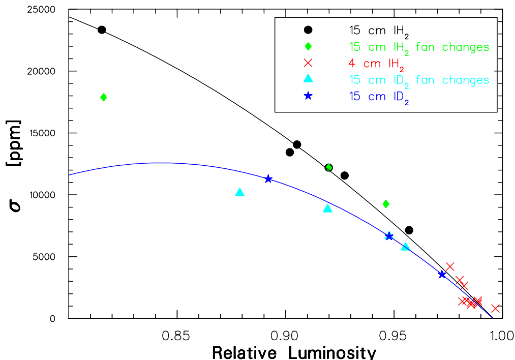
Figure 38: Fluctuation widths vs. Relative Luminosity, for various targets, raster and fan settings, and beam currents; all data with same high voltages and ADC gain setting, OS=3. The lines represent quadratic fits to the lH_2 (black) and lD_2 (blue) data respectively. For both Relative Luminosity and the \sigma 's, results are averages of the three 3 Lumi detectors.
