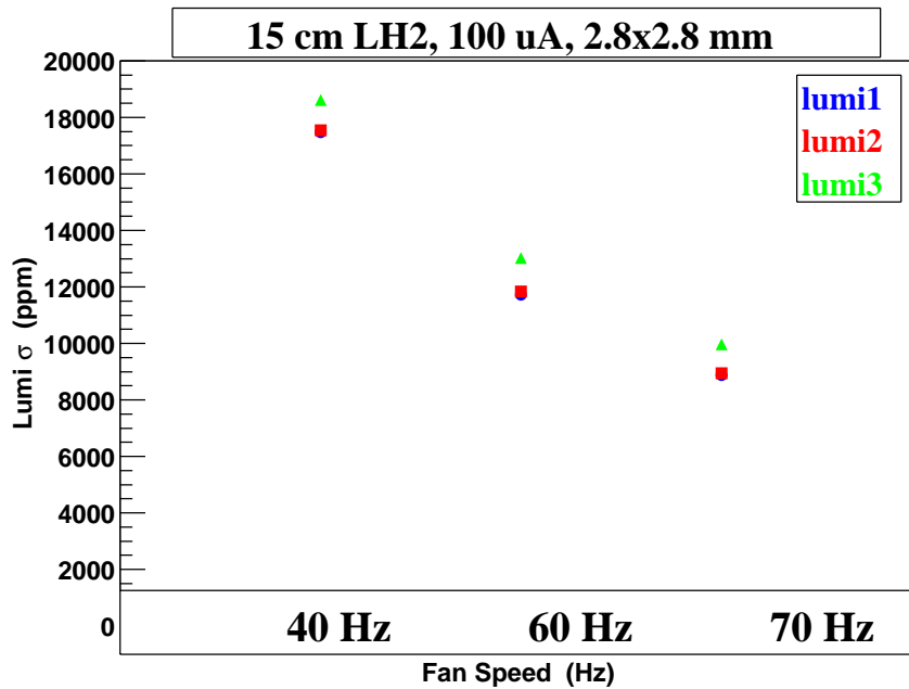
Figure 15: 15 cm lH_2 Lumi Sigma vs. Fan Speed.
