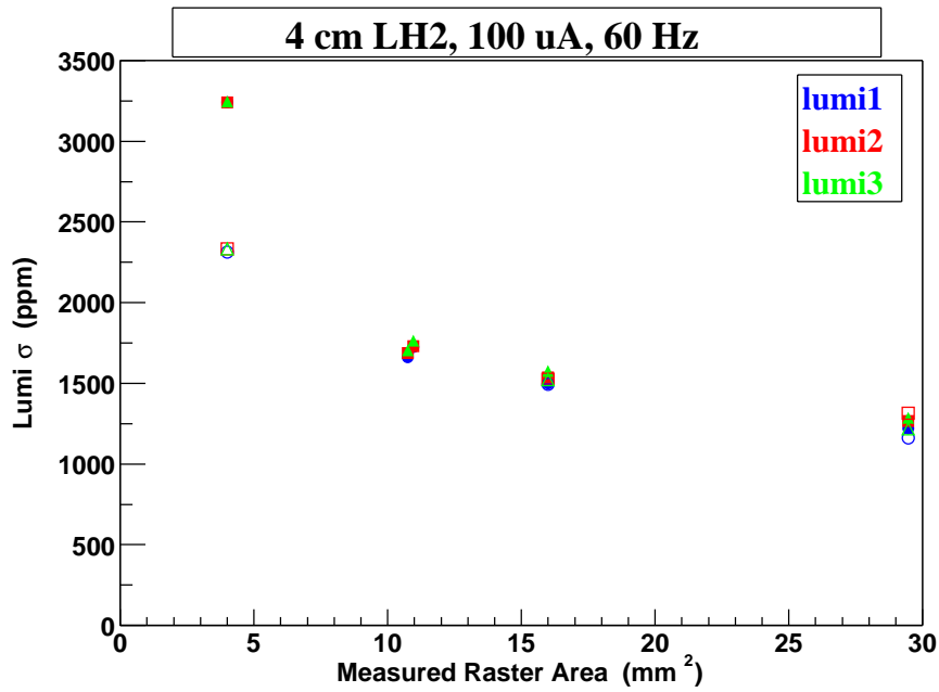
Figure 33: 4 cm IH_2 Lumi Sigma vs. Measured Raster Area, open markers larger spot size.
