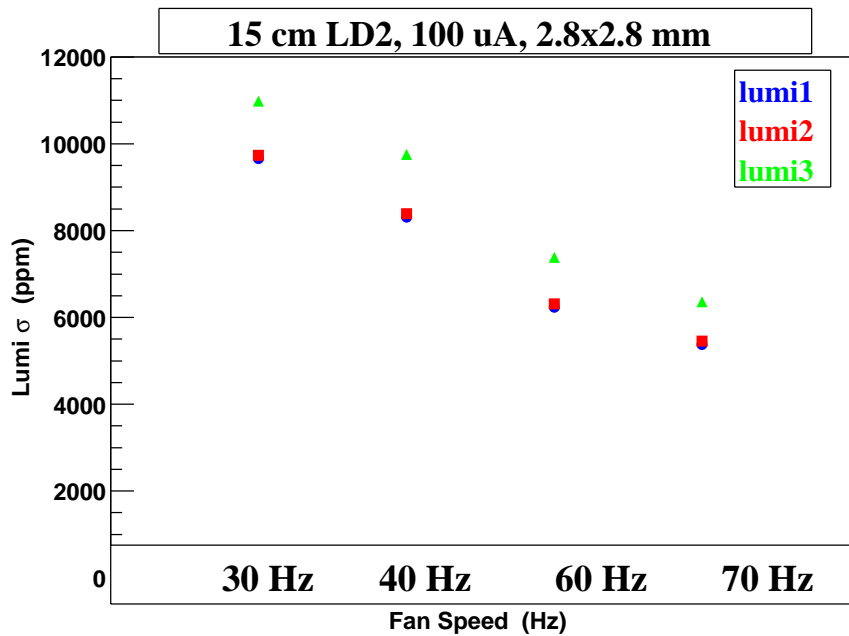
Figure 19: 15 cm LD 2 Lumi Sigma vs. Fan Speed.
