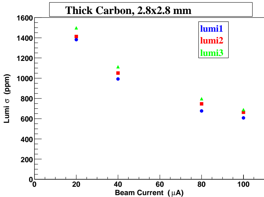
Figure 13: Carbon target (OS=3) Lumi Sigma vs. Beam Current.
