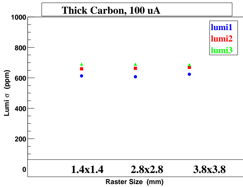
Figure 21: Carbon target Lumi Sigma vs. Raster Size.
