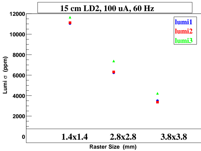
Figure 29: 15 cm LD_2 Lumi Sigma vs. Raster Size.
