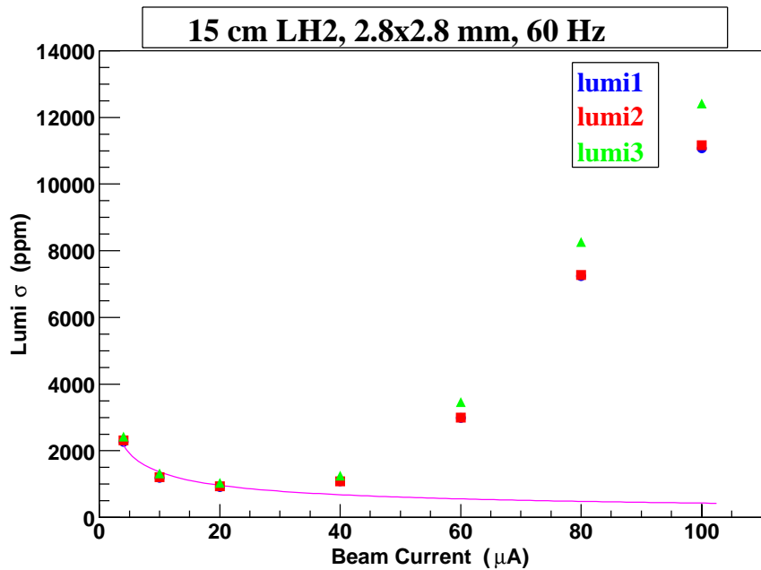
Figure 10: 15 cm LH_2 (OS=3) Lumi Sigma vs. Beam Current. Counting statistics dependence shown by line.
