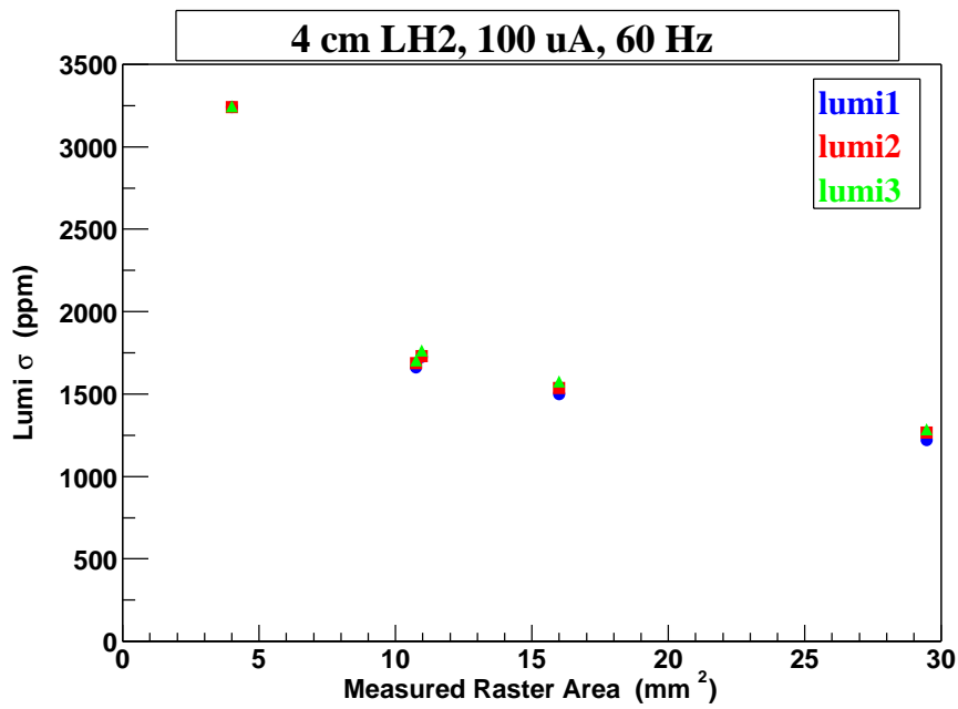
Figure 27: 4 cm LH_2 Lumi Sigma vs. Measured Raster Area.
