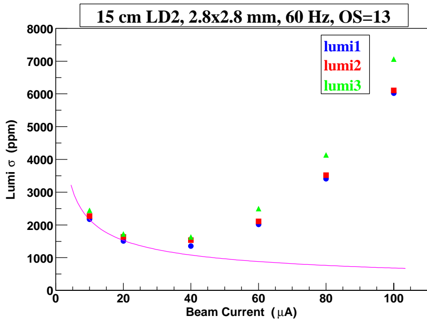
Figure 7: 15 cm LD_2 (OS=13) Lumi Sigma vs. Beam Current. Counting statistics dependence shown by line.
