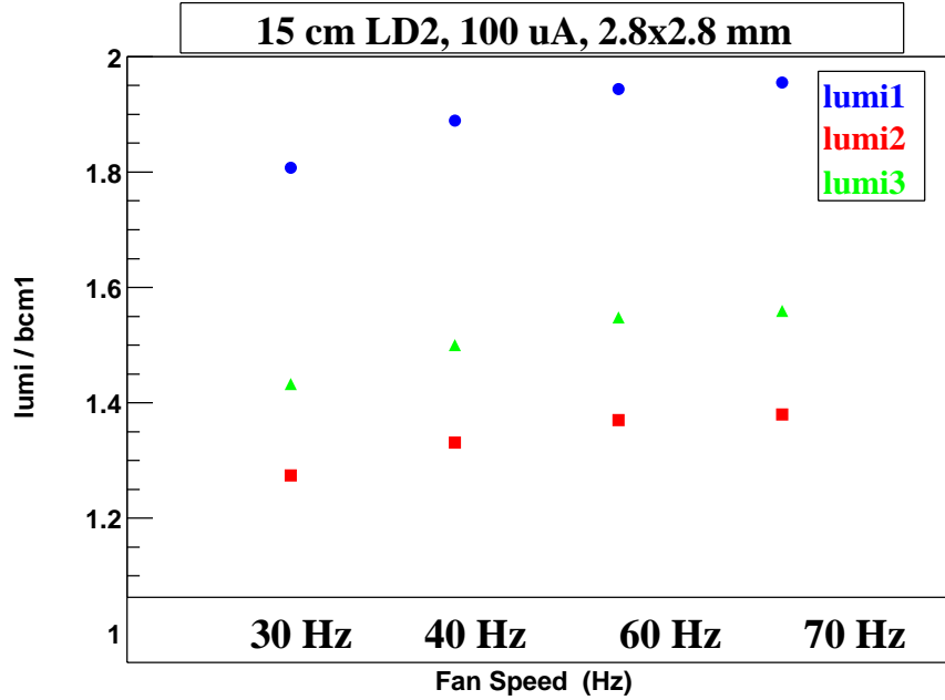
Figure 20: 15 cm lD_2 Lumi Bulk Effect vs. Fan Speed.
