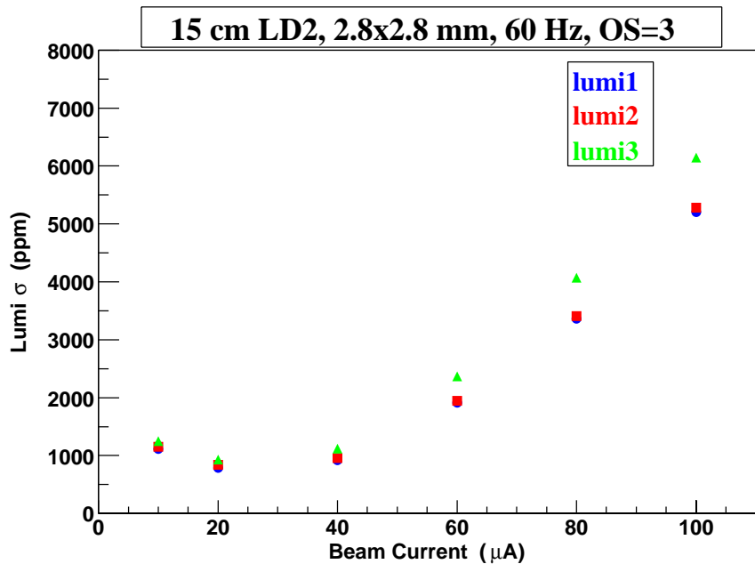
Figure 8: 15 cm LD_2 (OS=3) Lumi Sigma vs. Beam Current.
