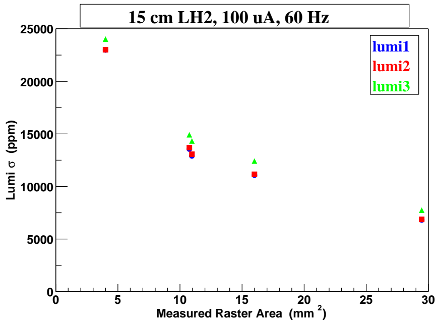
Figure 24: 15 cm LH_2 Lumi Sigma vs. measured Raster Area.
