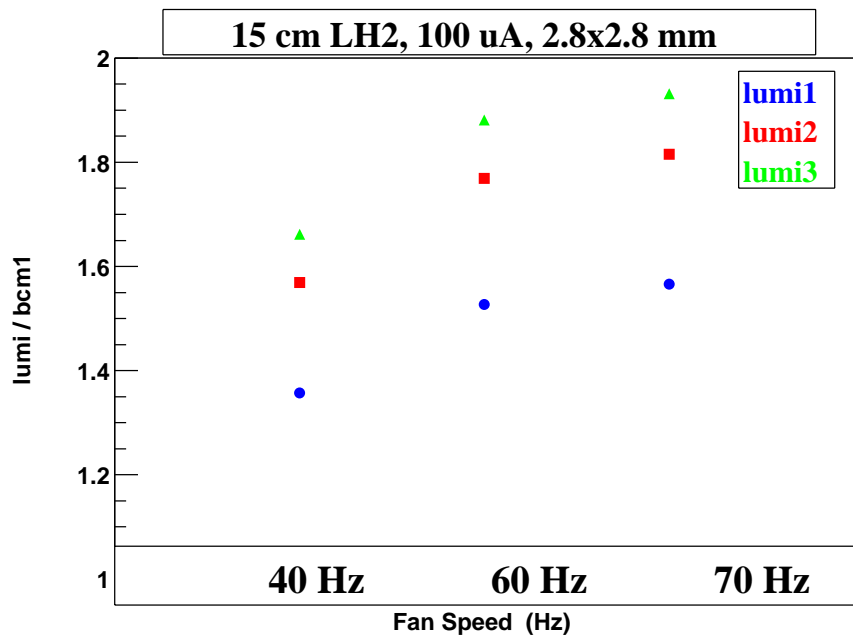
Figure 16: 15 cm LH_2 Lumi Bulk Effect vs. Fan Speed.
