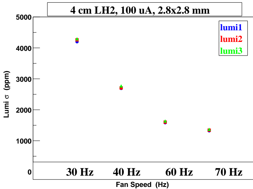
Figure 17: 4 cm LH_2 Lumi Sigma vs. Fan Speed.
