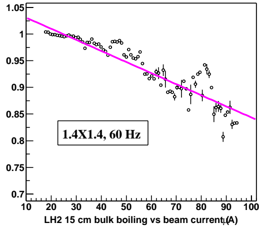
Figure 14: Bulk effect: relative ADC peak values (Lumi 1, normalized to beam current) vs. Beam Current for various configurations. Simple linear fits are shown, normalized to 1 at 20 \mu A. Data shown are for Lumi 1. The raster settings and fan speeds are indicated.
