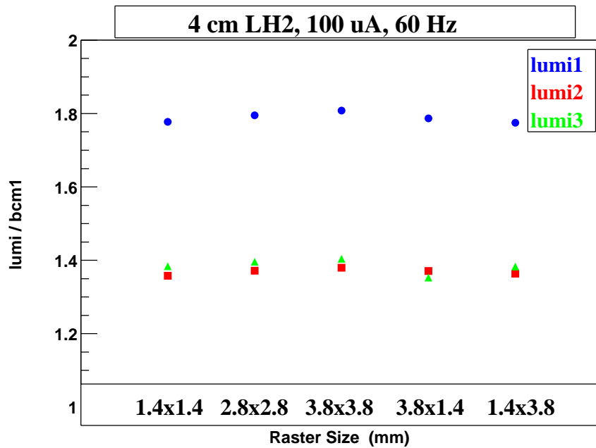
Figure 28: 4 cm LH_2 Lumi Bulk Effect vs. Raster Size.
