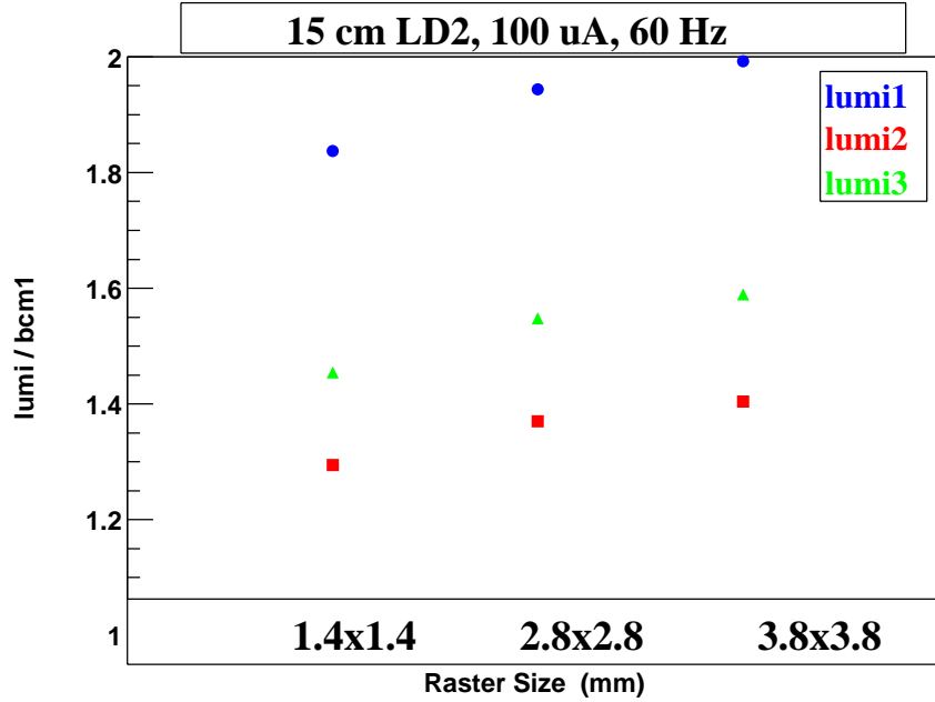
Figure 31: 15 cm LD_2 Lumi Bulk Effect vs. Raster Size.
