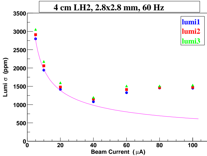
Figure 11: 4 cm LH_2 (OS=3) Lumi Sigma vs. Beam Current. Counting statistics dependence shown by line.
