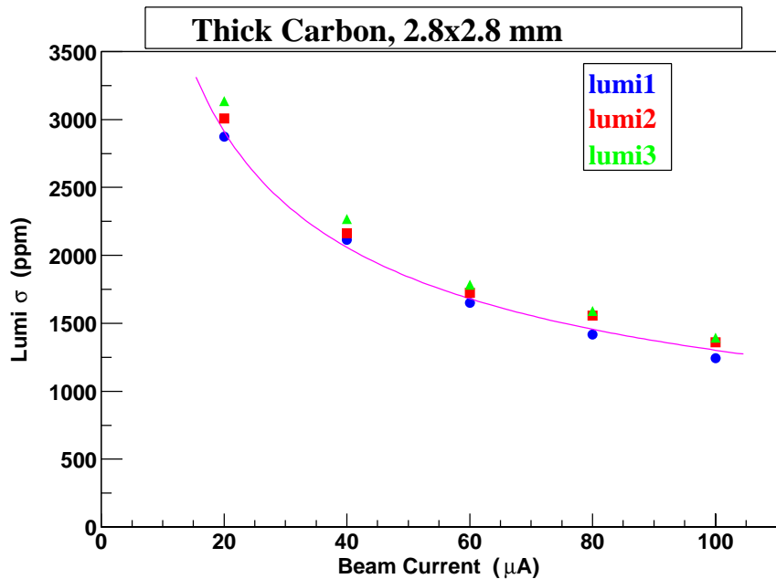
Figure 12: Carbon target (OS=13) Lumi Sigma vs. Beam Current. Counting statistics dependence shown by line.
