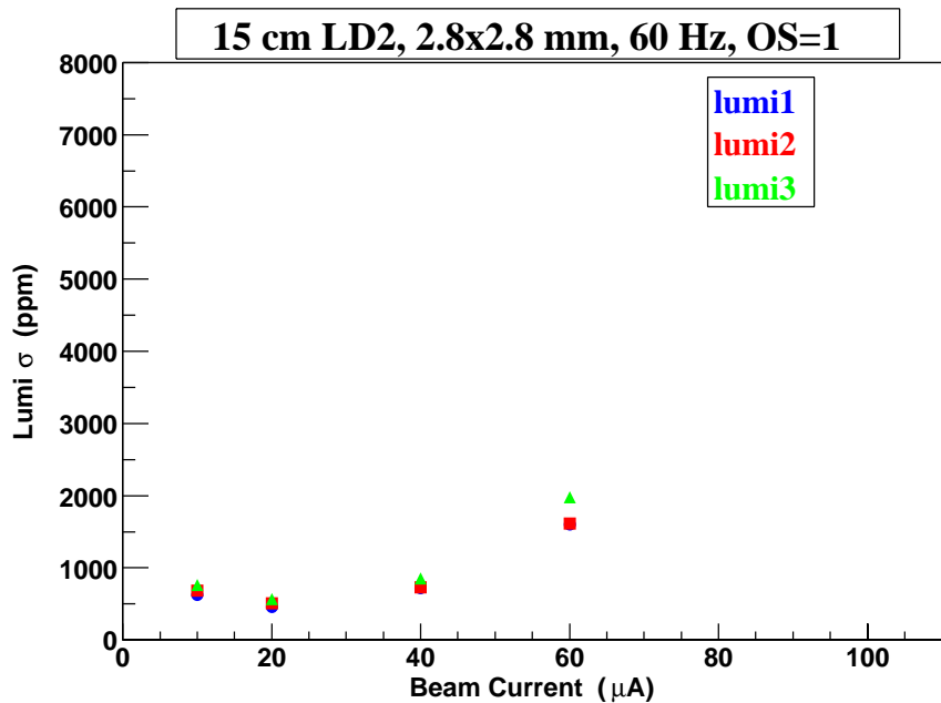
Figure 9: 15 cm LD_2 (OS=1) Lumi Sigma vs. Beam Current.
