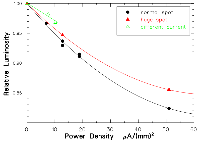
Figure 39: Relative Luminosity vs. Beam Power Density, for the 15 cm lH_2 cell, 60 Hz fan speed, OS=3. The black circles are data taken at 100 \mu\text{A} , for various raster settings, with the normal beam spot, the red closed triangles are similar data taken with the 'huge' intrinsic beam spot, and the green open triangles are data taken with the normal spot, but at lower beam currents. The fits are simple quadratic or linear fits, forced to go through relative Luminosity = 1 at zero power density.
