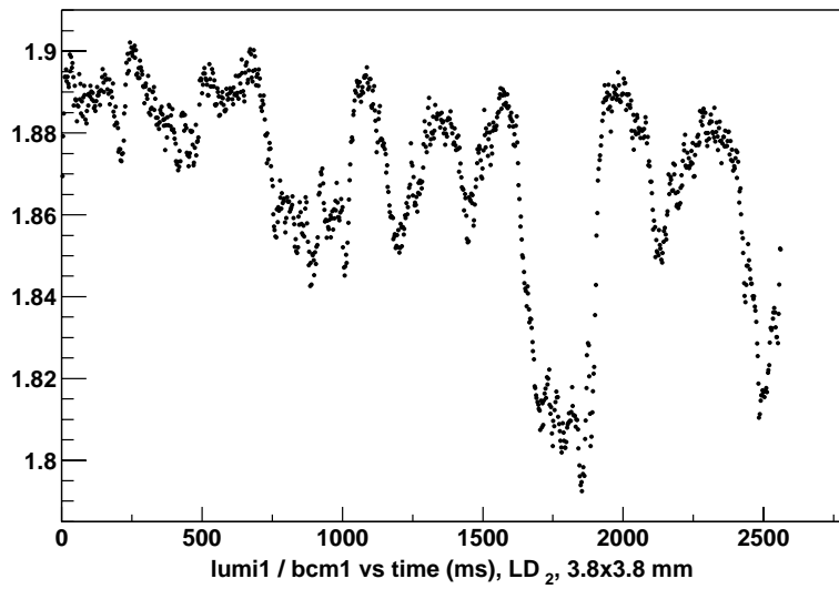
Figure 36: Lumi 1 signal , normalized by beam current, vs. time, for 15 cm ID_2 , OS=13, at 100 \mu A, with 2.8 mm \times 2.8 mm raster (upper plot) and 3.8 mm \times 3.8 mm raster (lower plot).
