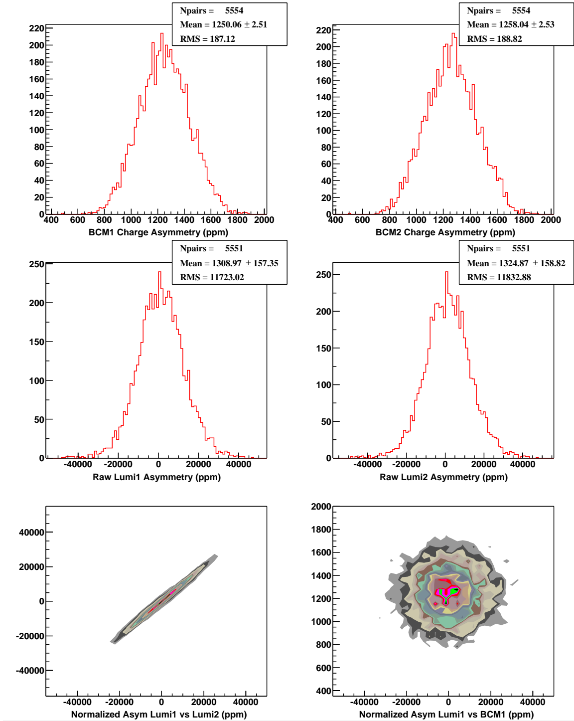
Figure 6: Typical IH_2 target data (15 cm cell). Window-pair asymmetry distributions for beam current (upper row), and for Lumi 1 and Lumi 2 (middle row) are shown. Here the data from the two Lumi detectors (after normalizing by beam current) are not statistically independent, due to target density fluctuations (lower left plot).
