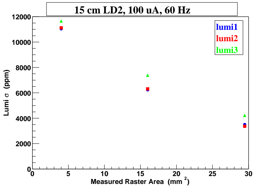
Figure 30: 15 cm LD_2 Lumi Sigma vs. Measured Raster Area.
