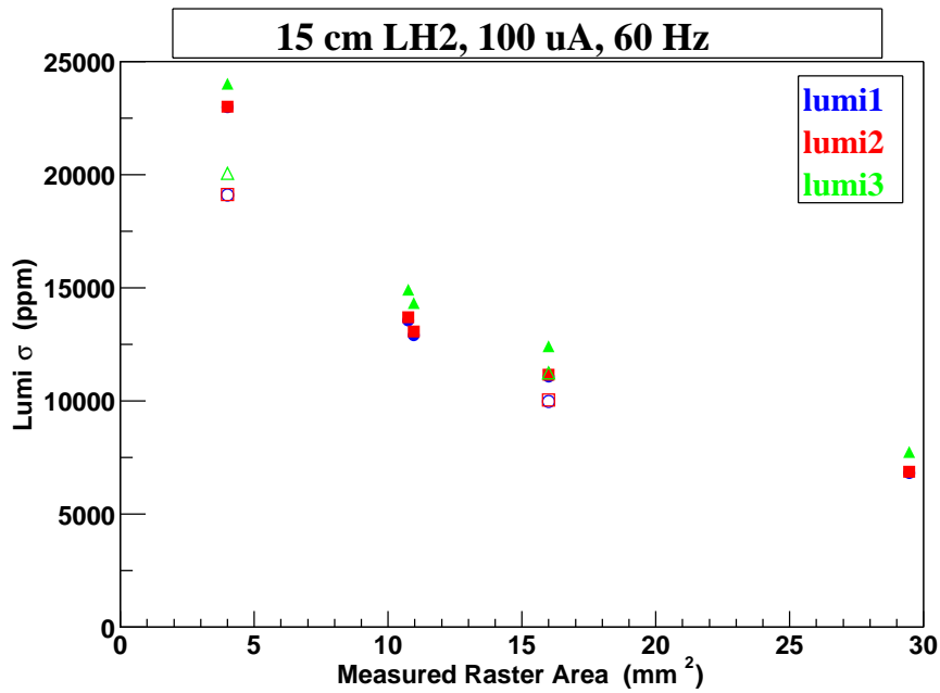
Figure 32: 15 cm IH_2 Lumi Sigma vs. Measured Raster Area, open markers larger spot size.
