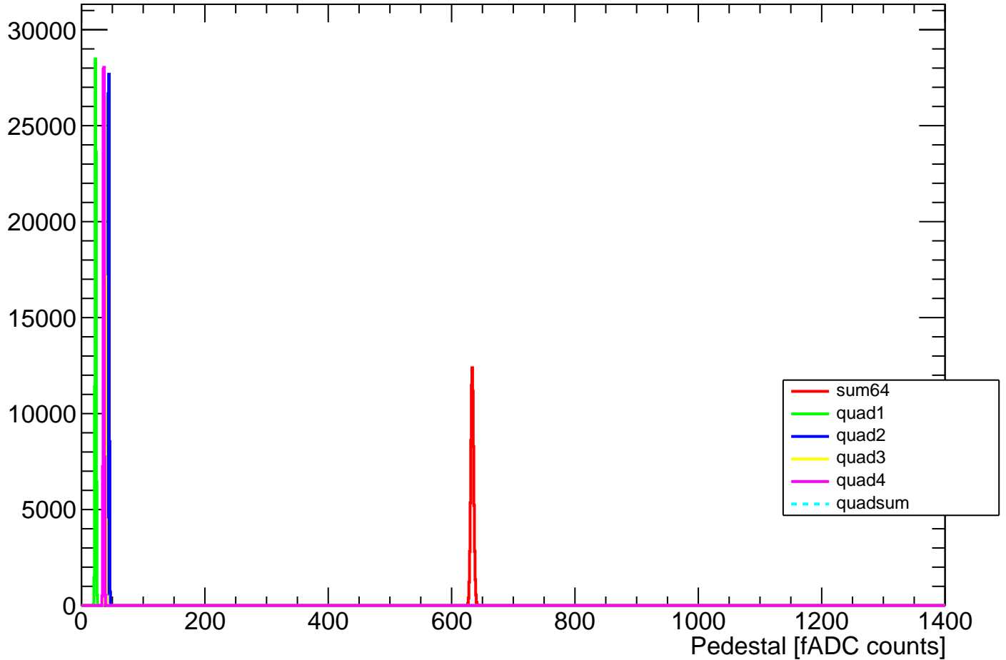
Pedestal Distribution (average fADC count between 0 - 24 ns)
