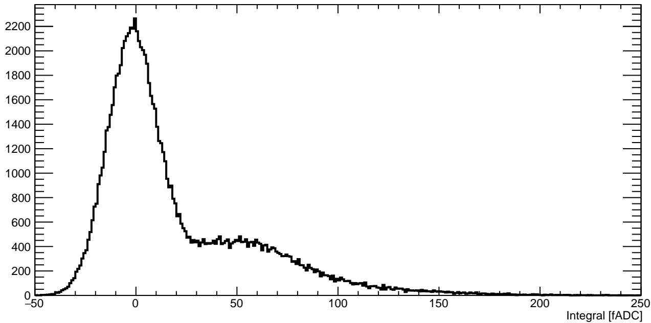
fADC Integral Distribution (with pedestal subtraction)
