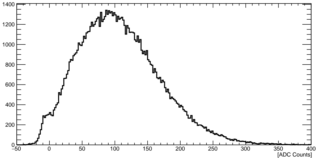
Sum of 8 Maroc Channels (adcPedSub)
