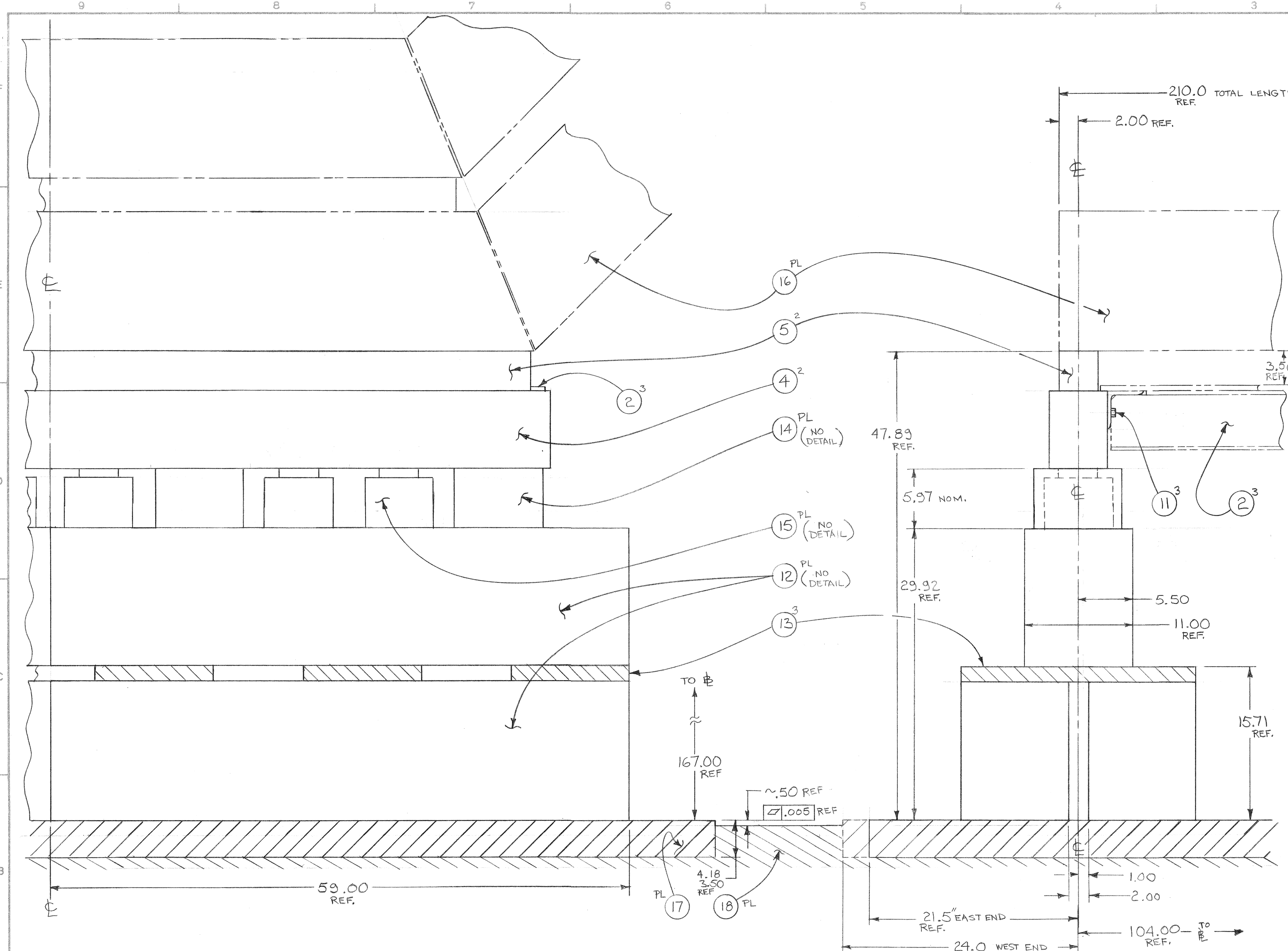
① CLEO II - MAGNET YOKE SUPPORT - ASSEMBLY SCALE: 1:15 NOTE: ONE END ONLY SHOWN HERE
