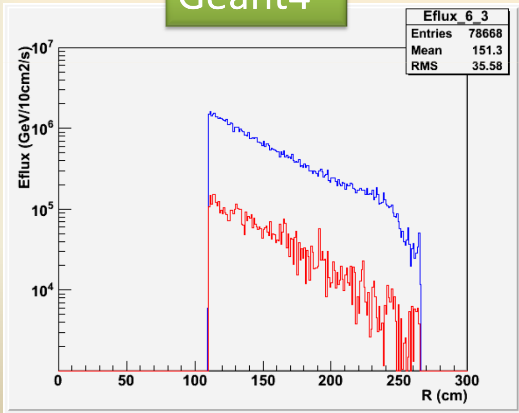
Geant4
