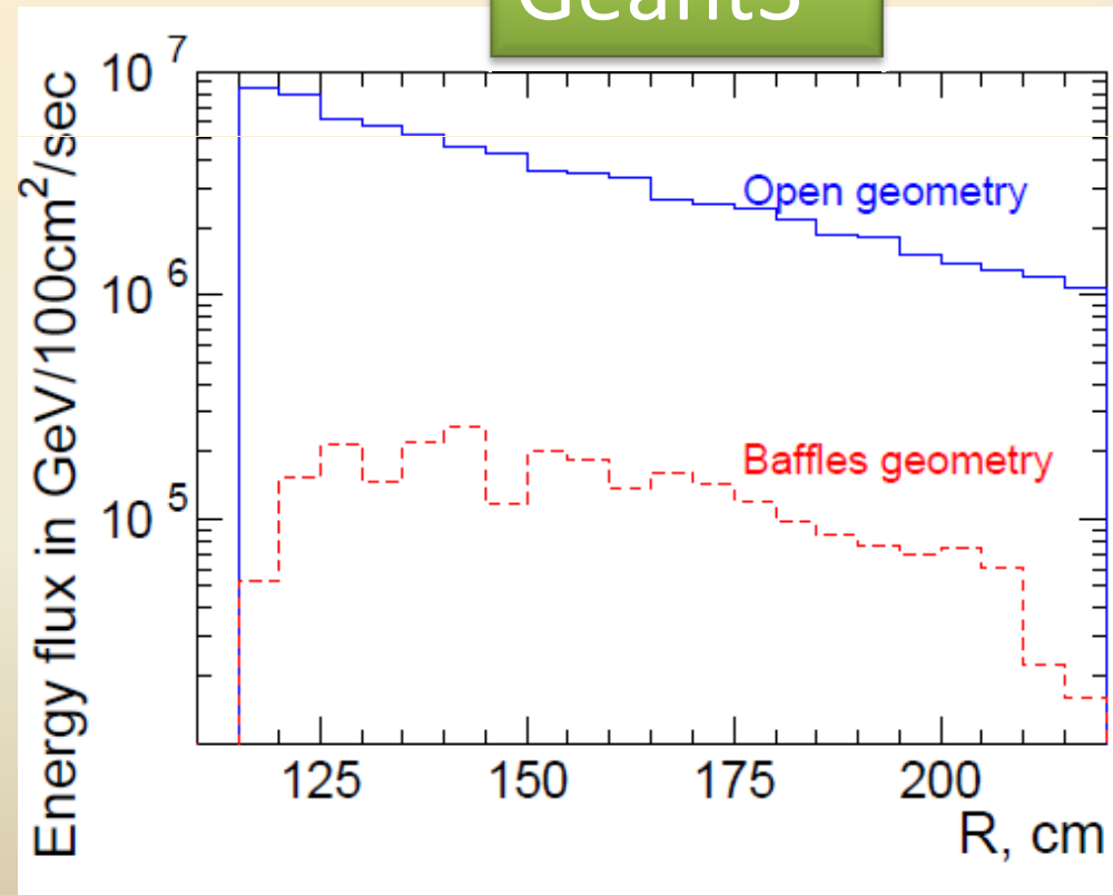
Geant3
