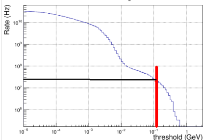
HCal energy deposited rate Vs Threshold, G_M^1, Q^2 = 13.5 \text{ GeV}^2, I = 44 \mu\text{A}
