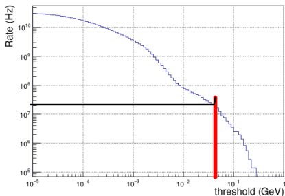
HCal energy deposited rate Vs threshold, Q^2 = 3.5 \text{ GeV}^2, I = 44 \mu\text{A}
