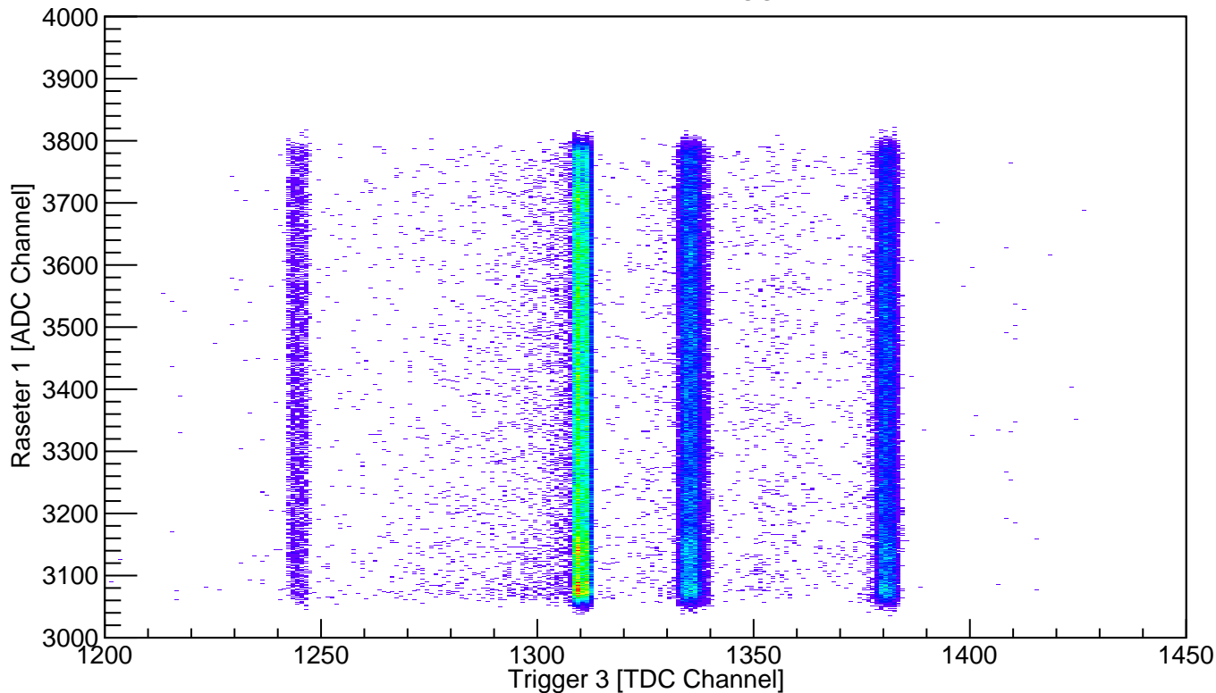
Raster 1 Current vs. Trigger 3 Time
