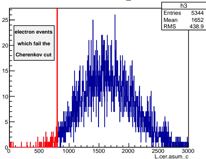
Cherenkov of cut_e
