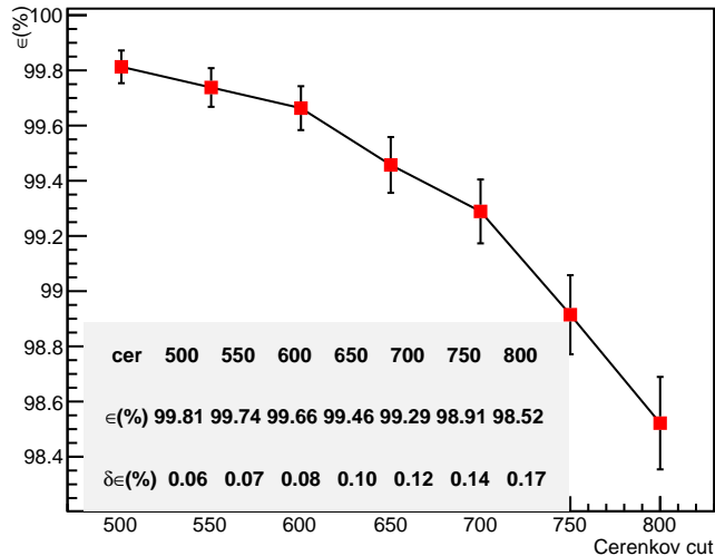
Cherenkov cut efficiency
