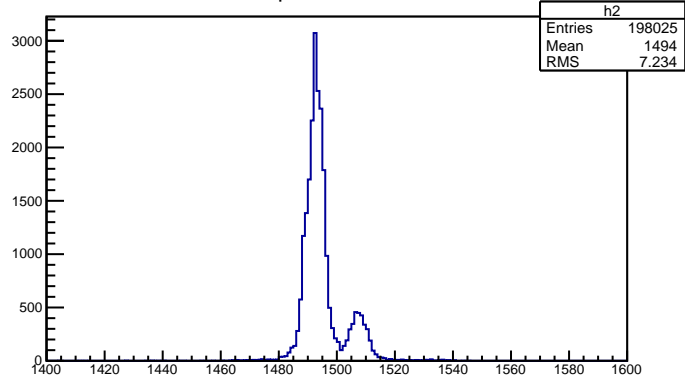
Raw TDC spectrum of S2mR7 on LHRS
