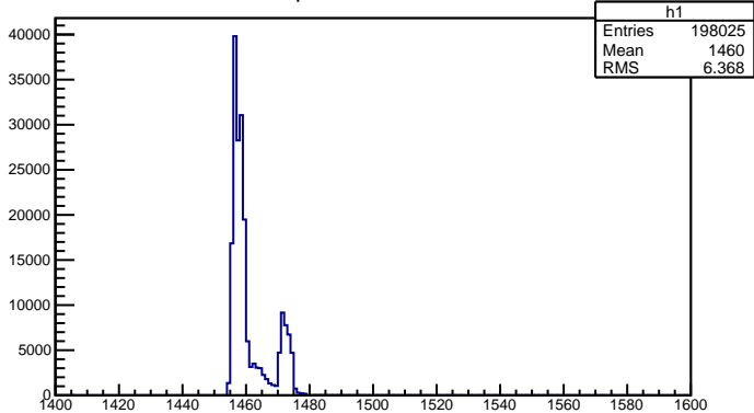
Raw TDC spectrum of S0A on LHRS
