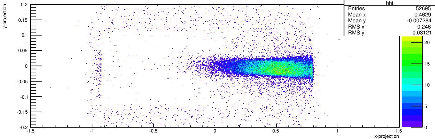
s0 Track Projection:Inefficient Events(No TDC Hit on s0-B)
