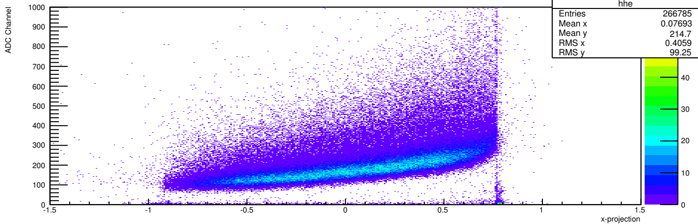
s0-A Amplitude vs. x-Projection
