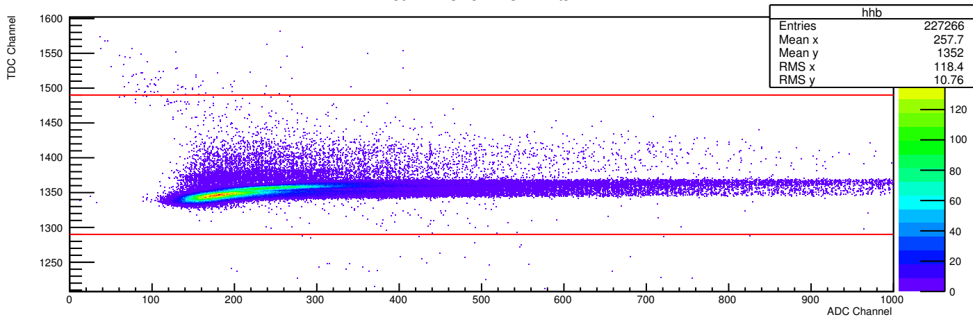
s0-B TDC vs. ADC:All Hits
