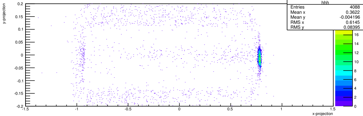
s0 Track Projection:Inefficient Events(No TDC Hit on s0-A)
