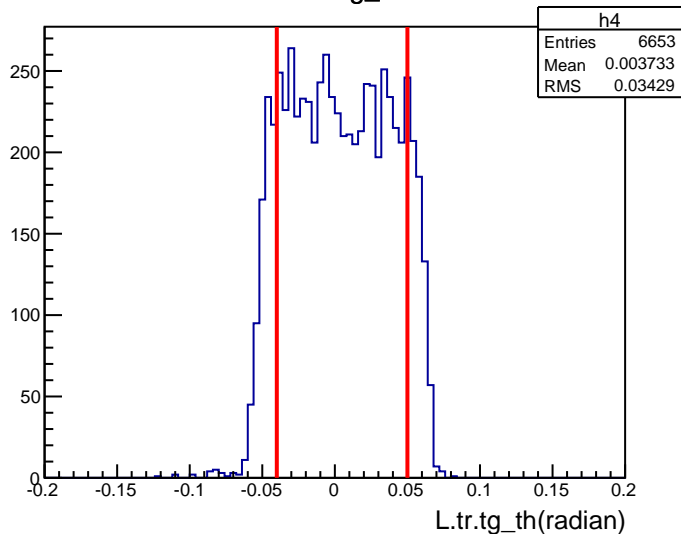
cut4: -0.04 < tg\_th < 0.05
