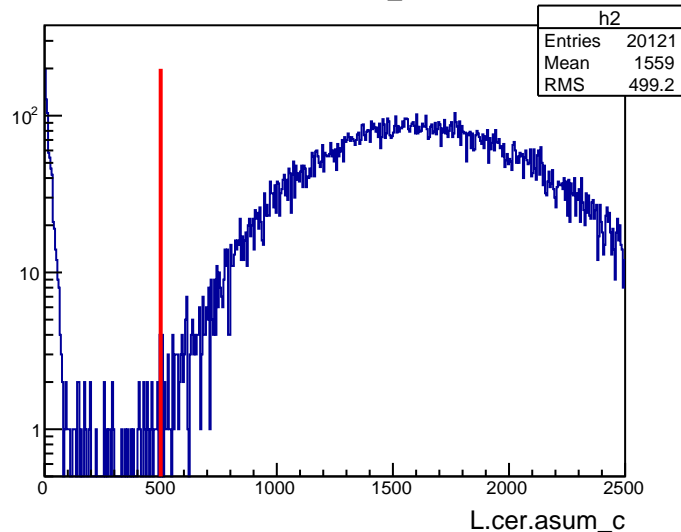
cut4: -0.04 < tg\_th < 0.05
