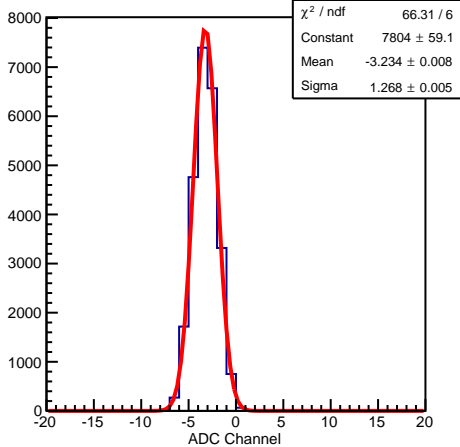
S2m-4L Pedestal: 0 Hz
