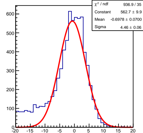
S2m-4L Pedestal: ~280,000 Hz
