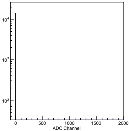
S2m-4L Pedestal: ~13,600 Hz
