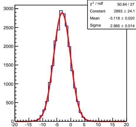
S2m-4L Pedestal: ~1470 Hz
