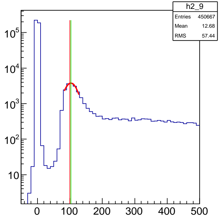
ADC 10 main peak
