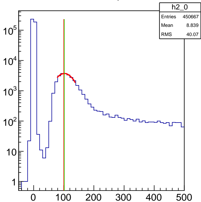
ADC 1 main peak
