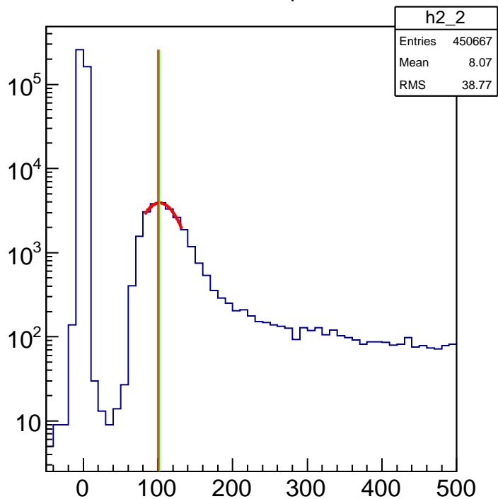
ADC 3 main peak
