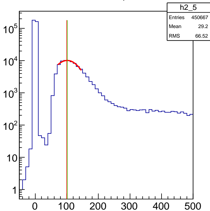
ADC 6 main peak
