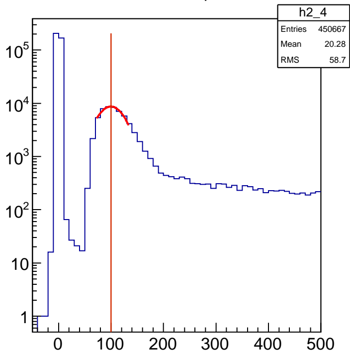
ADC 5 main peak
