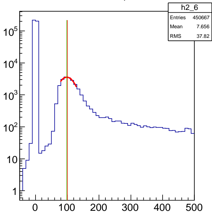
ADC 7 main peak
