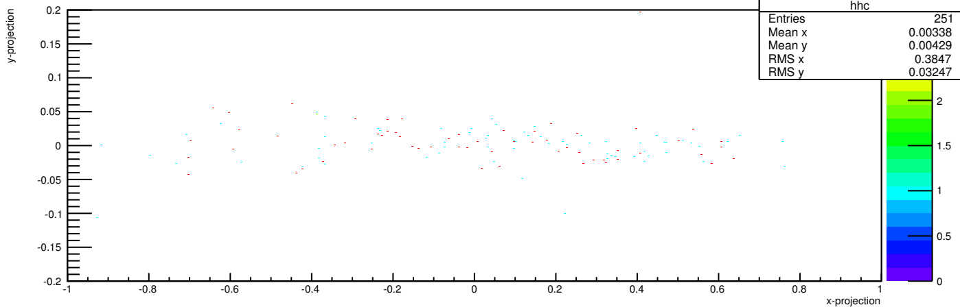
Gas Cherenkov Track Projection: Inefficient Electron Events (No TDC Hit on Hardware Sum)
