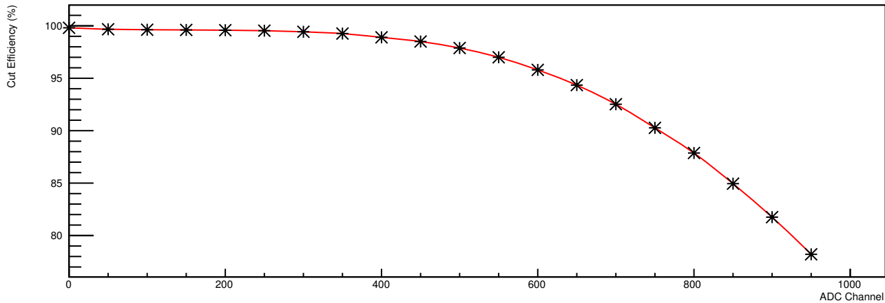
GC Electron Detection Efficiency
