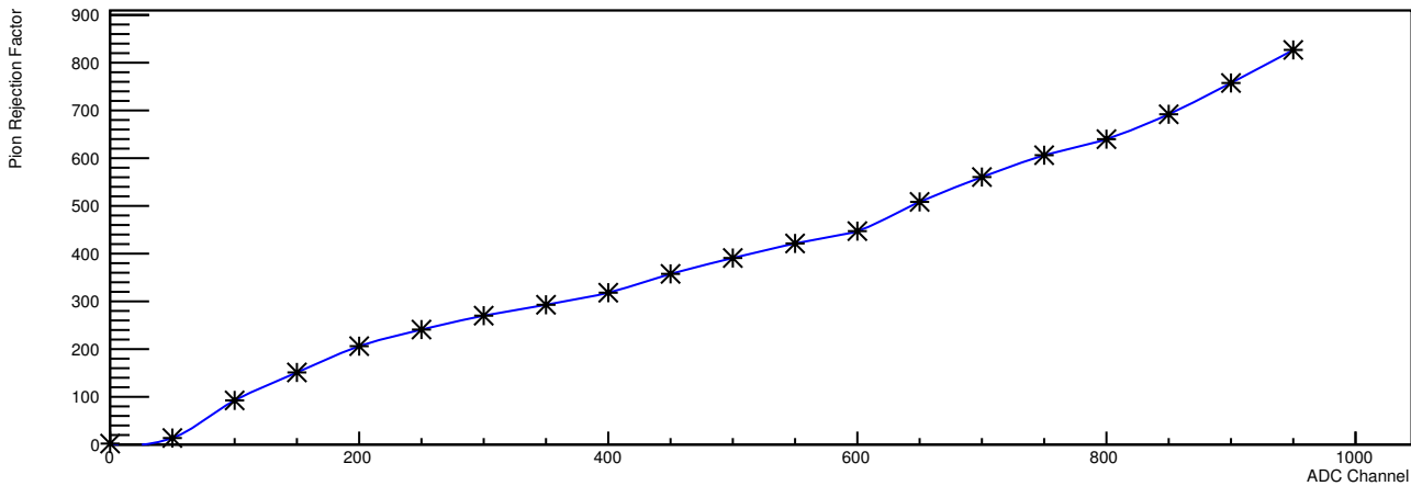
GC Pion Rejection Efficiency
