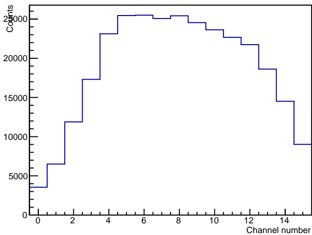
Rs2lt0-15_counts
