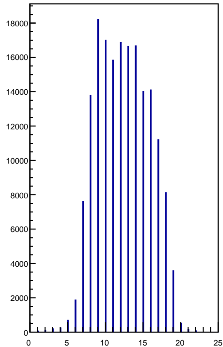
Number of hits Per WG on U3
