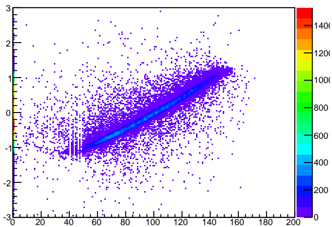
Track X vs Straw Number on U3
