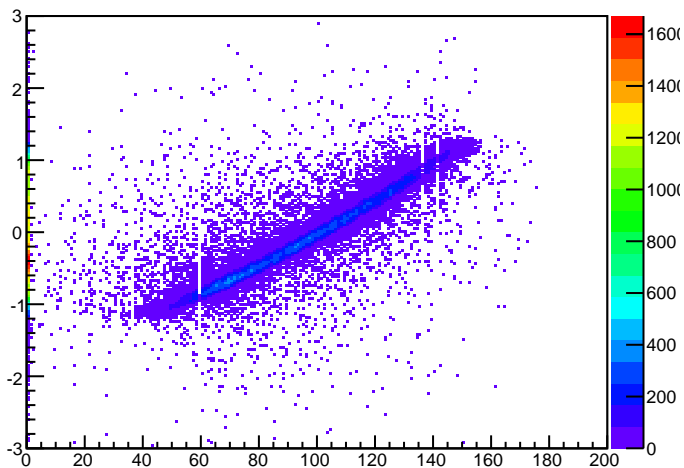
Track X vs Straw Number on U1
