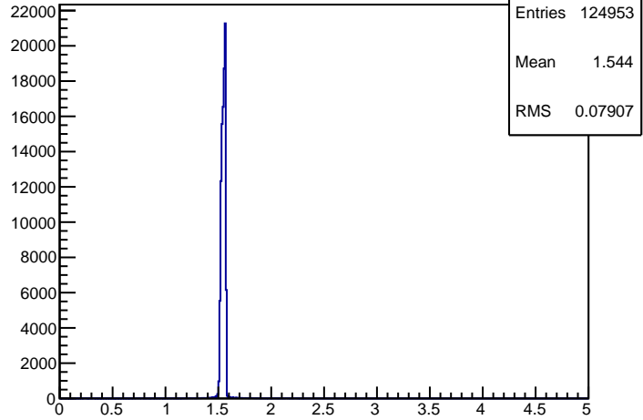
R-arm nu, energy transfer
