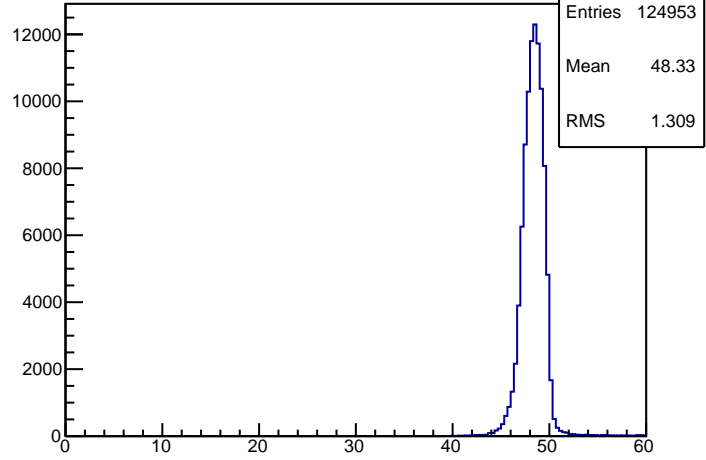
R-arm Electron Angle of scattering (deg)
