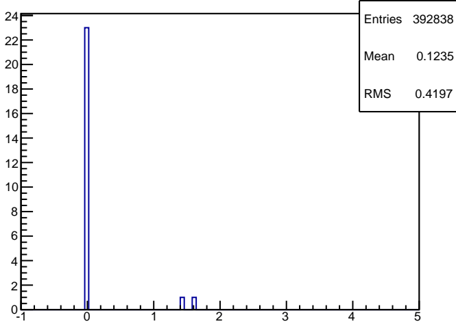
R-arm W, Invariant mass
