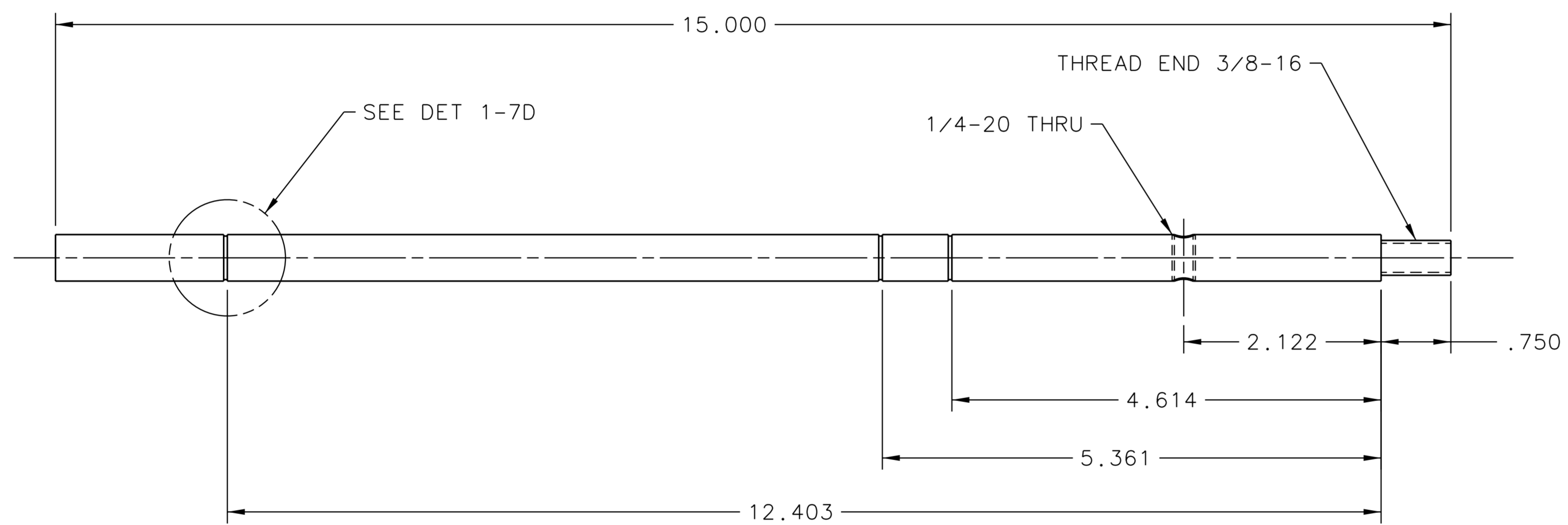
FRONT VIEW 1-6B
