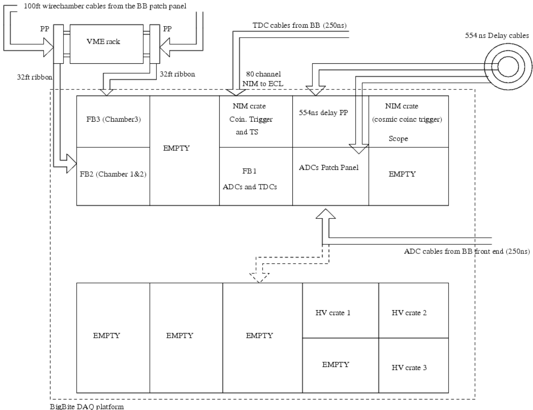
BigBite DAQ platform
