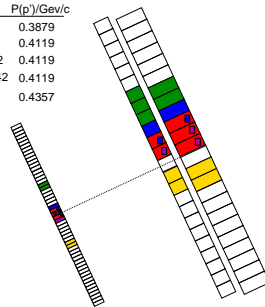
Figure 4: Diagram showing the three scintillator planes in the proton detector and the pattern of hits in the bars for events selected by cutting on the sieve hole pattern shown in Fig.5; note the color coding to illustrate which bars are illuminated by protons being scattered by electrons going through the each sieve hole. This gives an angle and momentum correspondence for determining a transport matrix for the proton detector.
