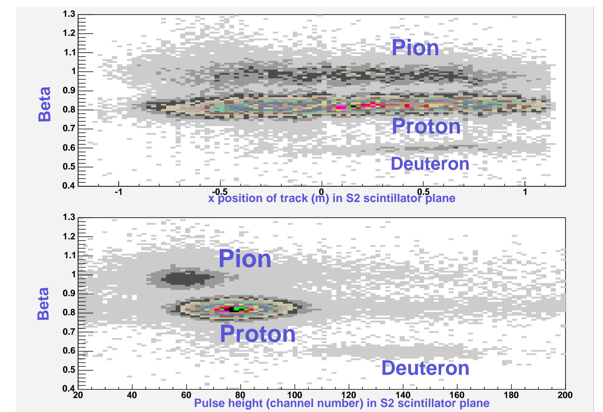
\beta versus x position of tracks (top) and beta versus pulse height (bottom) in the S2 scintillator plane of the right HRS
