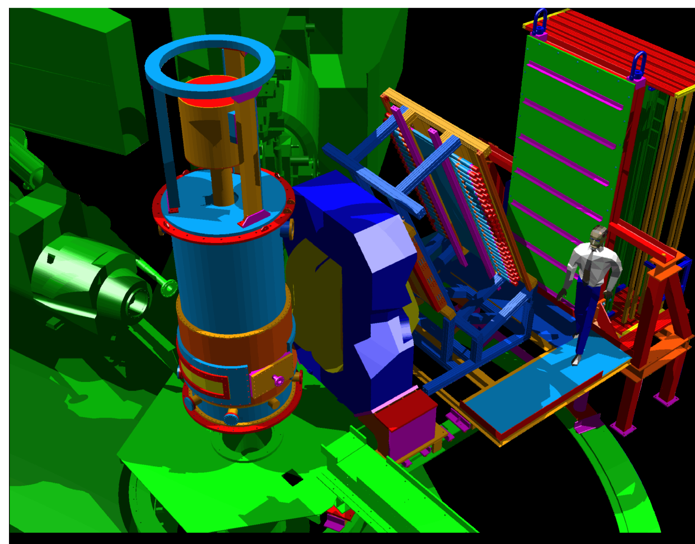
Short Range Correlations Experiment layout
