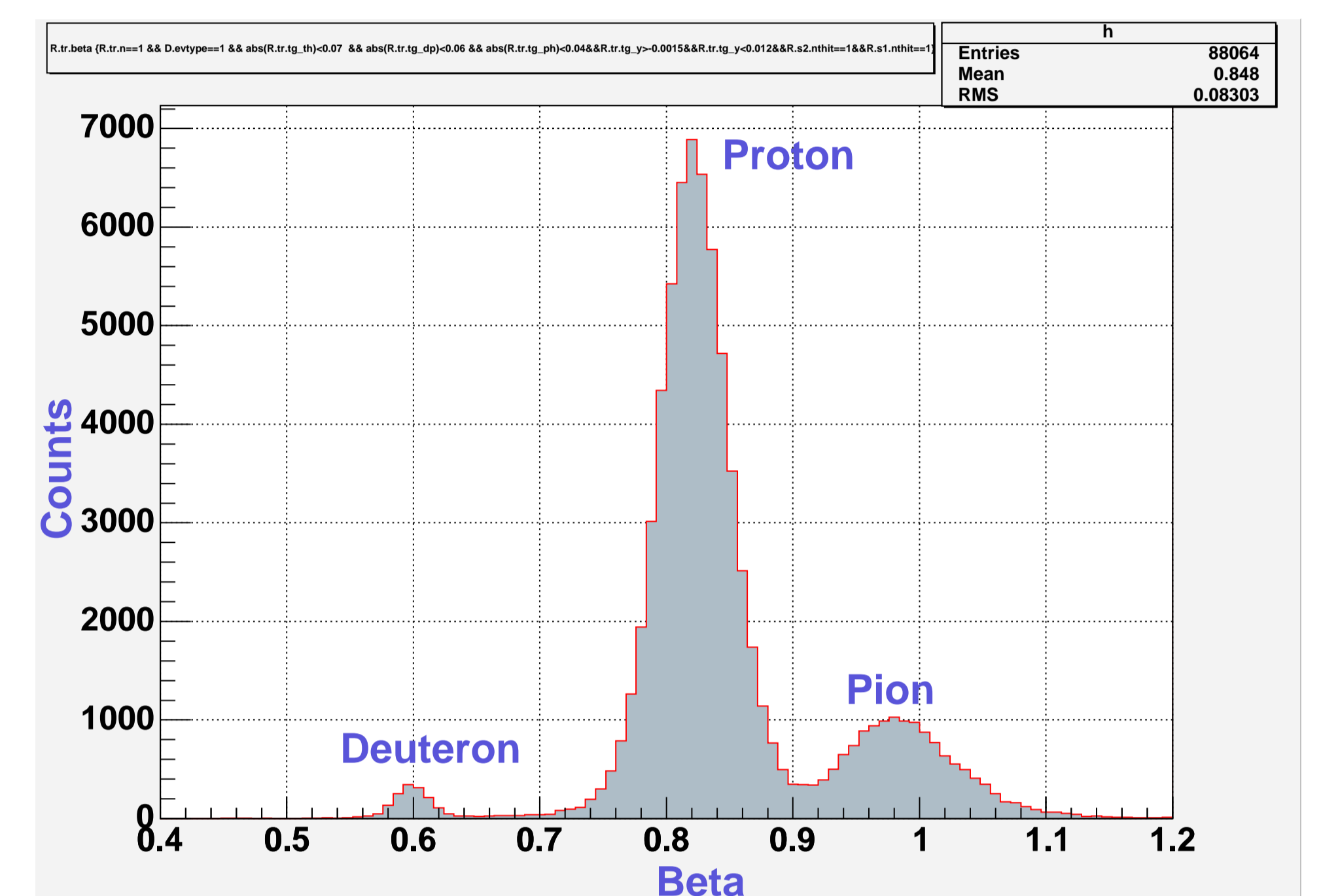
\beta for different particle species detected by the right HRS
