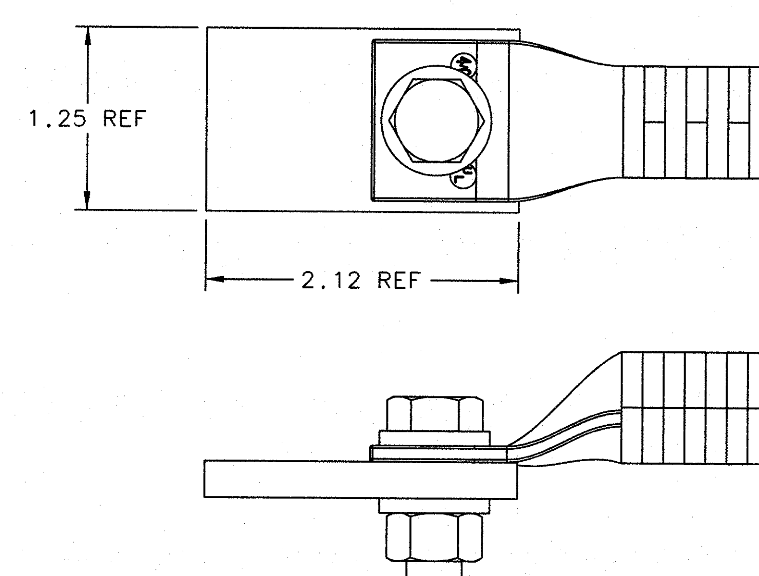
DETAIL VIEW 4-2A - 4 REQD SCALE 1-1/2:1 (TYP CONN FOR CLG WATER ON LEADS)
