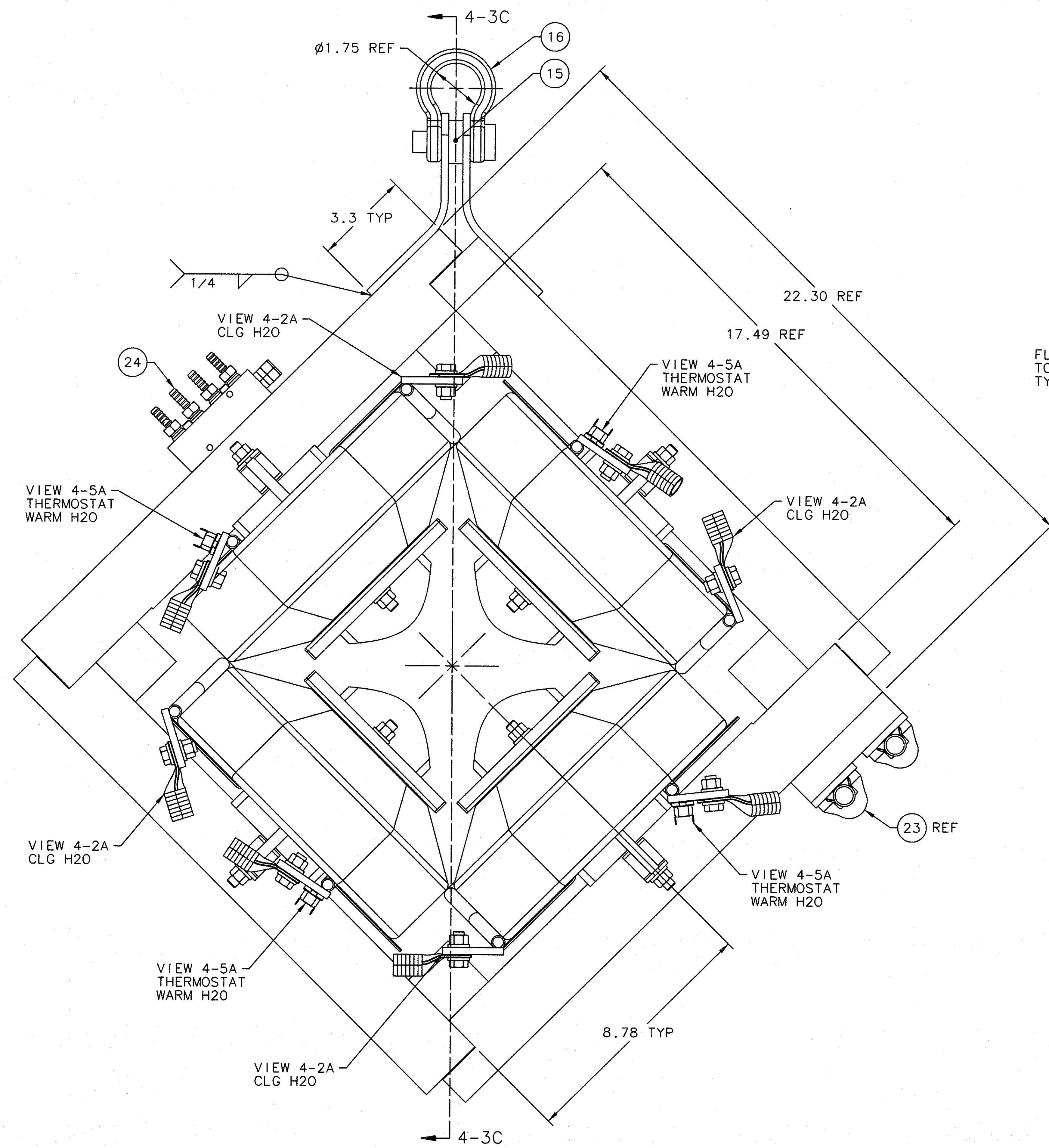
FRONT VIEW 4-7C (WATER HOSES & POWER CABLES NOT SHOWN FOR CLARITY)
