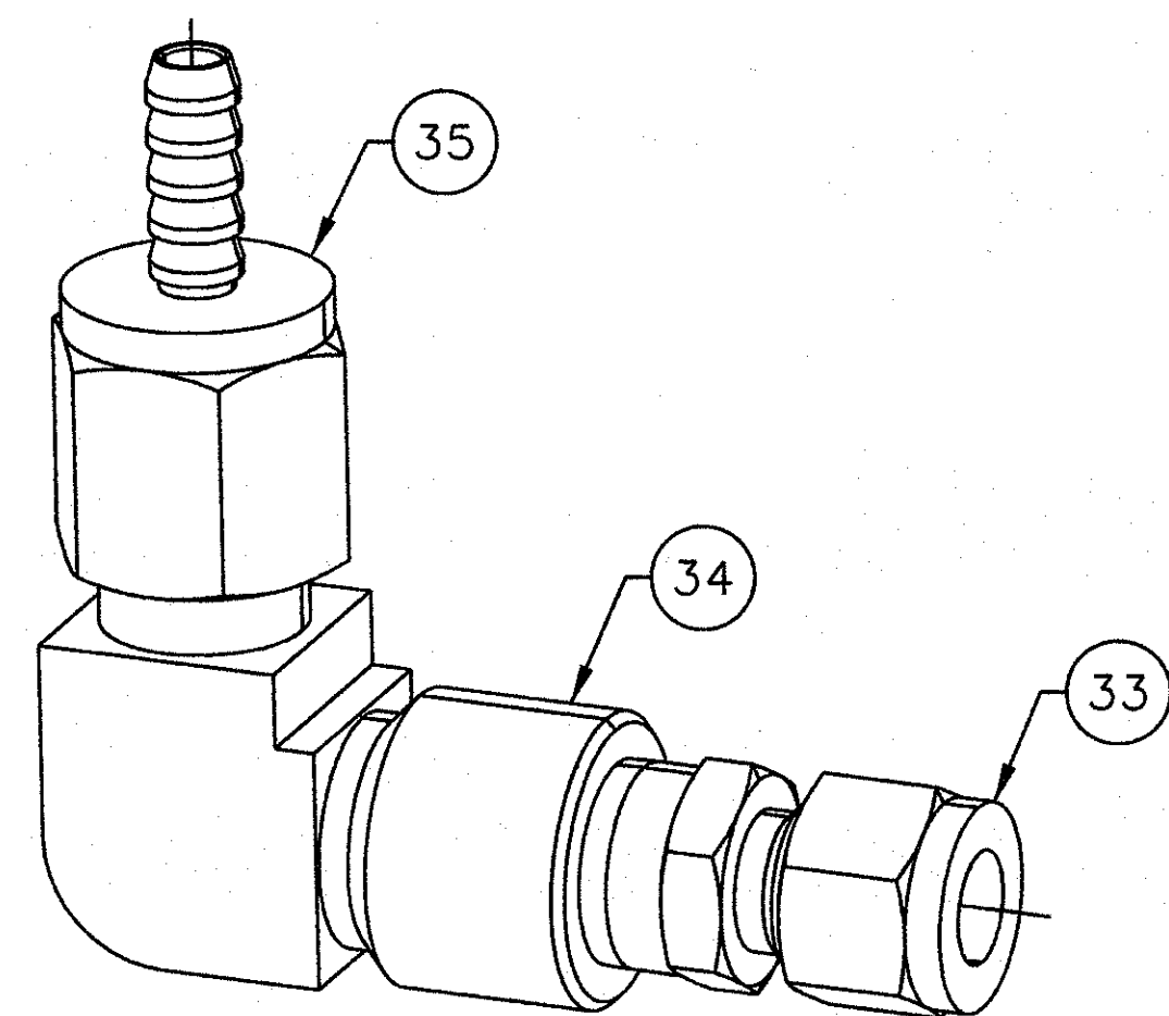
DETAIL VIEW 4-8A - 8 REQD SCALE 1-1/2:1 (TYP CONN FOR COOLING ON LEADS)
