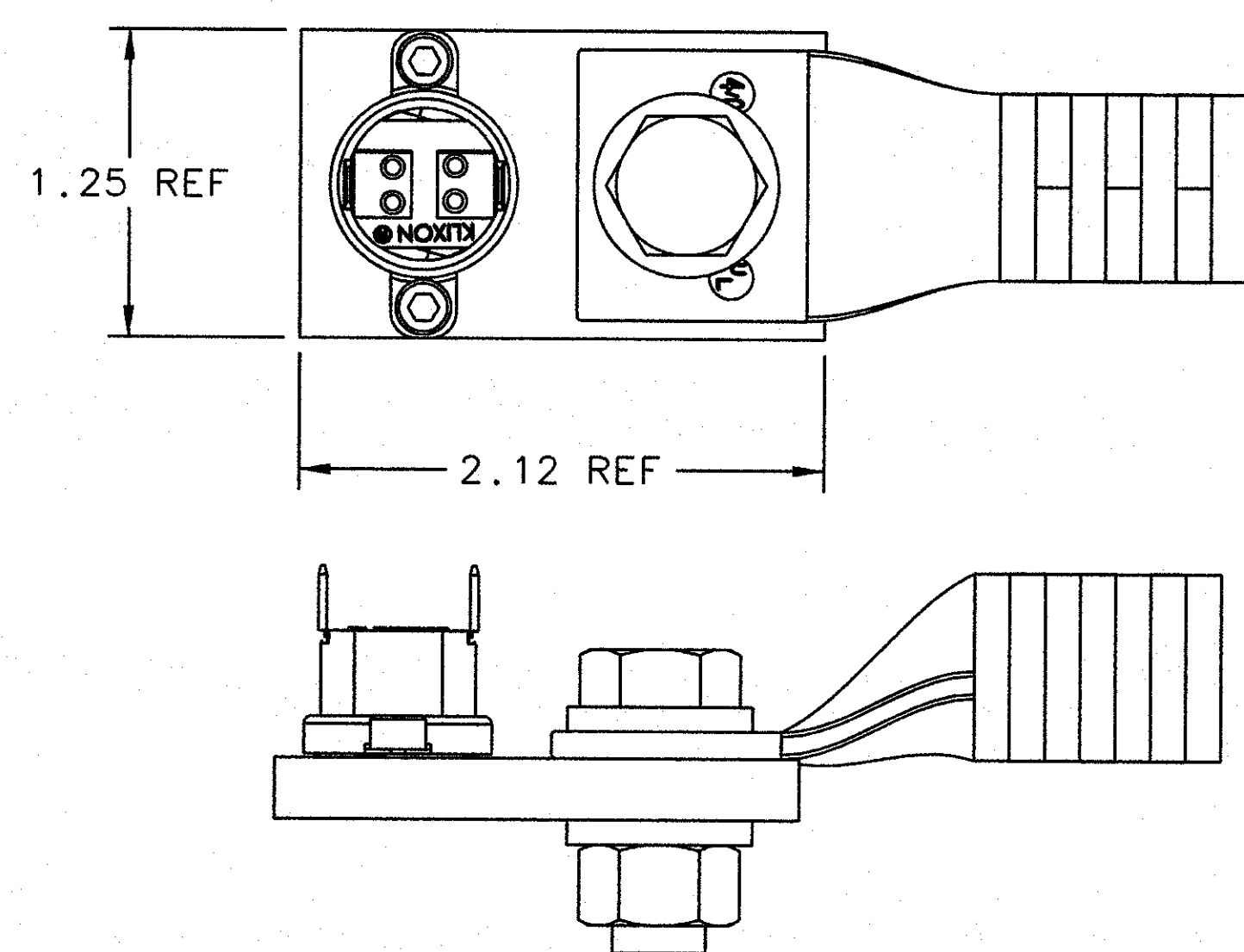
DETAIL VIEW 4-5A - 4 REQD SCALE 1-1/2:1 (TYP CONN FOR WARM WATER ON LEADS)
