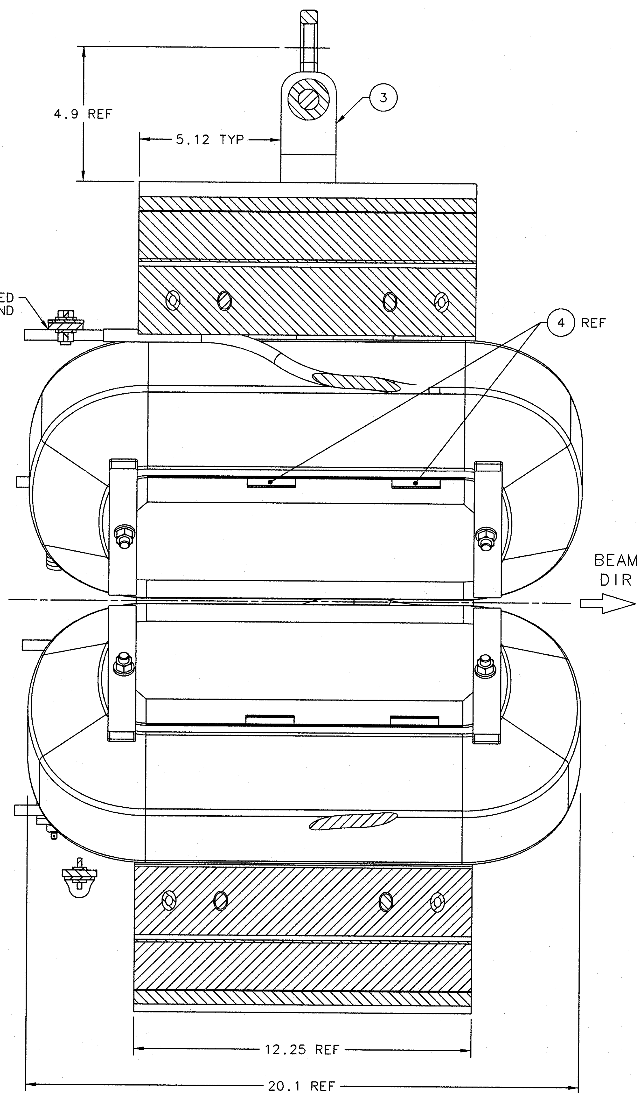
SECTION VIEW 4-3C (4-7C)
