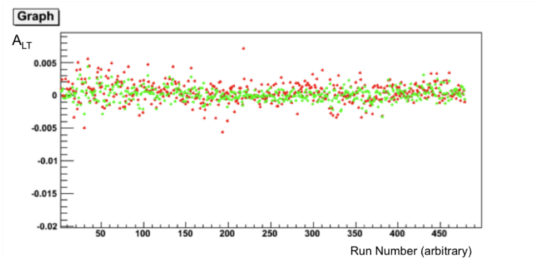
FIG. 5.18: The livetime asymmetry for E07-013. The red points are for T1 and the green are T6, which makes up over 90% of all data. The average value is 1.5 \times 10^{-4} .
