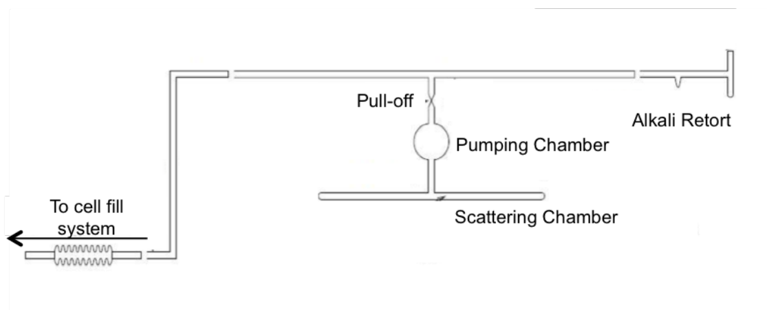
FIG. 4.8: A ^3\text{He} cell before being removed from the string.
