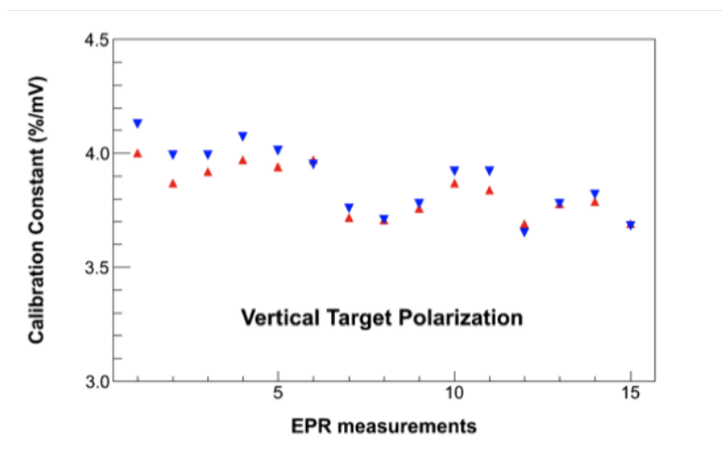
FIG. 4.19: Calibration constants for all EPR measurements during E07-013. Red triangles are constants from up sweeps and blue triangles are constants from down sweeps.
