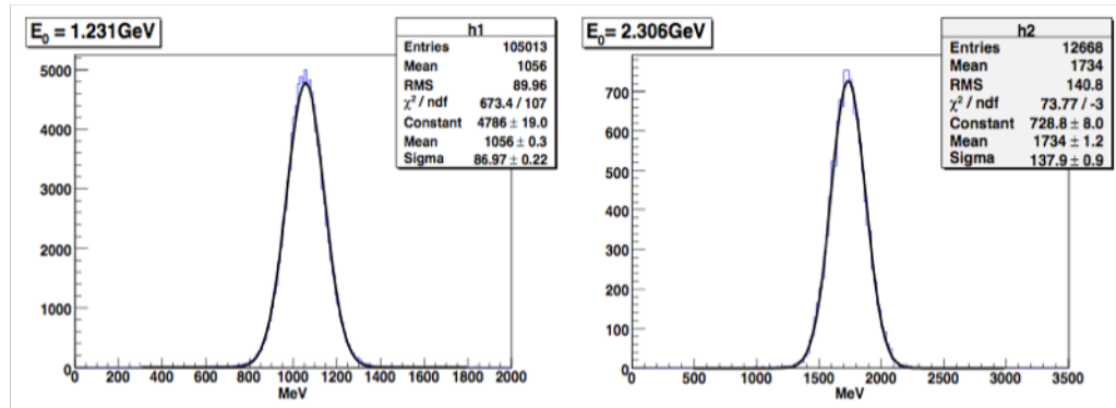
FIG. 3.10: Electron energy reconstruction for E_b = 1.231 GeV (left) and 2.306 GeV (right). The resolution is given by \sigma/\text{mean} , which is about 8%. The mean is lower than the incoming beam energy since there is some energy loss before the scattered particle reaches the shower.
