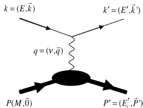
FIG. 1.5: Elastic scattering of an electron from a target with structure
