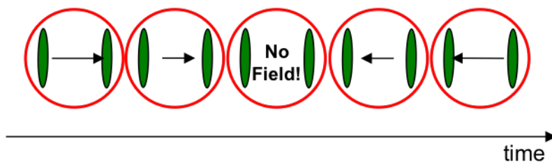
FIG. 4.14: RF field vs. time. The red circle represents the same set of coils as in Figure 4.11. The green coils are the RF generating coils. The pattern repeats as time passes.
