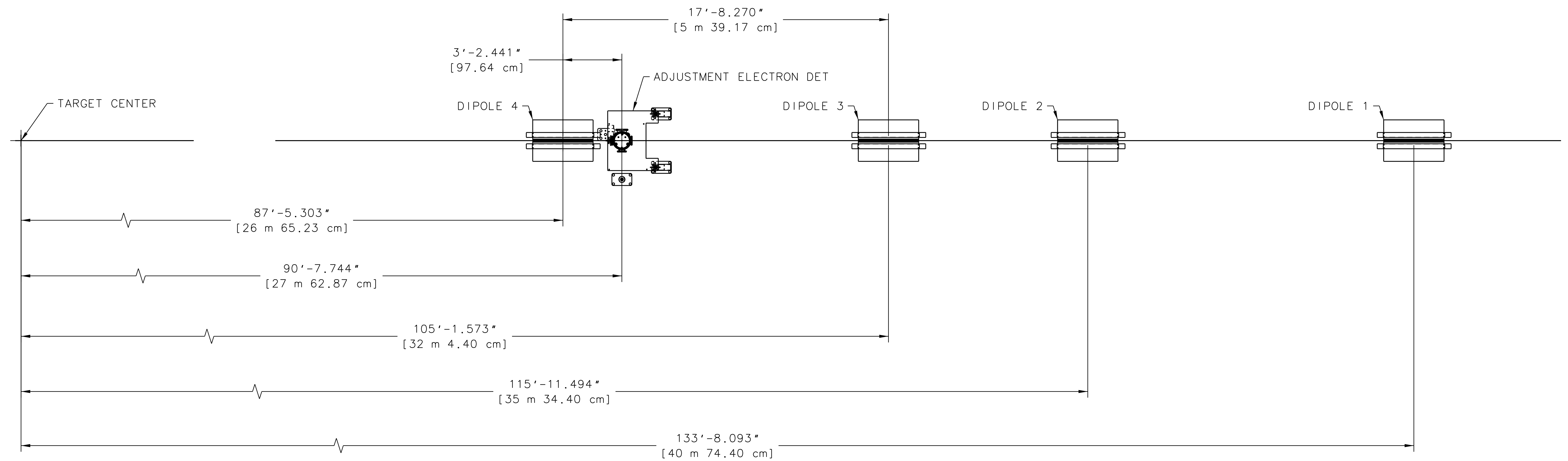
TOP VIEW
