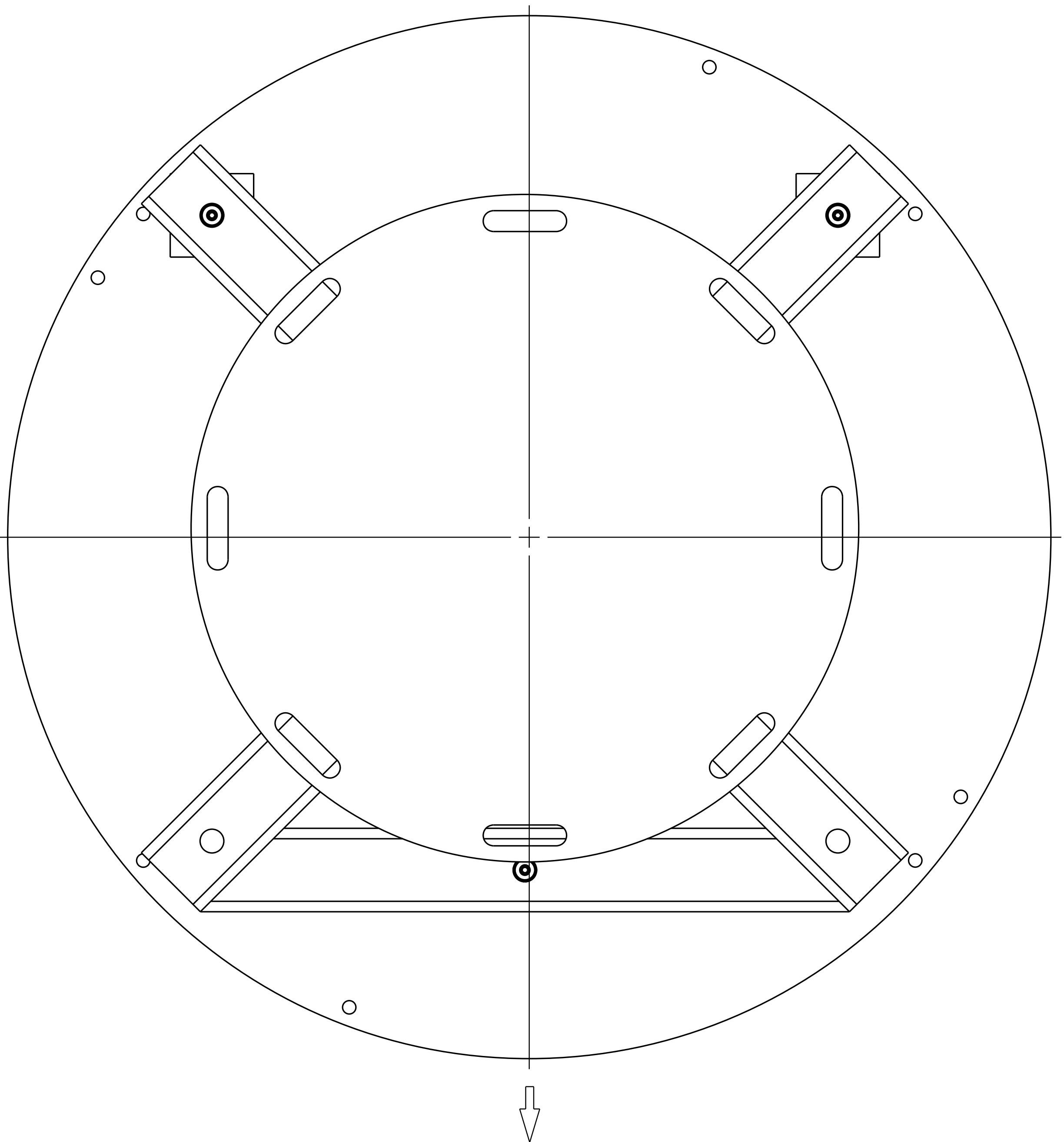
BOTTOM VIEW 1-7A
