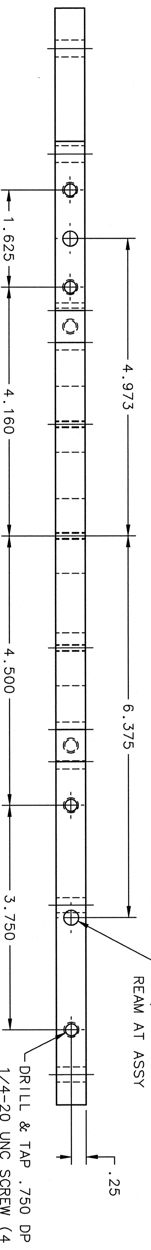
BOTTOM VIEW 1-6A
