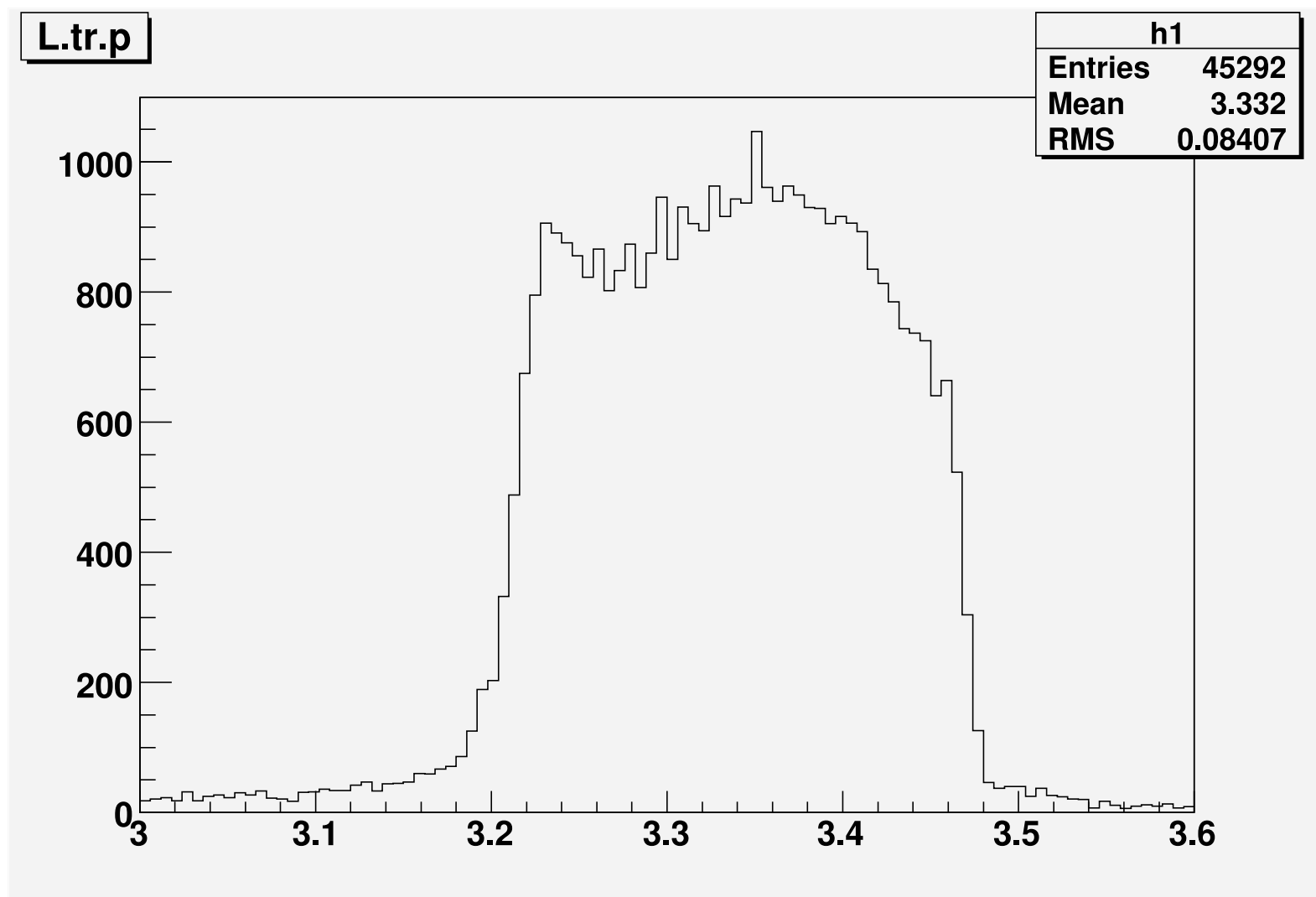
Figure 2: Electron momentum. N20, run 2280
