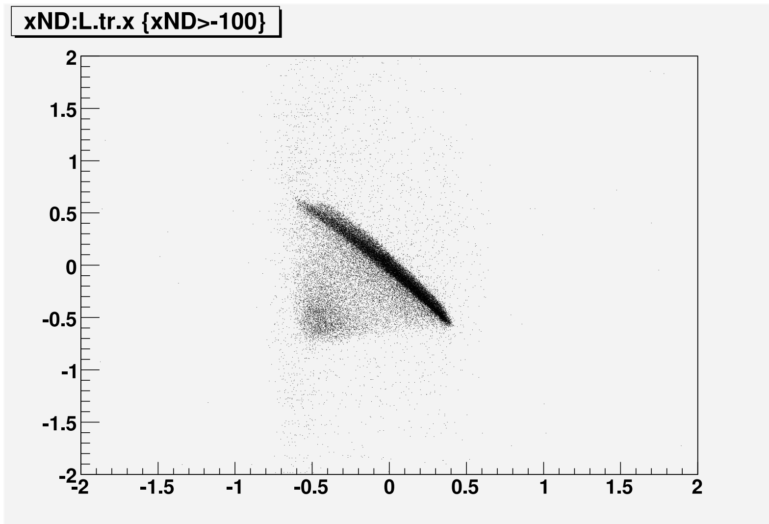
Figure 3: X coordinate in ND vs X in spectrometer. N20, run 2280
