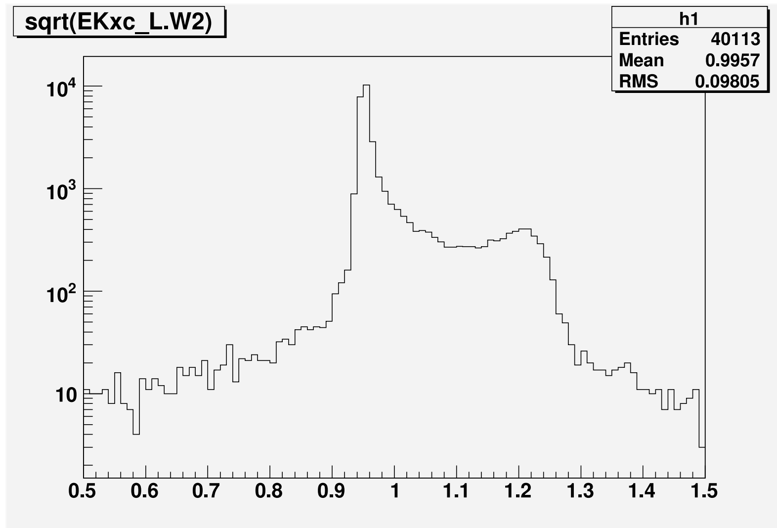
Figure 1: Missing mass distribution. N20, run 2280
