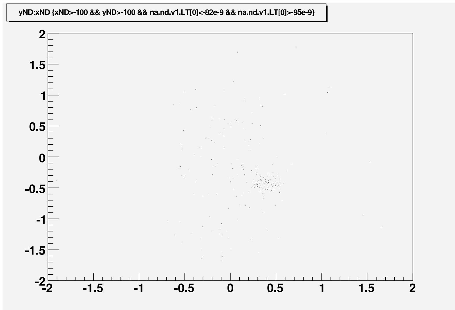
Figure 6: Y coordinate in ND vs X in ND, with cut on one of the left vetos time . N20, run 2280
