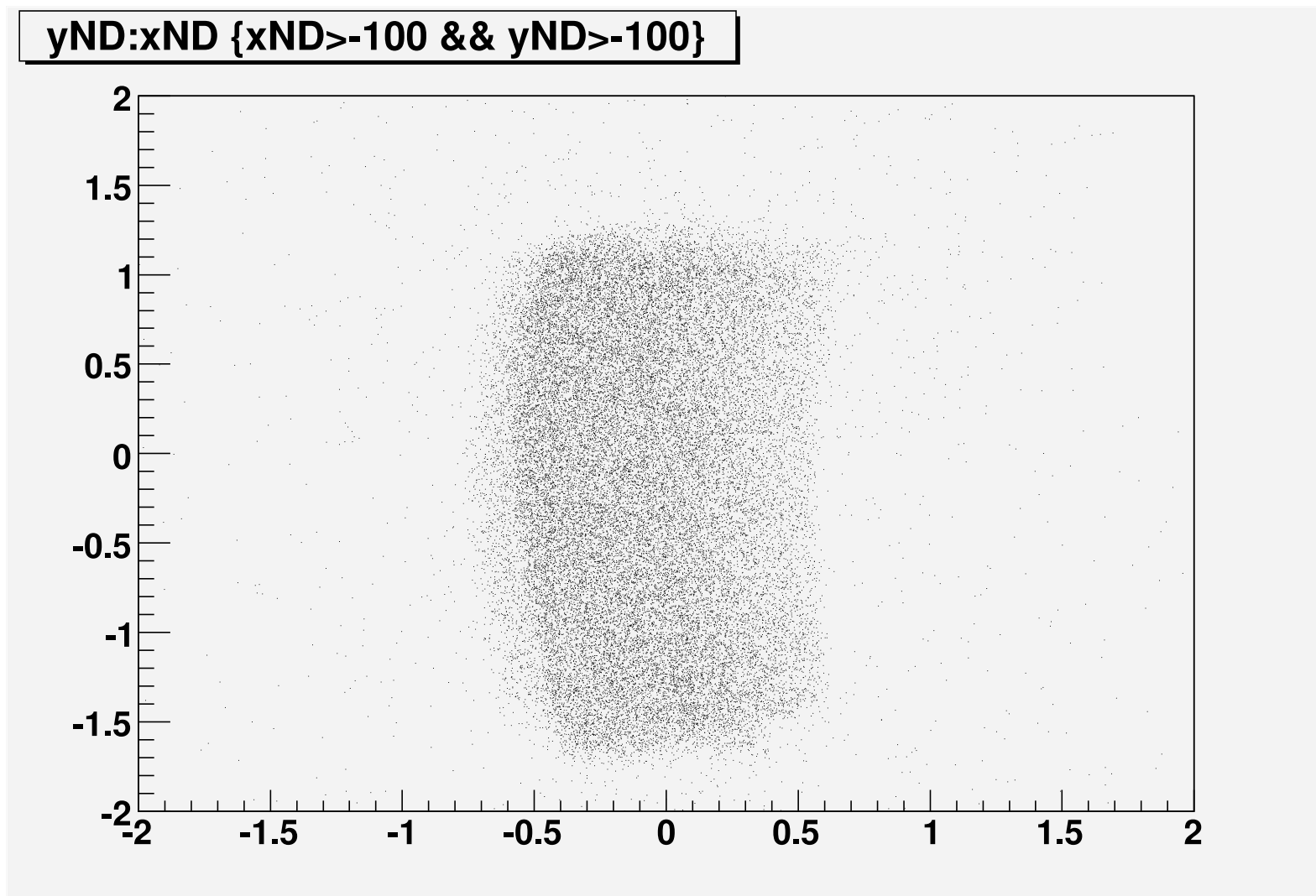
Figure 4: Y coordinate in ND vs X in ND. N20, run 2280
