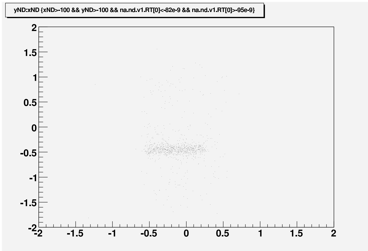
Figure 5: Y coordinate in ND vs X in ND, with cut on one of the right vetos time. N20, run 2280
