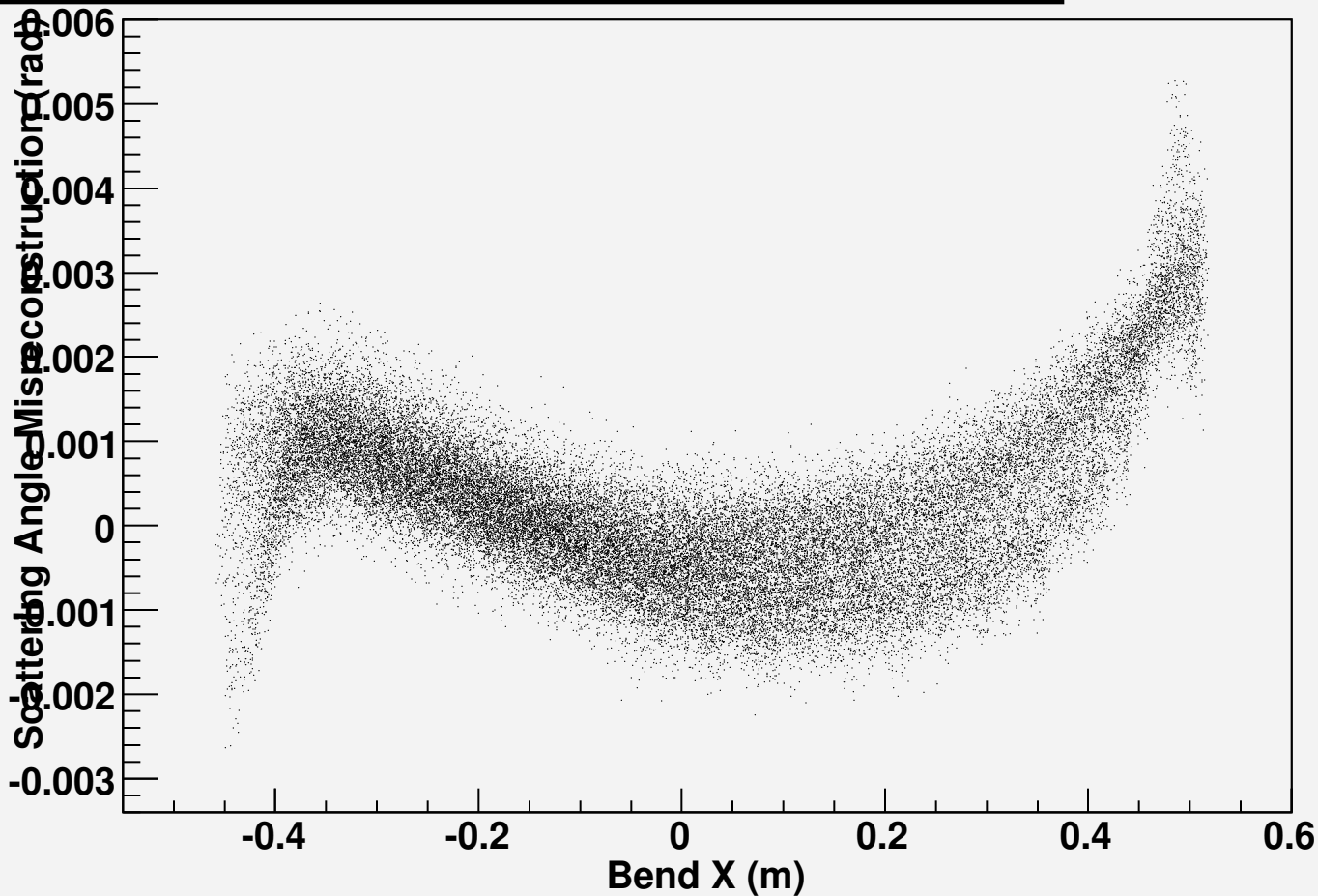
Scattering Angle Misreconstruction vs Bend X - Simulation
