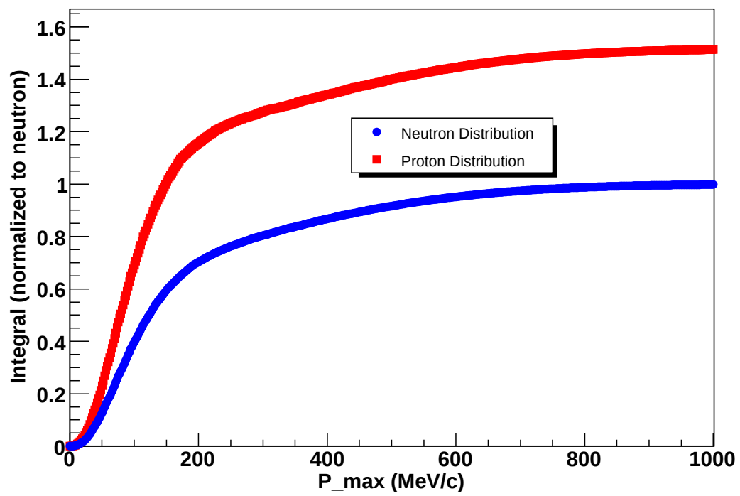
Integral of Density
