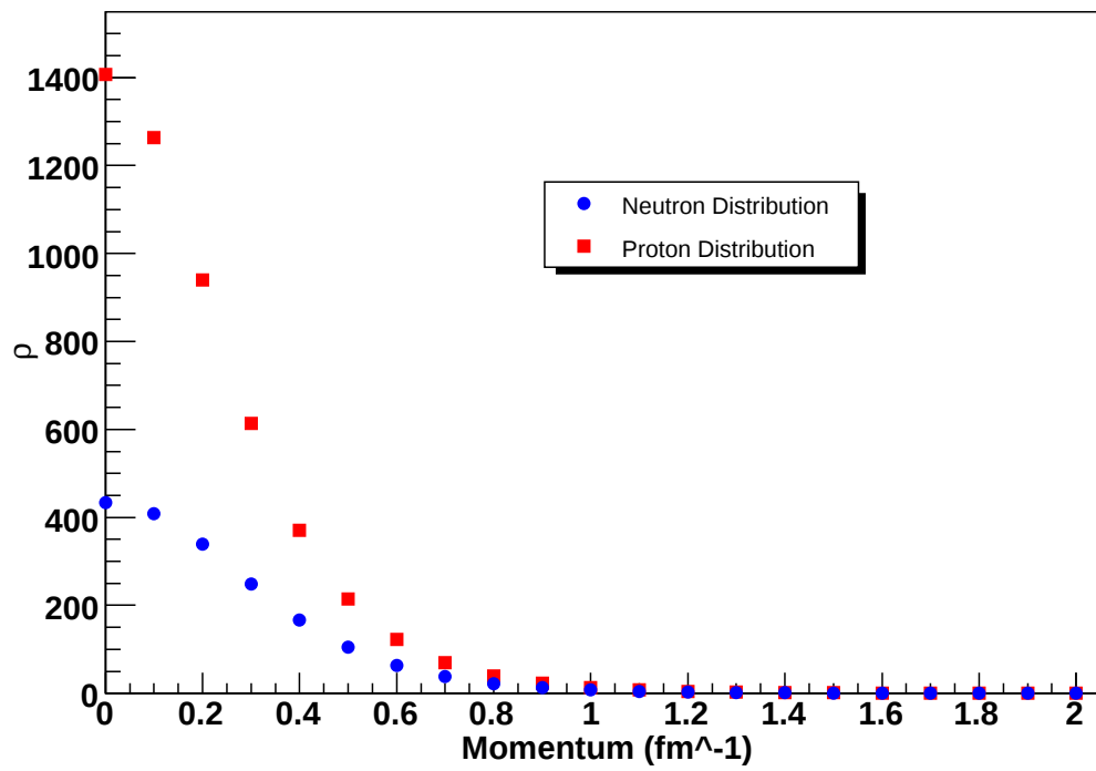
Density v. Momentum
