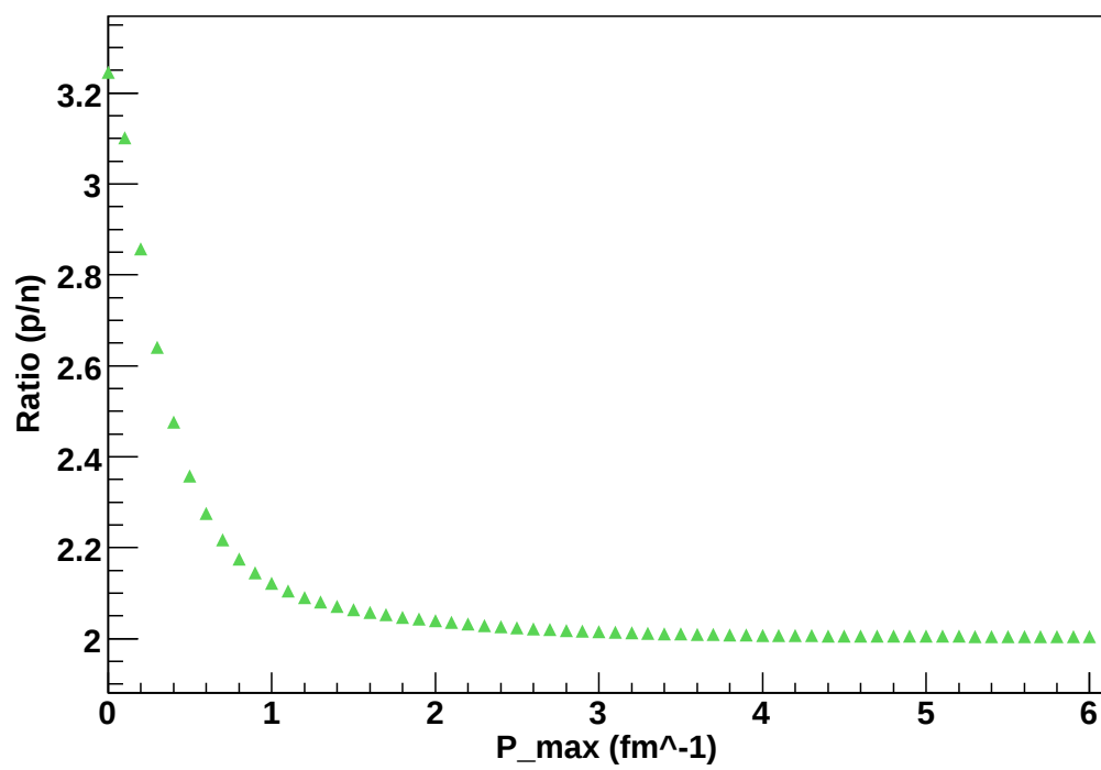
Ratio of Integrals
