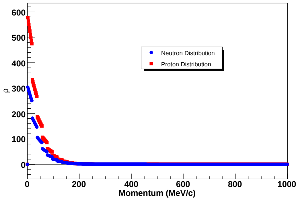
Density v. Momentum
