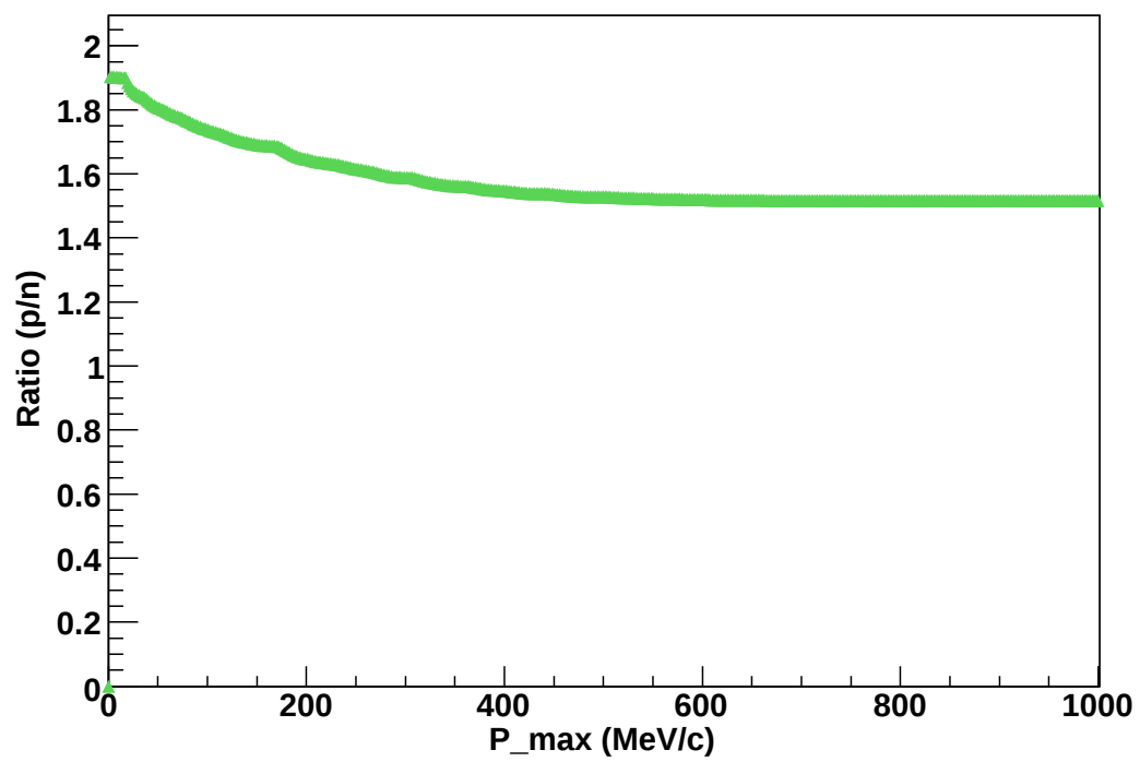
Ratio of Integrals
