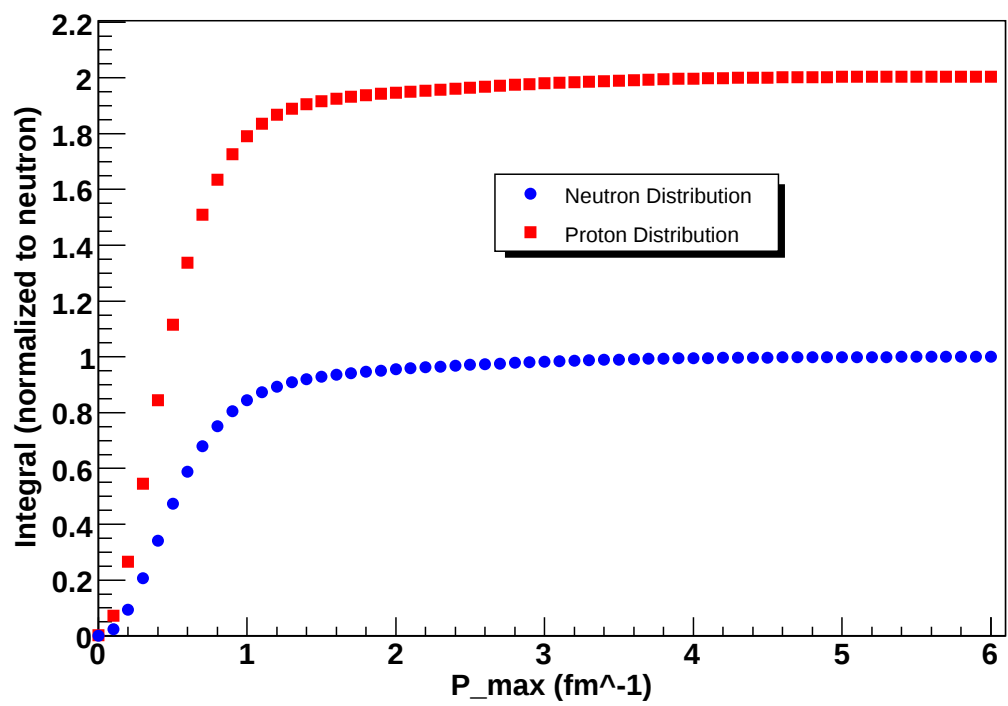
Integral of Density
