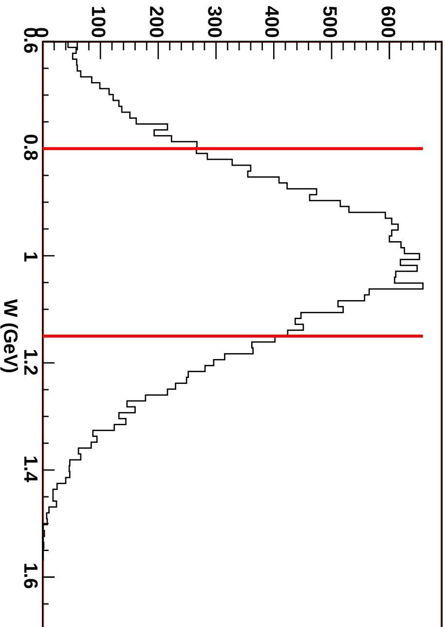
Invariant Mass W - Kinematic 3 - p_{\text{miss},\parallel} cut, p_{\text{miss},\perp} cut
