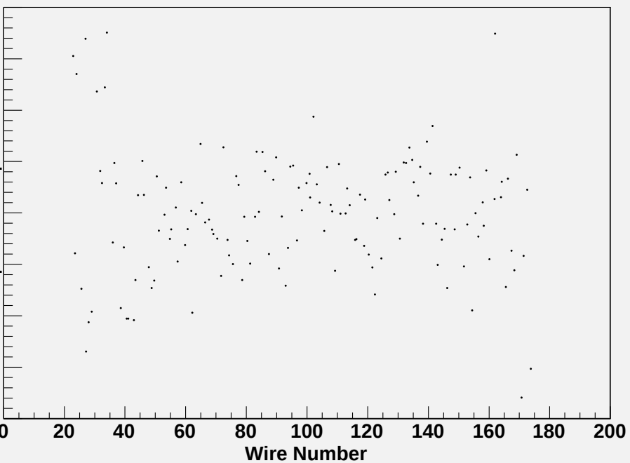
Residual vs wire for plane U3 before optimization
