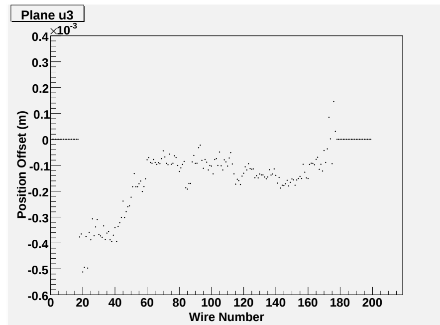
Optimized position for plane U3
