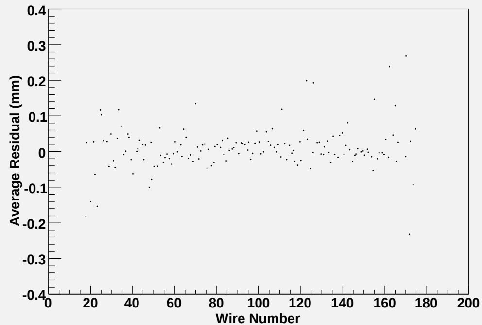
Residual vs wire for plane U3 after optimization
