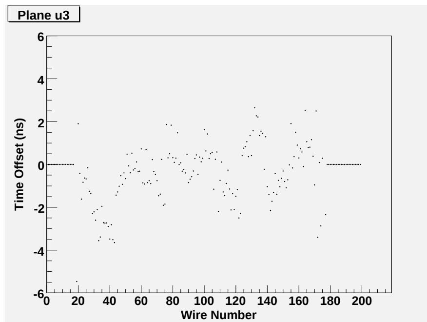
Time offset for plane U3, optimized without position optimization
