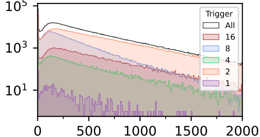
ShowerSum
