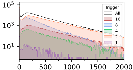
Shower_r
