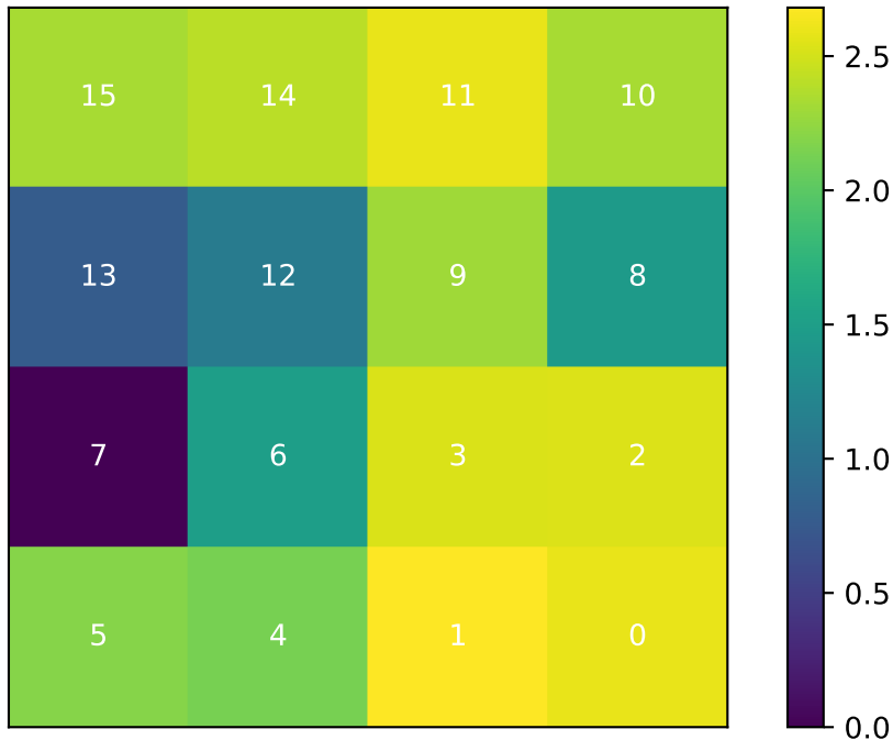
Normalized Sum Before Coincidence Cuts
