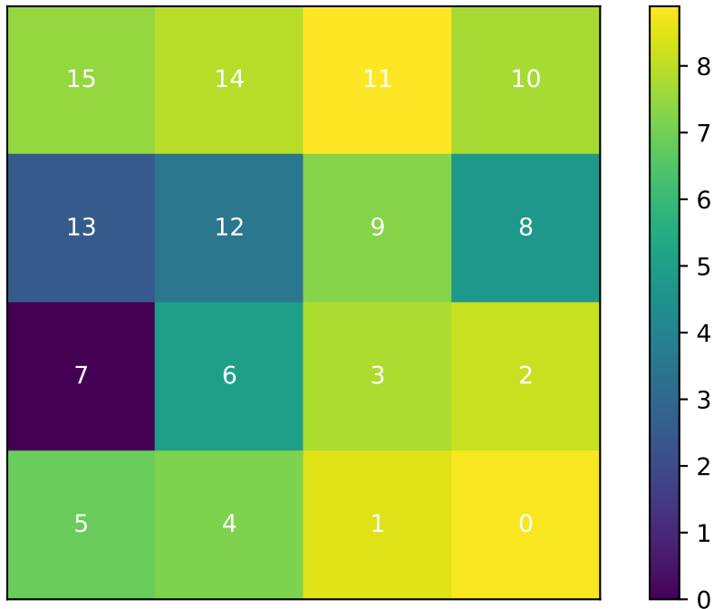
Normalized Sum Before Coincidence Cuts
