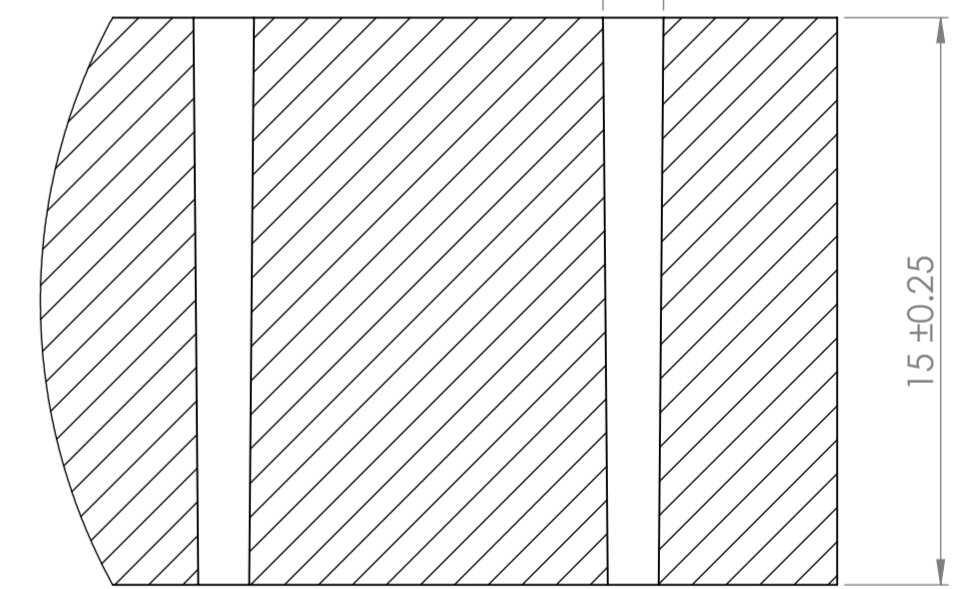
DETAIL B SCALE 5 : 1
