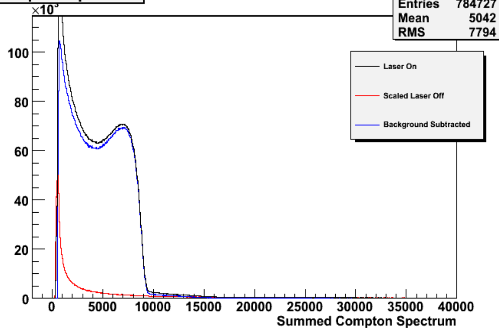
Compton Spectrum
