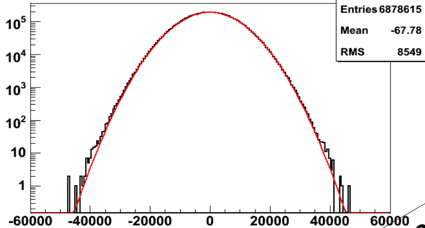
Kinematics #1
