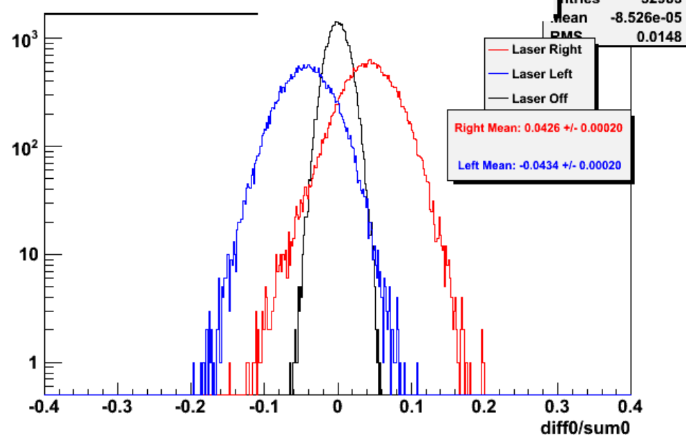
Compton Spectrum
