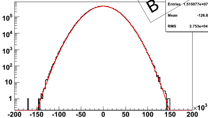
Kinematics #2
