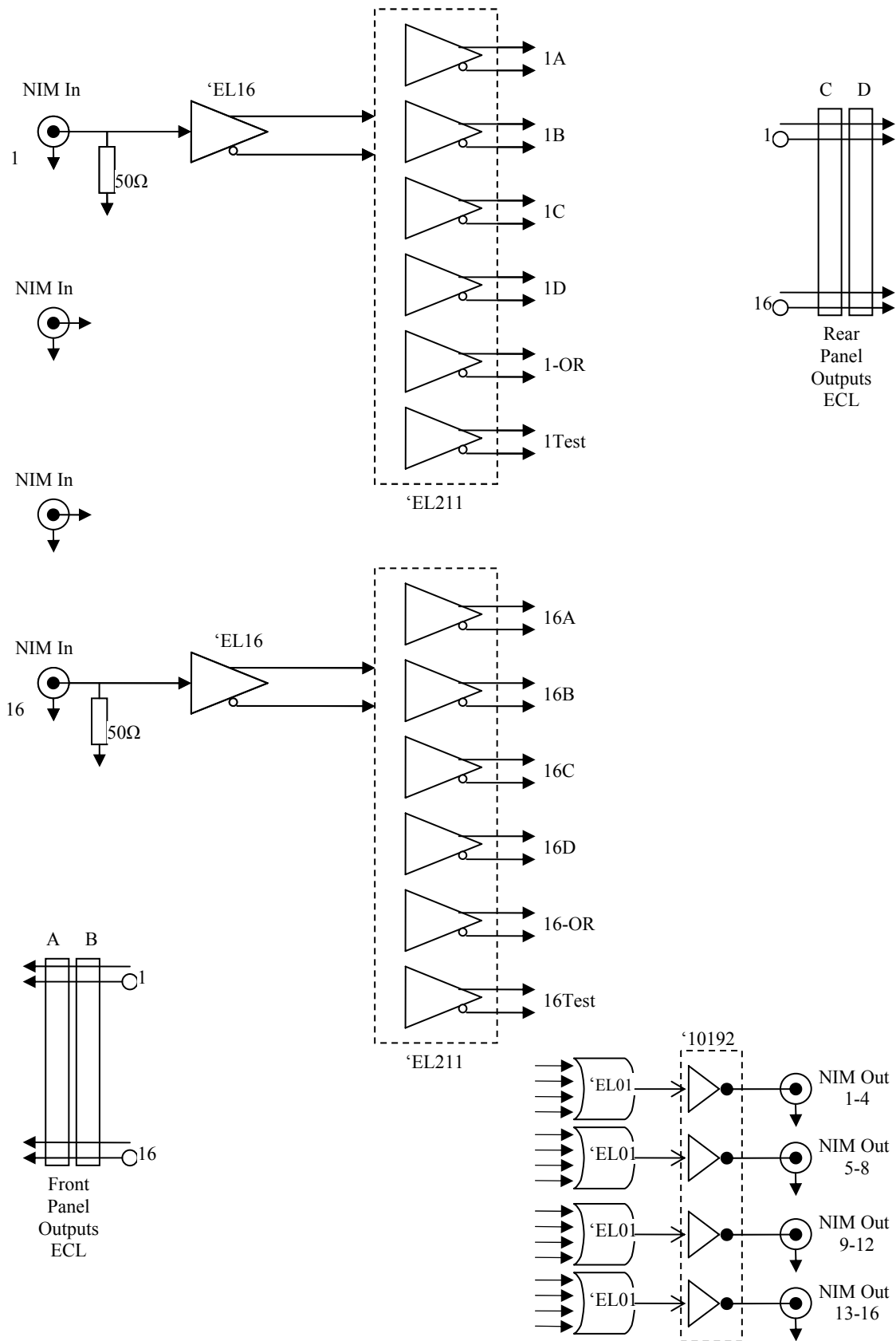
Figure 1: NIM to ECL Fanout Module 1 to 4 Fanout with quad OR NIM output Single Width NIM module
