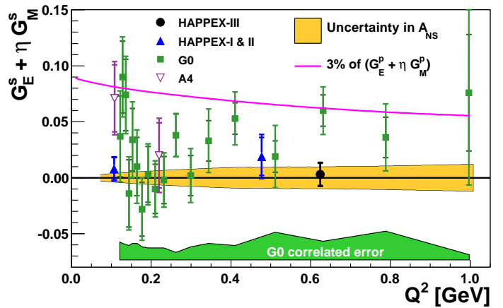
FIG. 2: Results of strange-quark vector form factors for all measurements of forward-angle scattering from the proton. The global fit is described in the text. The solid curve represents a 3% contribution to the comparable linear combination of proton form factors.
