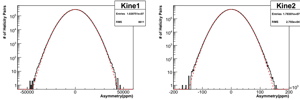
Fig. 9. Blinded counting asymmetry in ppm for the global electron narrow trigger for Q^2 = 1.1 and Q^2 = 1.9 (GeV/c) ^2 . Data for Q^2 = 1.1 (GeV/c) ^2 were collected only on the Left HRS and the whole data set is shown. Data for Q^2 = 1.9 (GeV/c) ^2 were taken on both Left and Right HRSs and only the Right HRS data set is shown, which accounts for about 80% of the total statistics. Data for Q^2 = 1.9 (GeV/c) ^2 collected from the Left HRS shows similar Gaussian distribution but the root-mean-square value is different from the Right HRS due to different rates and DAQ performance.
