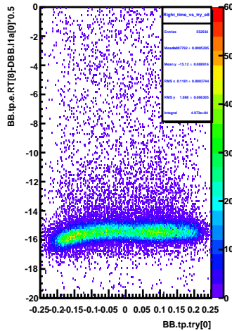
Right_time_vs_try_e8
