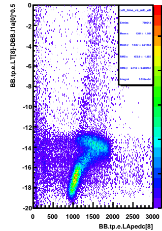
Left_time_vs_adc_e8
