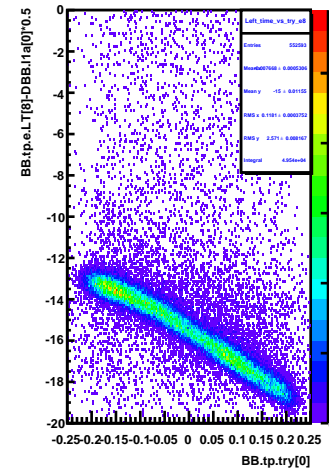
Left_time_vs_try_e8
