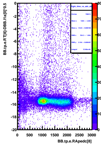
Right_time_vs_adc_e8
