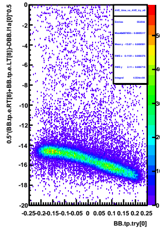
AVE_time_vs_AVE_try_e8
