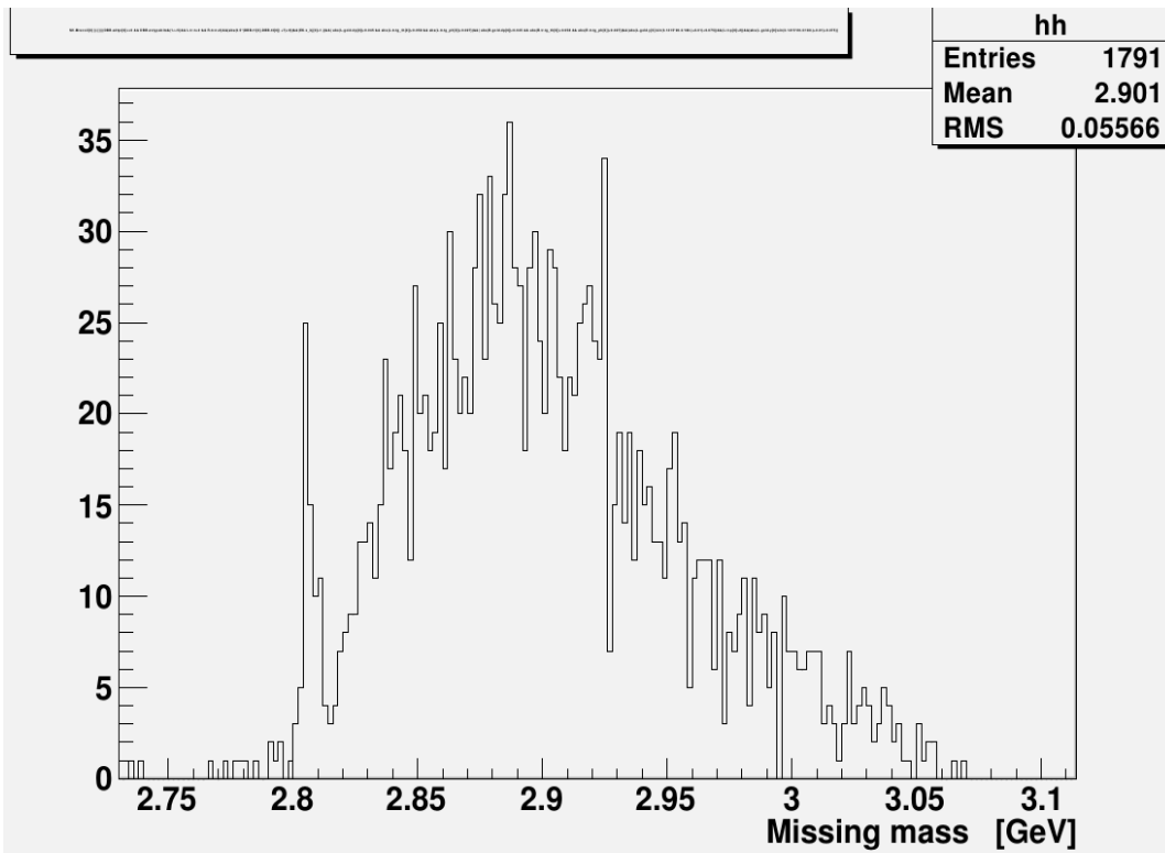
fig2 :Missing mass
