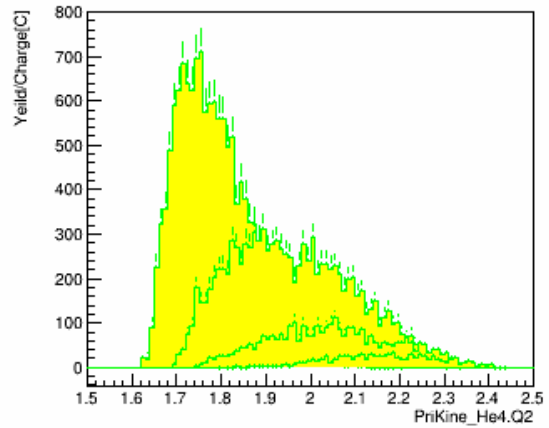
Q2_w_pID_N_CT_sub_bg_kin_3
