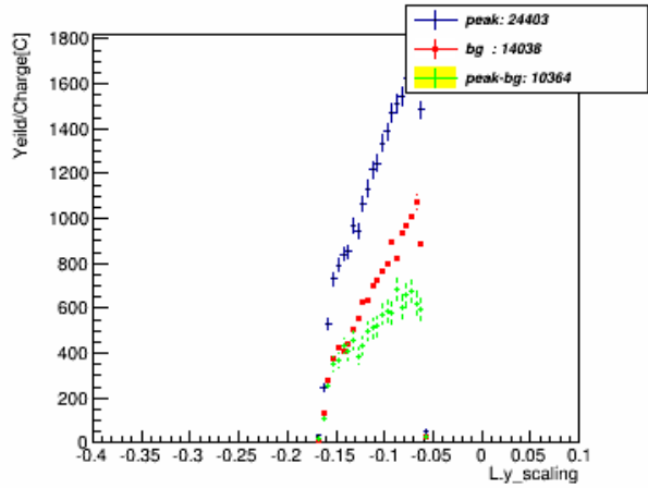
yscaling_w_pID_N_CT_xcut_1.1_to_1.3_kin_3
