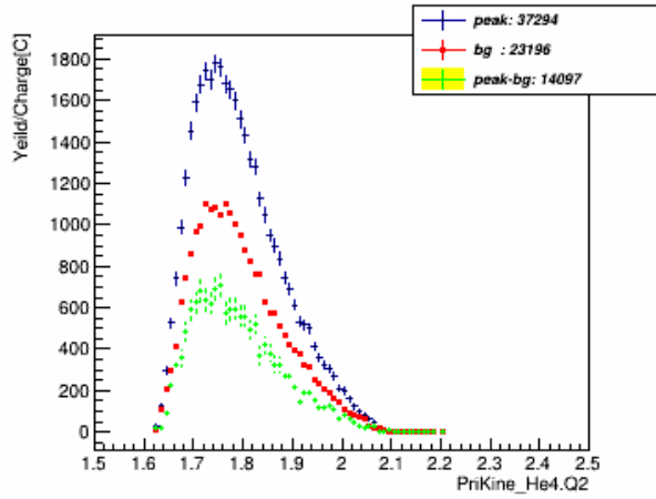
Q2_w_pID_N_CT_xcut_0.9_to_1.1_kin_3
