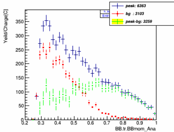
p_w_pID_N_CT_xcut_1.3_to_1.5_kin_3
