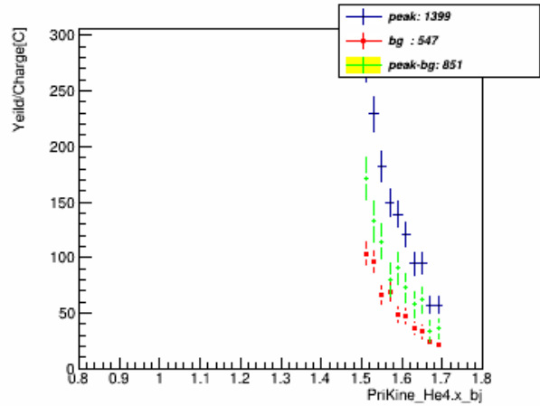
xbj_w_pID_N_CT_xcut_1.5_to_1.7_kin_3
