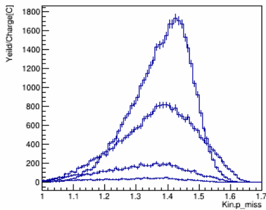
p_miss_w_pID_N_CT_xcut_0.9_to_1.1_kin_3
