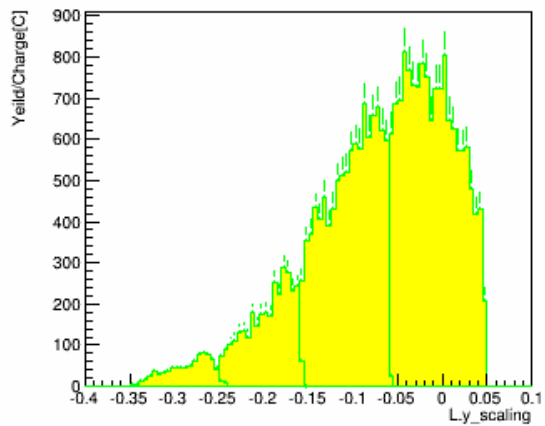
yscaling_w_pID_N_CT_sub_bg_kin_3
