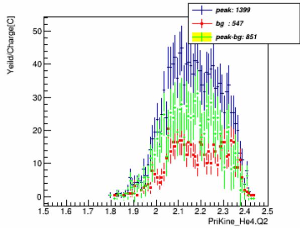
Q2_w_pID_N_CT_xcut_1.5_to_1.7_kin_3
