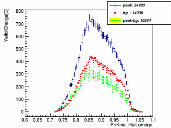
omega_w_pID_N_CT_xcut_1.1_to_1.3_kin_3
