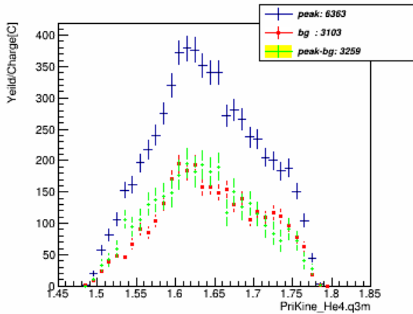
q3m_w_pID_N_CT_xcut_1.3_to_1.5_kin_3
