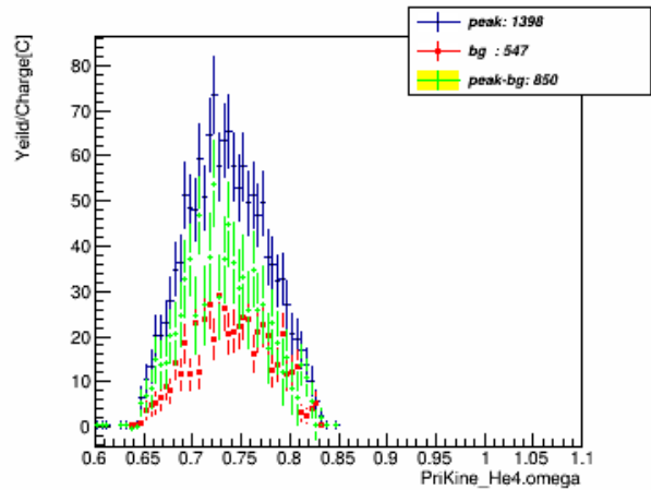
omega_w_pID_N_CT_xcut_1.5_to_1.7_kin_3
