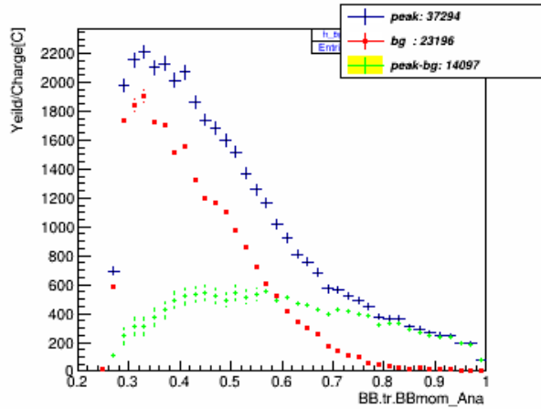
p_w_pID_N_CT_xcut_0.9_to_1.1_kin_3
