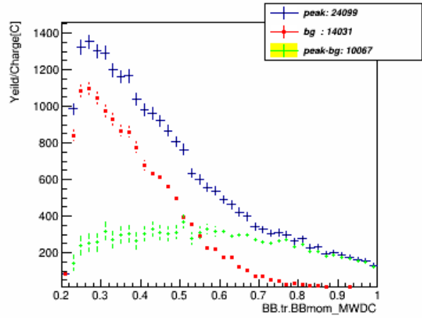
p_MWDC_w_pID_N_CT_xcut_1.1_to_1.3_kin_3
