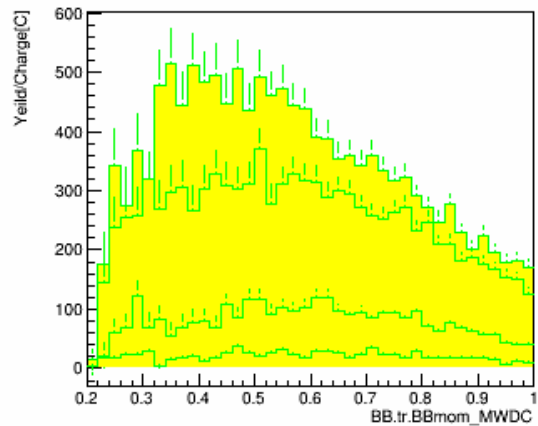
p_MWDC_w_pID_N_CT_sub_bg_kin_3
