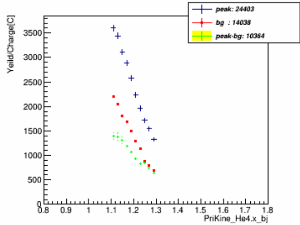
xbj_w_pID_N_CT_xcut_1.1_to_1.3_kin_3
