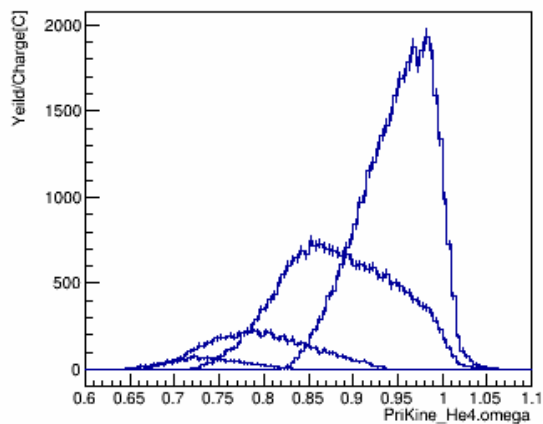
omega_w_pID_N_CT_xcut_0.9_to_1.1_kin_3
