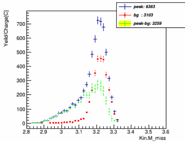
M_miss_w_pID_N_CT_xcut_1.3_to_1.5_kin_3
