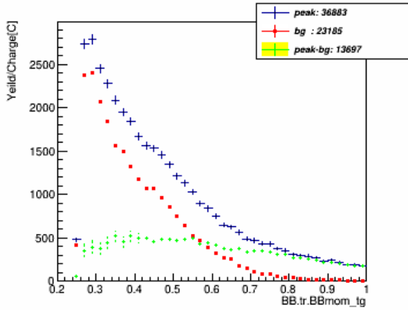
p_tg_w_pID_N_CT_xcut_0.9_to_1.1_kin_3
