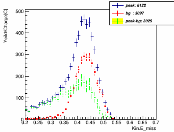
E_miss_w_pID_N_CT_xcut_1.3_to_1.5_kin_3
