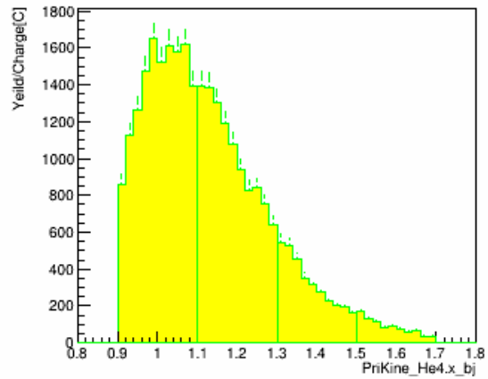
xbj_w_pID_N_CT_sub_bg_kin_3
