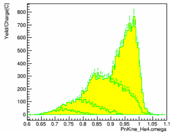
omega_w_pID_N_CT_sub_bg_kin_3
