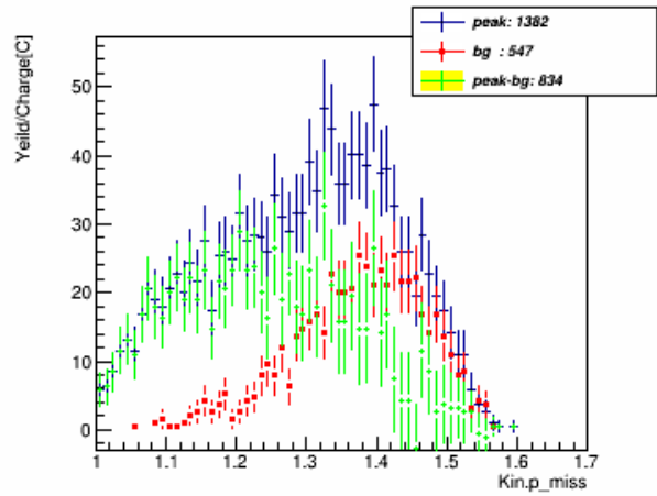
p_miss_w_pID_N_CT_xcut_1.5_to_1.7_kin_3
