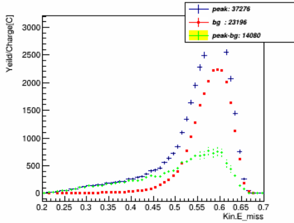
E_miss_w_pID_N_CT_xcut_0.9_to_1.1_kin_3
