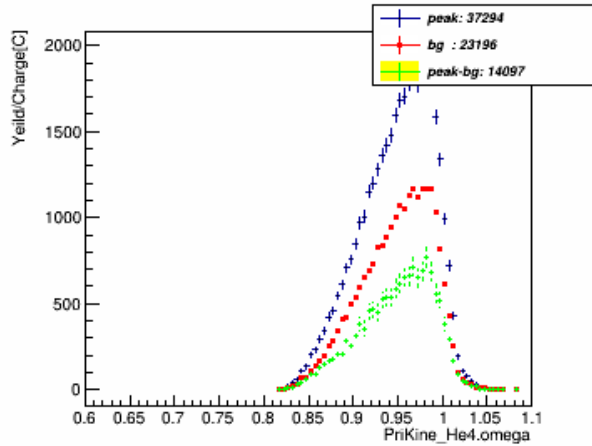
omega_w_pID_N_CT_xcut_0.9_to_1.1_kin_3
