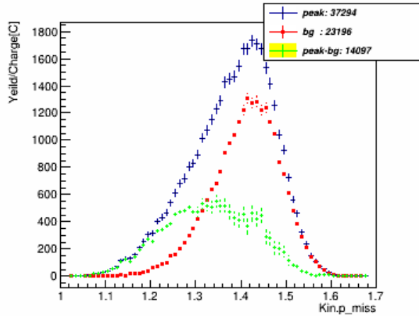
p_miss_w_pID_N_CT_xcut_0.9_to_1.1_kin_3
