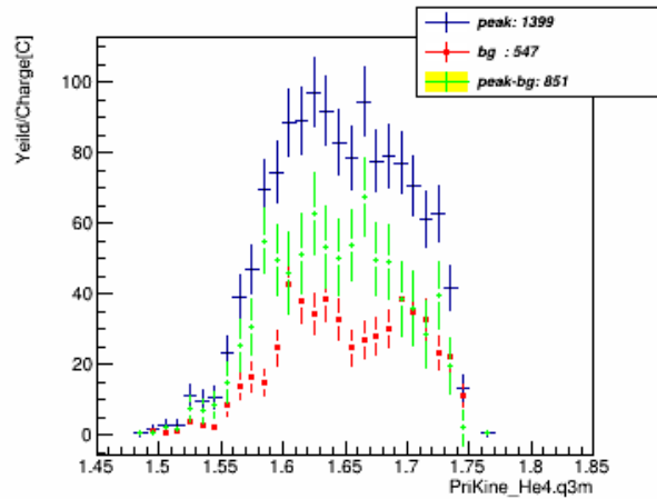
q3m_w_pID_N_CT_xcut_1.5_to_1.7_kin_3
