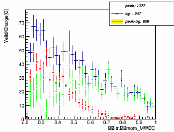
p_MWDC_w_pID_N_CT_xcut_1.5_to_1.7_kin_3
