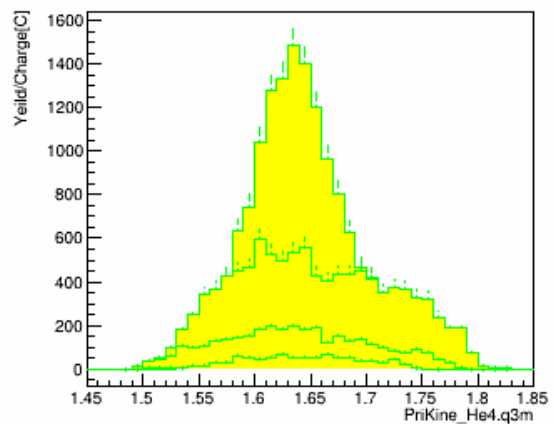
q3m_w_pID_N_CT_sub_bg_kin_3
