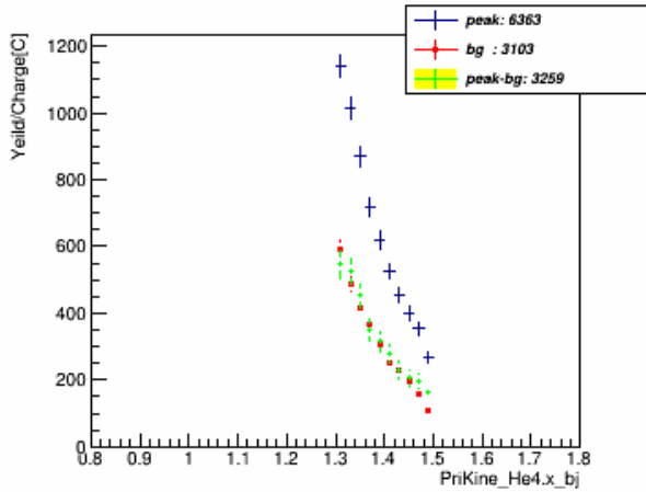
xbj_w_pID_N_CT_xcut_1.3_to_1.5_kin_3
