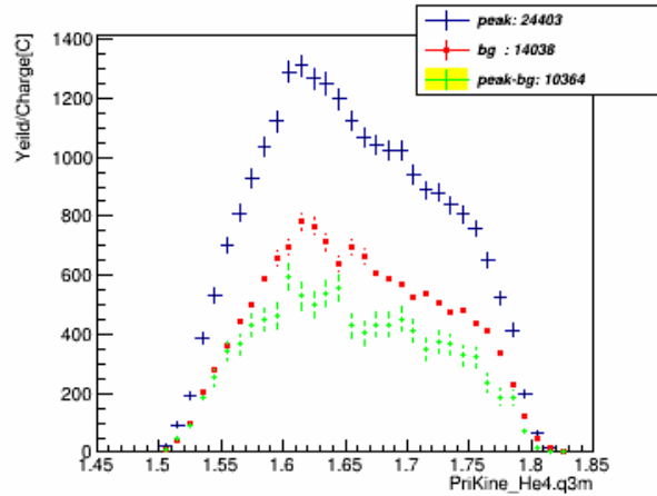
q3m_w_pID_N_CT_xcut_1.1_to_1.3_kin_3
