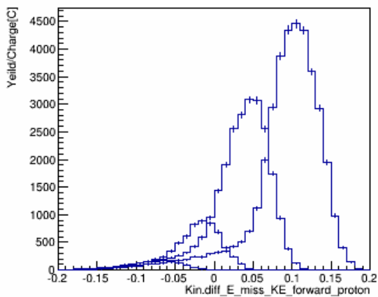
E_miss_forward_w_pID_N_CT_xcut_0.9_to_1.1_kin_3
