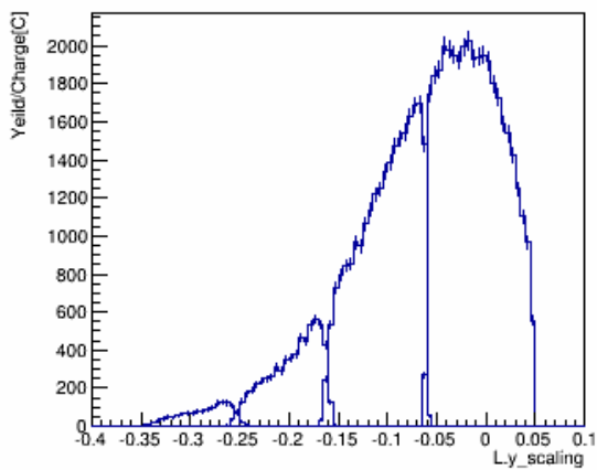
yscaling_w_pID_N_CT_xcut_0.9_to_1.1_kin_3
