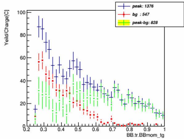
p_tg_w_pID_N_CT_xcut_1.5_to_1.7_kin_3
