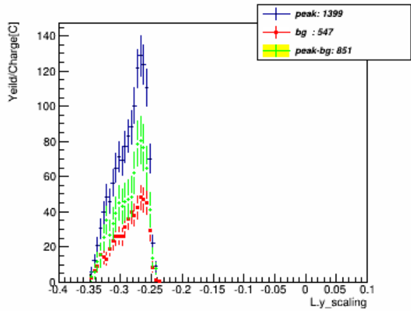
yscaling_w_pID_N_CT_xcut_1.5_to_1.7_kin_3
