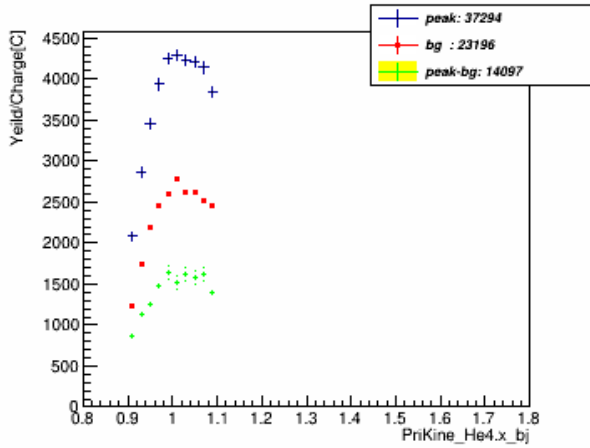
xbj_w_pID_N_CT_xcut_0.9_to_1.1_kin_3
