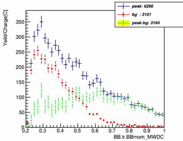
p_MWDC_w_pID_N_CT_xcut_1.3_to_1.5_kin_3
