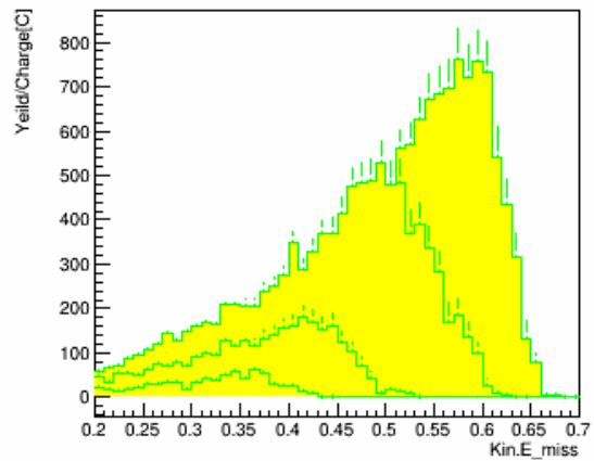
E_miss_w_pID_N_CT_sub_bg_kin_3
