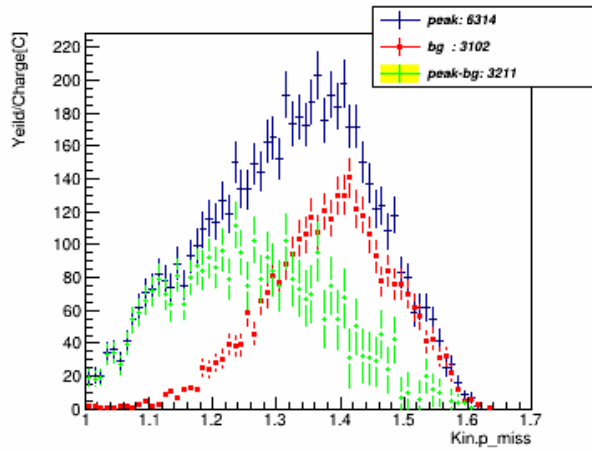
p_miss_w_pID_N_CT_xcut_1.3_to_1.5_kin_3
