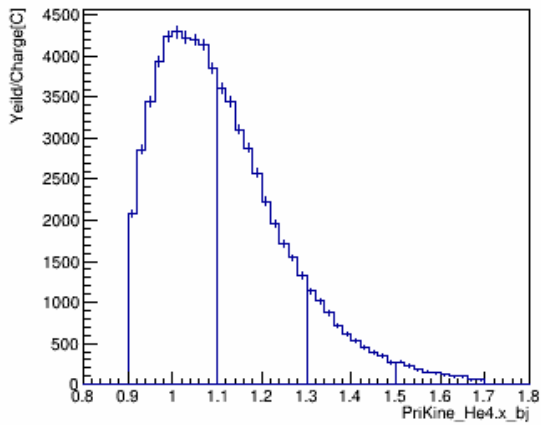
xbj_w_pID_N_CT_xcut_0.9_to_1.1_kin_3
