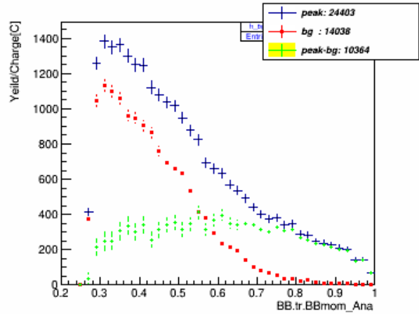
p_w_pID_N_CT_xcut_1.1_to_1.3_kin_3
