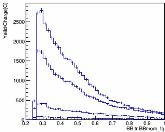
p_tg_w_pID_N_CT_xcut_0.9_to_1.1_kin_3
