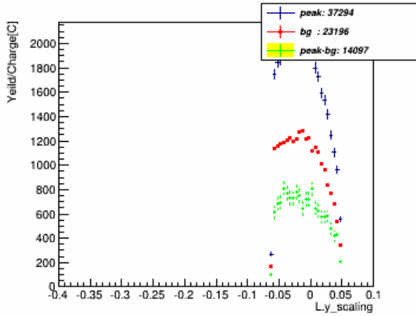
yscaling_w_pID_N_CT_xcut_0.9_to_1.1_kin_3
