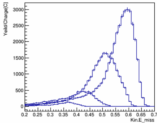
E_miss_w_pID_N_CT_xcut_0.9_to_1.1_kin_3
