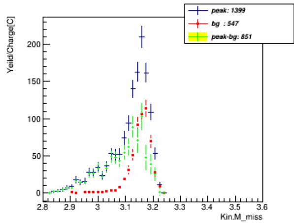
M_miss_w_pID_N_CT_xcut_1.5_to_1.7_kin_3
