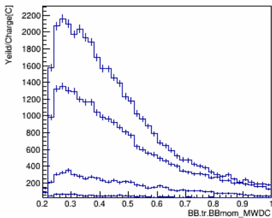
p_MWDC_w_pID_N_CT_xcut_0.9_to_1.1_kin_3
