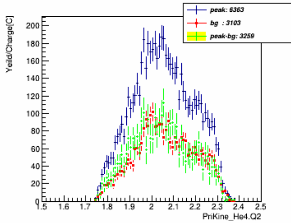
Q2_w_pID_N_CT_xcut_1.3_to_1.5_kin_3
