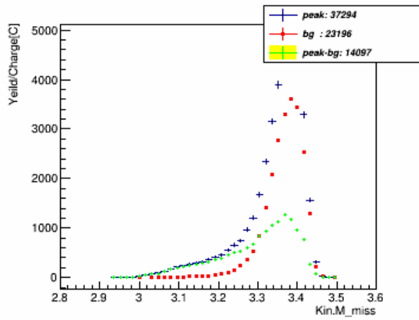
M_miss_w_pID_N_CT_xcut_0.9_to_1.1_kin_3
