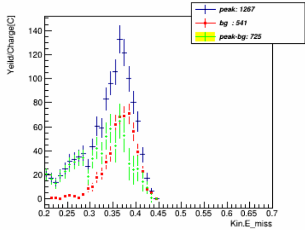
E_miss_w_pID_N_CT_xcut_1.5_to_1.7_kin_3
