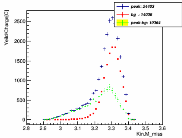
M_miss_w_pID_N_CT_xcut_1.1_to_1.3_kin_3
