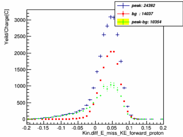
E_miss_forward_w_pID_N_CT_xcut_1.1_to_1.3_kin_3
