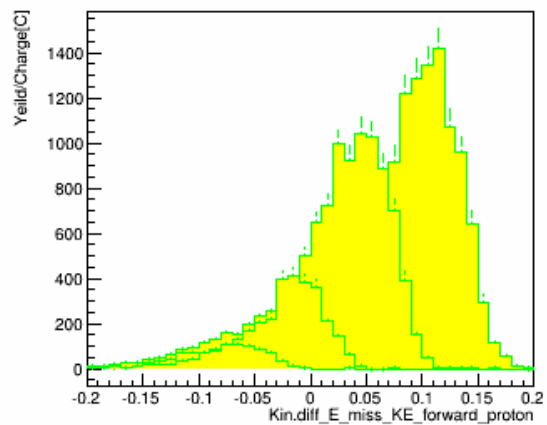
E_miss_forward_w_pID_N_CT_sub_bg_kin_3
