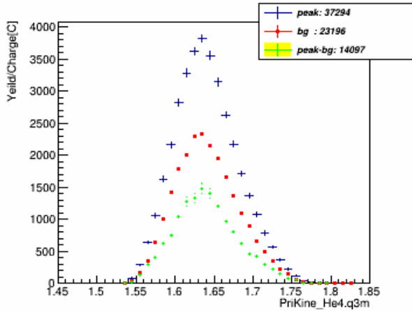
q3m_w_pID_N_CT_xcut_0.9_to_1.1_kin_3
