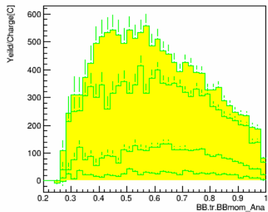
p_w_pID_N_CT_sub_bg_kin_3
