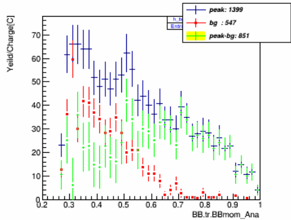
p_w_pID_N_CT_xcut_1.5_to_1.7_kin_3
