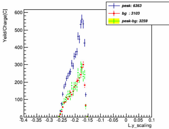
yscaling_w_pID_N_CT_xcut_1.3_to_1.5_kin_3
