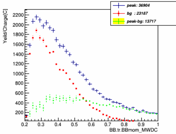
p_MWDC_w_pID_N_CT_xcut_0.9_to_1.1_kin_3
