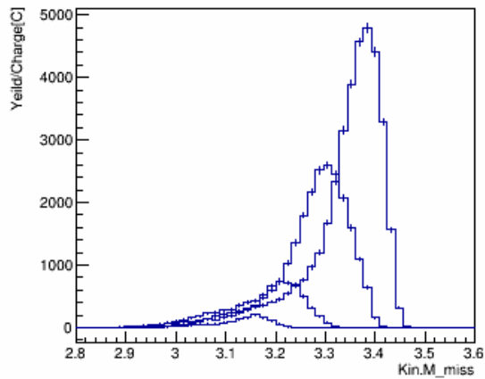
M_miss_w_pID_N_CT_xcut_0.9_to_1.1_kin_3
