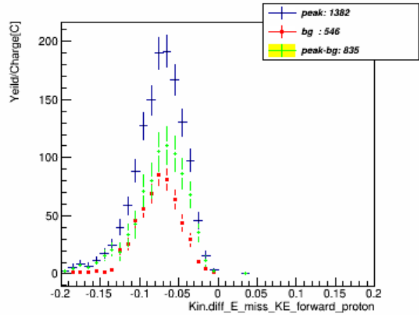
E_miss_forward_w_pID_N_CT_xcut_1.5_to_1.7_kin_3
