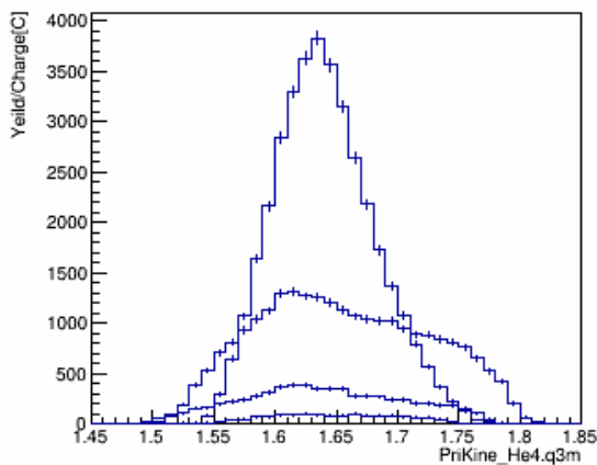
q3m_w_pID_N_CT_xcut_0.9_to_1.1_kin_3
