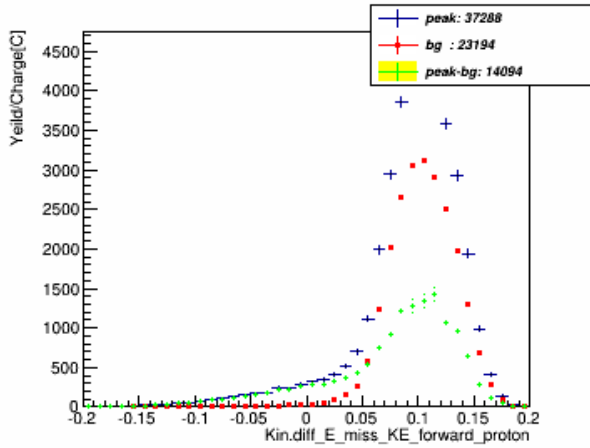
E_miss_forward_w_pID_N_CT_xcut_0.9_to_1.1_kin_3
