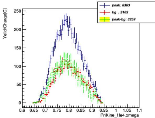
omega_w_pID_N_CT_xcut_1.3_to_1.5_kin_3
