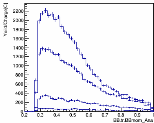
p_w_pID_N_CT_xcut_0.9_to_1.1_kin_3
