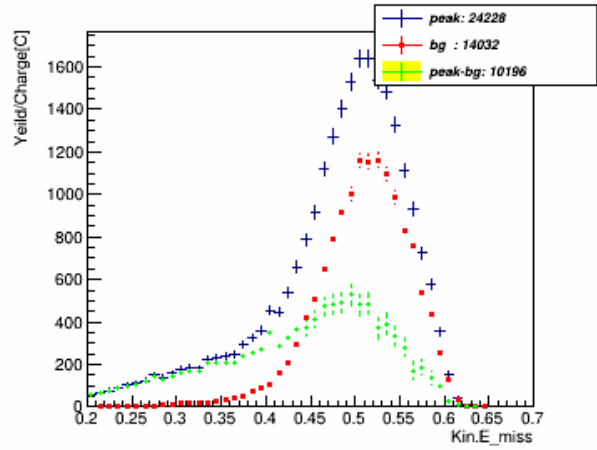
E_miss_w_pID_N_CT_xcut_1.1_to_1.3_kin_3
