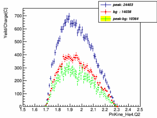
Q2_w_pID_N_CT_xcut_1.1_to_1.3_kin_3
