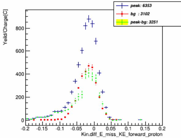
E_miss_forward_w_pID_N_CT_xcut_1.3_to_1.5_kin_3
