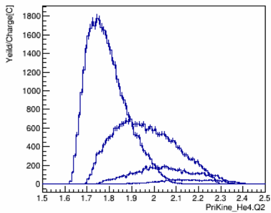
Q2_w_pID_N_CT_xcut_0.9_to_1.1_kin_3
