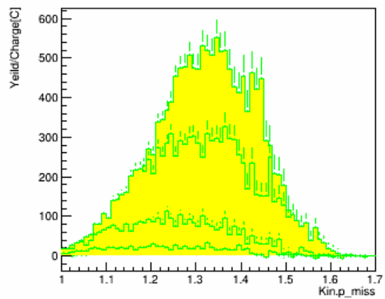
p_miss_w_pID_N_CT_sub_bg_kin_3
