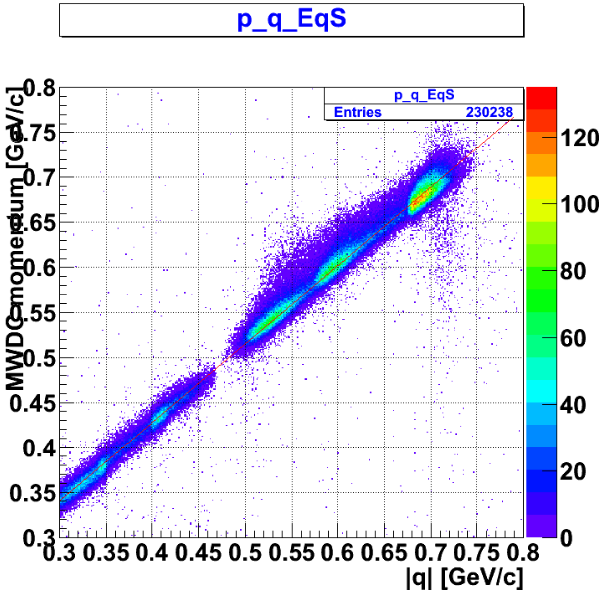
Figure 2.1 expected p from |q| vs MWDC p in [GeV/c] The red line has slope of 0.873 not 1. with offset of 0.078 GeV/c.
