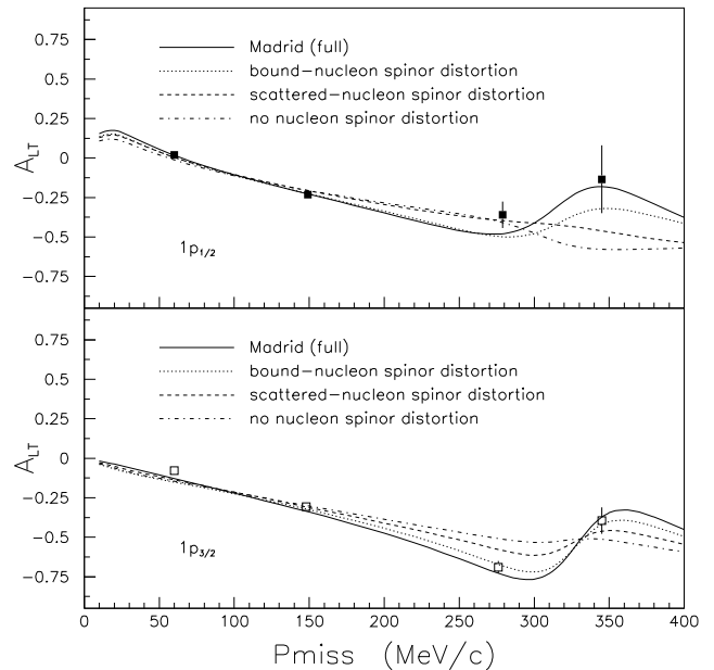
FIG. 15: Left-right asymmetry A_{LT} together with relativistic calculations for the removal of protons from the 1p -shell of ^{16}\text{O} as a function of P_{\text{miss}} for E_{\text{beam}} = 2.442 GeV. Error bars are statistical (see Table XXV for the associated systematic uncertainties). The RDWIA calculations by the Madrid Group. Note that the solid curves shown in this figure are identical to those shown in Figure 14.
