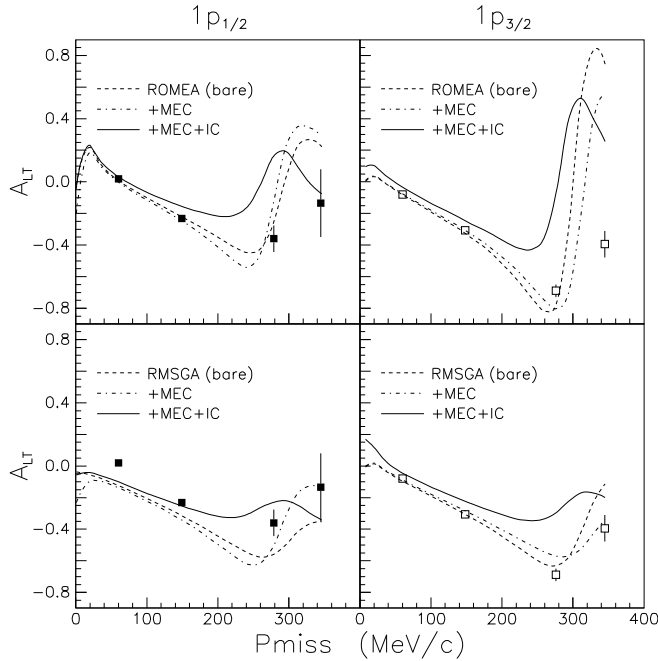
FIG. 19: Left-right asymmetry A_{LT} together with calculations by the Ghent Group of the A_{LT} asymmetry for the removal of protons from the 1p -shell of ^{16}\text{O} as a function of P_{\text{miss}} for E_{\text{beam}} = 2.442 GeV. Error bars are statistical (see Table XXV for the associated systematic uncertainties). The curves labelled “bare” are identical to those shown in Figure 14.
