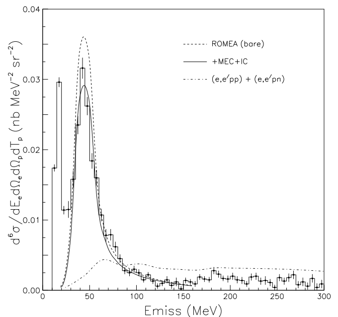
FIG. 25: Data from this work together with calculations by the Ghent Group for the E_{\text{miss}} -dependence of the cross sections obtained in dip-region kinematics for E_{\text{beam}} = 1.643 GeV. Error bars are statistical and on average, there is an additional \pm 5.9\% systematic uncertainty (see Table XXIX) associated with the data.
