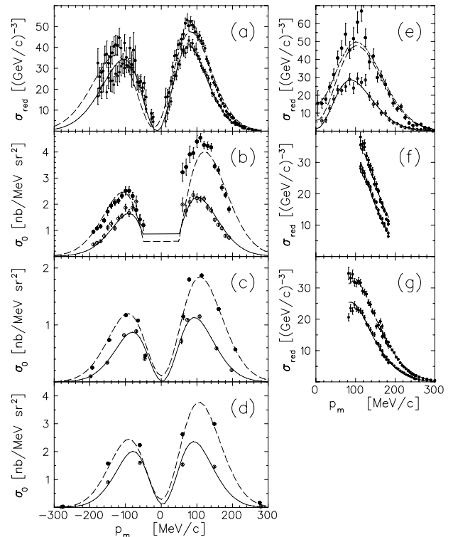
FIG. 11: Fits by Kelly to various ^{16}\text{O}(e, e'p) data sets based on the NLSH bound-nucleon wave function and the EDAL-O optical potential. Open points and solid lines pertain to the 1p_{1/2} -state, while solid points and dashed lines pertain to the 1p_{3/2} -state. The dashed-dotted lines include the contributions of the 2s_{1/2}1d_{5/2} -doublet to the 1p_{3/2} -state. Panel (d) shows the data from this work - see Table VII for the key to the other data sets.
