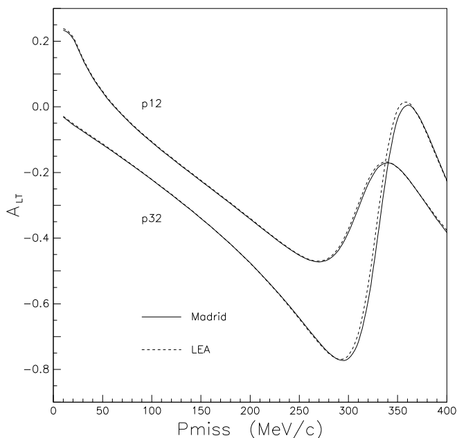
FIG. 8: Baseline RDWIA calculations for the A_{LT} asymmetry by the Madrid Group and Kelly (LEA) for the removal of protons from the 1p -shell of ^{16}\text{O} as a function of P_{\text{miss}} for E_{\text{beam}} = 2.442 GeV. Overall agreement is excellent over the entire P_{\text{miss}} range.
