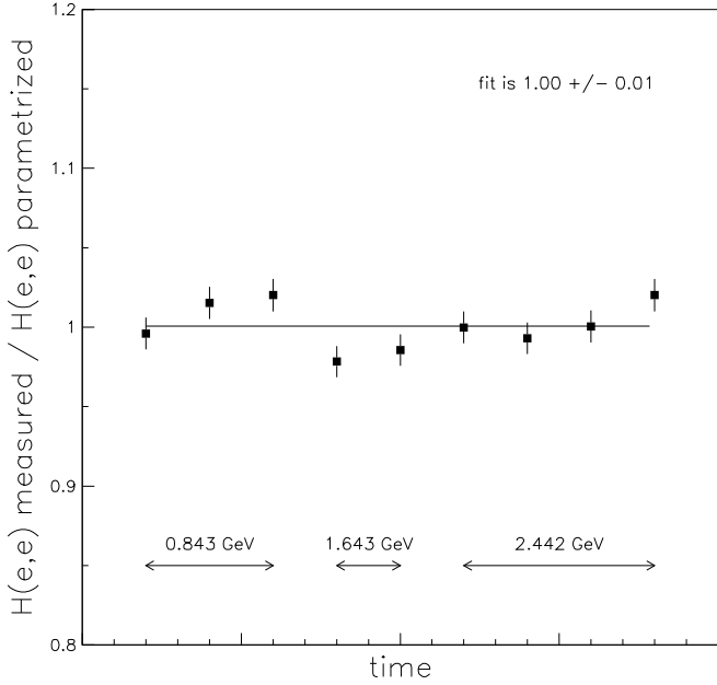
FIG. 4: Measured {}^1\text{H}(e, e) cross sections normalized to the absolute predictions of a parametrization at similar Q^2 . Statistical error bars are shown. The data shown in the figure were taken over the course of a three-month run period. The different data points for each E_{\text{beam}} represent different \text{HRS}_e angular settings.
