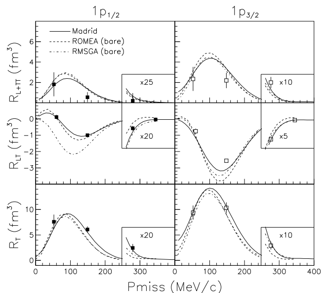
FIG. 17: Data from this work together with relativistic calculations for the R_{L+TT} , R_{LT} , and R_T response functions for the removal of protons from the 1p -shell of ^{16}\text{O} as a function of P_{\text{miss}} . Error bars are statistical (see Tables XXIV, XXV, and XXIII for the associated systematic uncertainties). The solid line is the RDWIA calculation of the Madrid Group, while the dashed and dashed-dotted lines are respectively the “bare” ROMEA and RMSGGA calculations of the Ghent Group.
