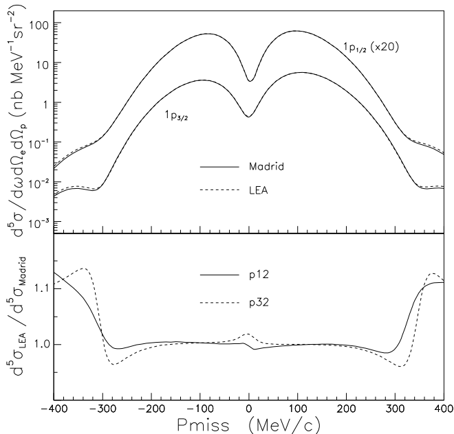
FIG. 7: Baseline RDWIA calculations by the Madrid Group and Kelly (LEA) for the removal of protons from the 1p -shell of ^{16}\text{O} as a function of P_{\text{miss}} for E_{\text{beam}} = 2.442 GeV. For the purposes of this comparison, the input into both calculations was identical (see Table V). Overall agreement is very good, and agreement is excellent for |P_{\text{miss}}| < 250 MeV/ c .
