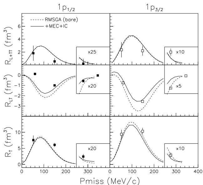
FIG. 21: Data from this work together with RMSGA calculations by the Ghent Group for the R_{L+TT} , R_{LT} , and R_T response functions for the removal of protons from the 1p -shell of ^{16}\text{O} as a function of P_{\text{miss}} . Error bars are statistical (see Tables XXIV, XXV, and XXIII for the associated systematic uncertainties). The curves labelled “bare” are identical to those shown in Figure 17.
