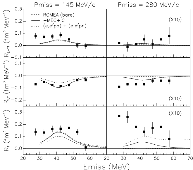
FIG. 23: Data from this work together with ROMEA calculations by the Ghent Group for the E_{\text{miss}} -dependence of the R_{L+TT} , R_{LT} , and R_T response functions. Error bars are statistical (see Tables XXVII, XXVIII, and XXVI for the associated systematic uncertainties). Also shown is the (e, e'pX) contribution.
