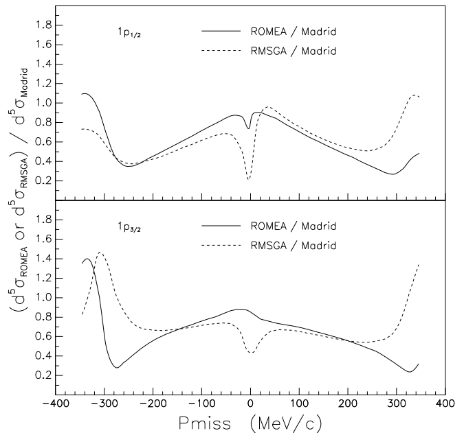
FIG. 9: Baseline RDWIA calculations by the Madrid Group compared to “bare” (no MEC nor IC) ROMEA and RMSGA calculations by the Ghent Group for the removal of protons from the 1p -shell of ^{16}\text{O} as a function of P_{\text{miss}} for E_{\text{beam}} = 2.442 GeV. Overall agreement is reasonable, particularly for |P_{\text{miss}}| < 200 MeV/c.
