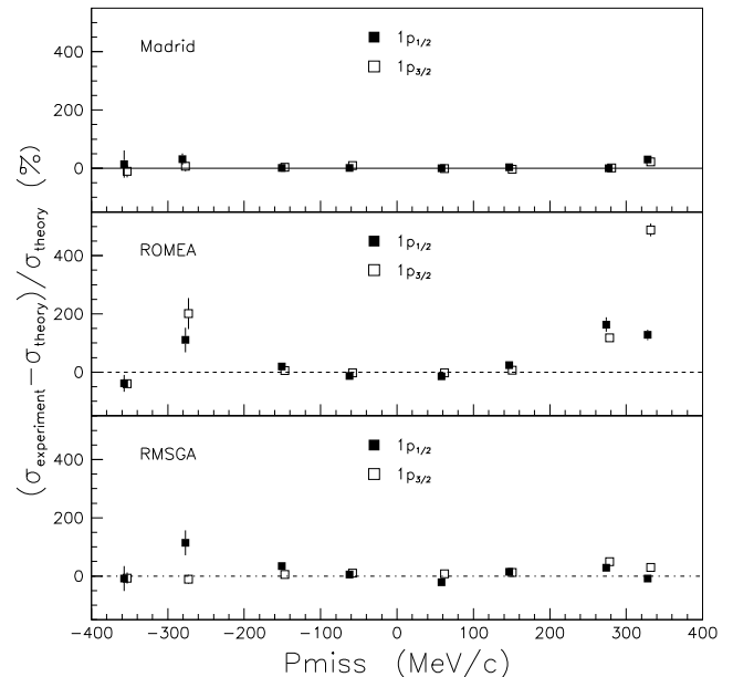
FIG. 13: Measured cross sections for the removal of protons from the 1p -shell of ^{16}\text{O} as a function of P_{\text{miss}} as compared to relativistic calculations at E_{\text{beam}} = 2.442 GeV. Error bars are statistical, and on average, there is an additional \pm 5.6\% systematic uncertainty (see Table XII) associated with the data. The top panel is the RDWIA calculation of the Madrid Group, while the middle and bottom panels are respectively the “bare” (no MEC nor IC) ROMEA and RMSGA calculations of the Ghent Group.
