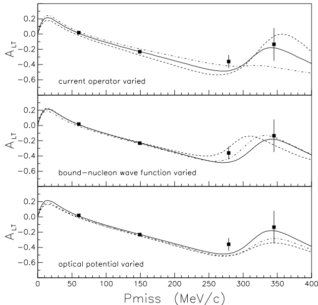
FIG. 16: Left-right asymmetry A_{LT} together with relativistic calculations for the removal of protons from the 1p_{1/2} -state of ^{16}\text{O} as a function of P_{\text{miss}} for E_{\text{beam}} = 2.442 GeV. Error bars are statistical (see Table XXV for the associated systematic uncertainties). The RDWIA calculations are by the Madrid Group. The solid curves in all three panels are the same and are identical to those shown for the removal of protons from the 1p_{1/2} -state of ^{16}\text{O} in Figures 14 and 15.
