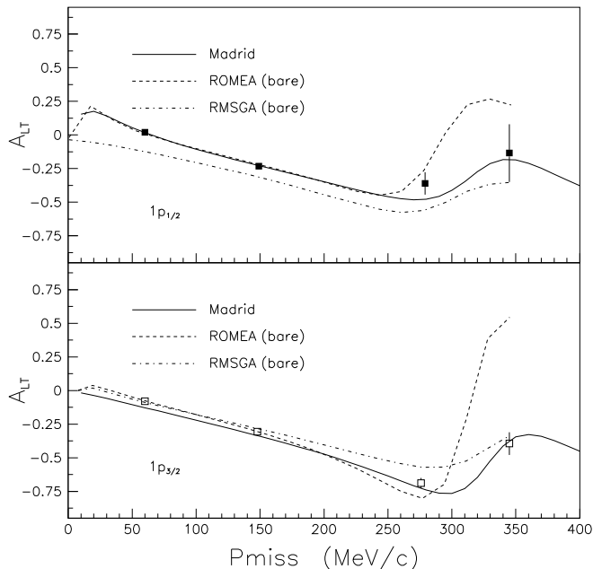
FIG. 14: Left-right asymmetry A_{LT} together with relativistic calculations of the A_{LT} asymmetry for the removal of protons from the 1p -shell of ^{16}\text{O} as a function of P_{\text{miss}} for E_{\text{beam}} = 2.442 GeV. Error bars are statistical (see Table XXV for the associated systematic uncertainties). The solid line is the RDWIA calculation of the Madrid Group, while the dashed and dashed-dotted lines are respectively the “bare” (no MEC nor IC) ROMEA and RMSGA calculations of the Ghent Group.
