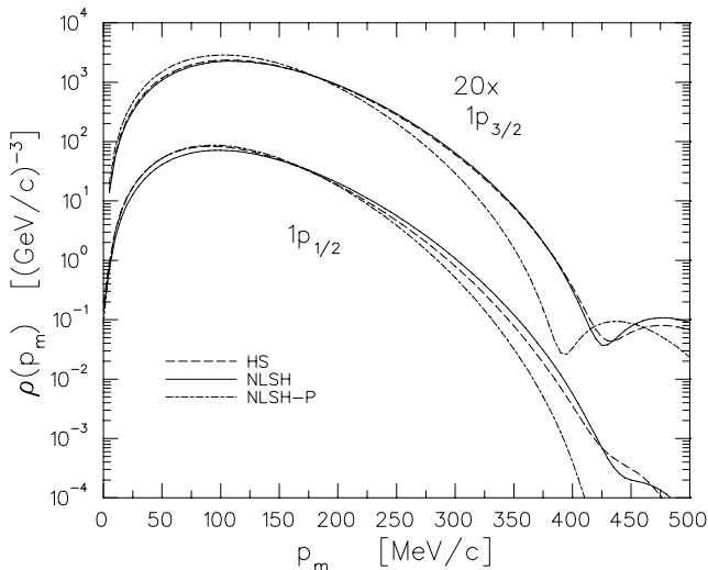
FIG. 10: PWIA momentum distributions for the HS, NLSH, and NLSH-P models. Appreciable difference exists for the 1p_{3/2} -state distributions, but there is little to distinguish between the 1p_{1/2} -state distributions. Note that the NLSH and NLSH-P wave functions predict binding energies, single-particle energies, and a charge radius for ^{16}\text{O} which are all in good agreement with the data.
