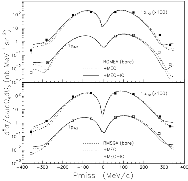
FIG. 18: Measured cross sections for the removal of protons from the 1p -shell of ^{16}\text{O} as a function of P_{\text{miss}} together with calculations by the Ghent Group at E_{\text{beam}} = 2.442 GeV. Error bars are statistical, and on average, there is an additional \pm 5.6\% systematic uncertainty (see Table XII). The curves labelled “bare” are identical to those shown in Figure 12.
