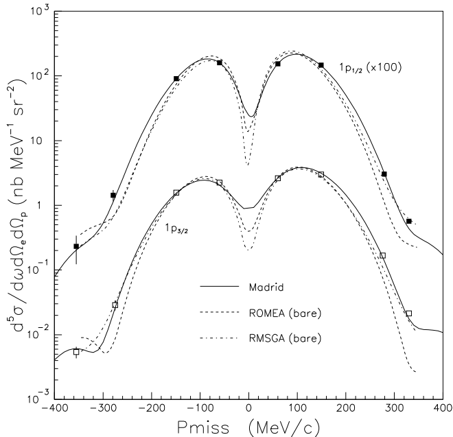
FIG. 12: Measured cross sections for the removal of protons from the 1p -shell of ^{16}\text{O} as a function of P_{\text{miss}} as compared to relativistic calculations at E_{\text{beam}} = 2.442 GeV. Error bars are statistical, and on average, there is an additional \pm 5.6\% systematic uncertainty (see Table XII) associated with the data. The solid line is the RDWIA calculation of the Madrid Group, while the dashed and dashed-dotted lines are respectively the “bare” (no MEC nor IC) ROMEA and RMSGA calculations of the Ghent Group.
