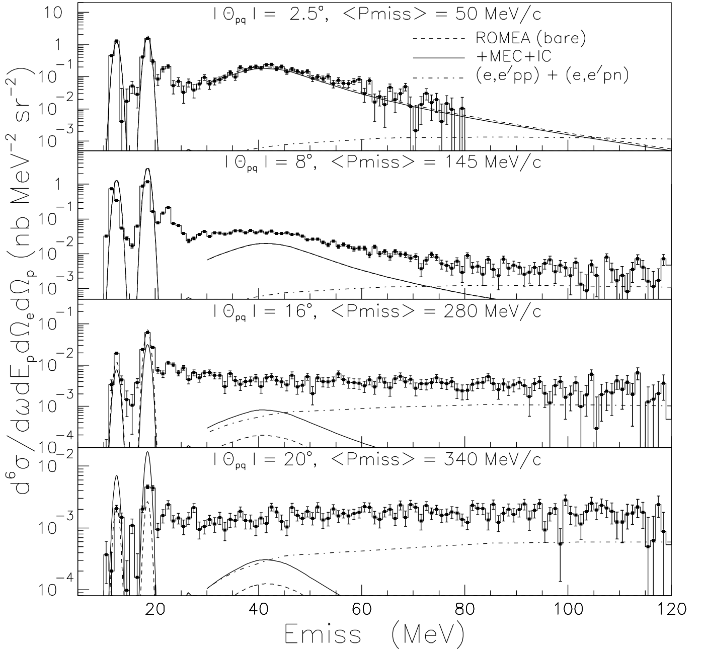
FIG. 22: Data from this work together with ROMEA calculations by the Ghent Group for the E_{\text{miss}} -dependence of the cross sections obtained at E_{\text{beam}} = 2.442 GeV. The data are the average cross sections measured on either side of \vec{q} at each \theta_{pq} . Error bars are statistical and on average, there is an additional \pm 5.9\% systematic uncertainty (see Tables XVIII – XXII) associated with the data. Also shown are calculations by the Ghent Group for the (e, e'pp) and (e, e'pn) contributions to the (e, e'p) cross section.
