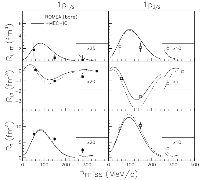
FIG. 20: Data from this work together with ROMEA calculations by the Ghent Group for the R_{L+TT} , R_{LT} , and R_T response functions for the removal of protons from the 1p -shell of ^{16}\text{O} as a function of P_{\text{miss}} . Error bars are statistical (see Tables XXIV, XXV, and XXIII for the associated systematic uncertainties). The curves labelled “bare” are identical to those shown in Figure 17.
