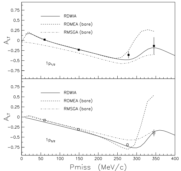
FIG. 15: Left-right asymmetry A_{LT} together with relativistic calculations of the A_{LT} asymmetry for the removal of protons from the 1p -shell of ^{16}\text{O} as a function of P_{\text{miss}} for E_{\text{beam}} = 2.442 GeV. Error bars are statistical (see Table XXV for the associated systematic uncertainties). The solid line is the RDWIA calculation, while the dashed and dashed-dotted lines are respectively the “bare” (no MEC nor IC) ROMEA and RMSGA calculations.
