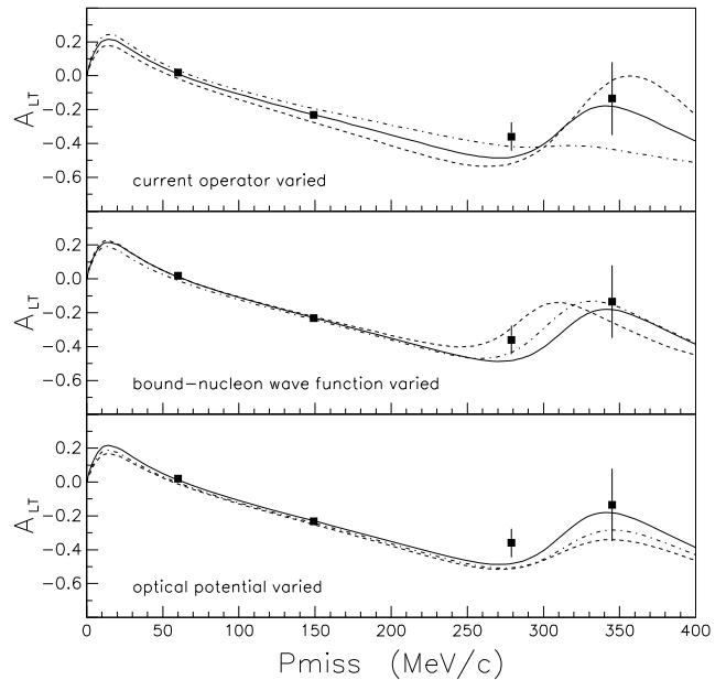
FIG. 17: Left-right asymmetry A_{LT} together with RDWIA calculations for the removal of protons from the 1p_{1/2} -state of ^{16}\text{O} as a function of P_{\text{miss}} for E_{\text{beam}} = 2.442 GeV. Error bars are statistical (see Table XXV for the associated systematic uncertainties). The solid curves in all three panels are the same and are identical to those shown for the removal of protons from the 1p_{1/2} -state of ^{16}\text{O} in Figures 15 and 16.
