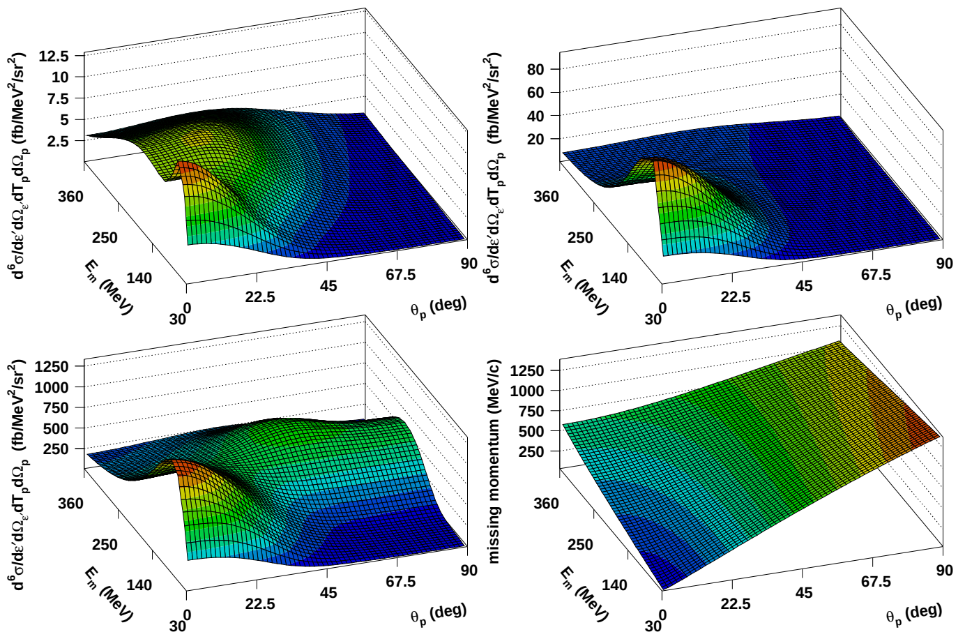
FIG. 25: Calculations by the Ghent Group [99] of the contribution to the differential ^{16}\text{O}(e, e'p) cross section from two-nucleon knockout as a function of E_{\text{miss}} and \theta_p for E_{\text{beam}} = 2.442 GeV. The upper-left panel shows the contribution of central correlations. The upper-right panel shows the combined contribution of central and tensor correlations. The lower-left panel shows the combined contribution of central and tensor correlations (two-nucleon correlations) together with MEC and IC (two-body currents). The relationship between the various kinematic quantities is shown in the bottom-right panel.
