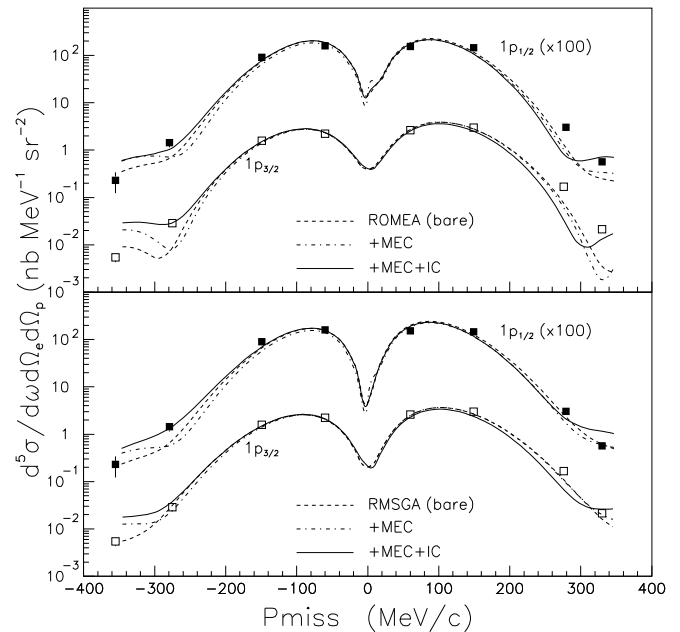
FIG. 19: Measured cross sections for the removal of protons from the 1p -shell of ^{16}\text{O} as a function of P_{\text{miss}} together with calculations by the Ghent Group at E_{\text{beam}} = 2.442 GeV. Error bars are statistical, and on average, there is an additional \pm 5.6\% systematic uncertainty (see Table XII). The curves labelled “bare” are identical to those shown in Figure 13.
