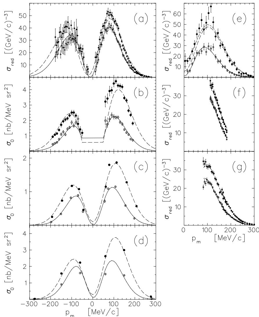
FIG. 12: Fits to various ^{16}\text{O}(e, e'p) data sets based on the NLSH bound-nucleon wave function and the EDAL-O optical potential. Open points and solid lines pertain to the 1p_{1/2} -state, while solid points and dashed lines pertain to the 1p_{3/2} -state. The dashed-dotted lines include the contributions of the 2s_{1/2}1d_{5/2} -doublet to the 1p_{3/2} -state. Panel (d) shows the data from this work - see Table VII for the key to the other data sets.
