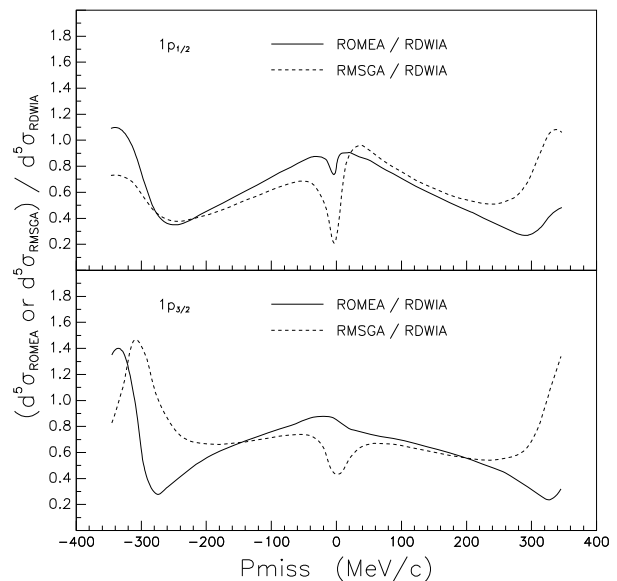
FIG. 10: Baseline RDWIA calculations compared to “bare” (no MEC nor IC) ROMEA and RMSGA calculations by the Ghent Group for the removal of protons from the 1p -shell of ^{16}\text{O} as a function of P_{\text{miss}} for E_{\text{beam}} = 2.442 GeV.
