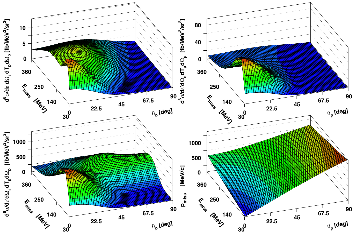
FIG. 23: Calculations by the Ghent Group of the contribution to the differential ^{16}\text{O}(e, e'p) cross section from two-nucleon knockout as a function of E_{\text{miss}} and \theta_p for E_{\text{beam}} = 2.442 GeV. The upper-left panel shows the contribution of central correlations. The upper-right panel shows the combined contribution of central and tensor correlations. The lower-left panel shows the combined contribution of central and tensor correlations (two-nucleon correlations) together with MEC and IC (two-body currents). The relationship between the various kinematic quantities is shown in the bottom-right panel.
