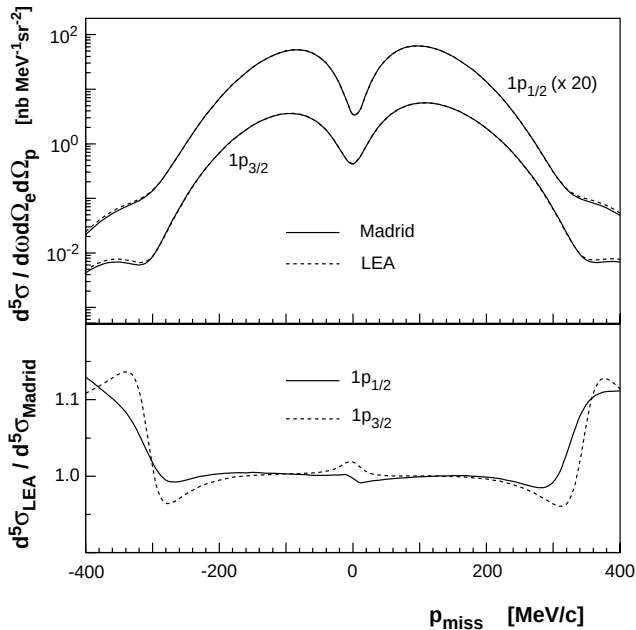
FIG. 8: Comparison baseline RDWIA calculations by the Madrid Group and Kelly (LEA) for the removal of protons from the 1p -shell of ^{16}\text{O} as a function of p_{\text{miss}} for E_{\text{beam}} = 2.442 GeV. For the purposes of this comparison, the input into both calculations was identical (see Table V). Overall agreement is very good, and agreement is excellent for -250 MeV/ c < p_{\text{miss}} < 250 MeV/ c .
