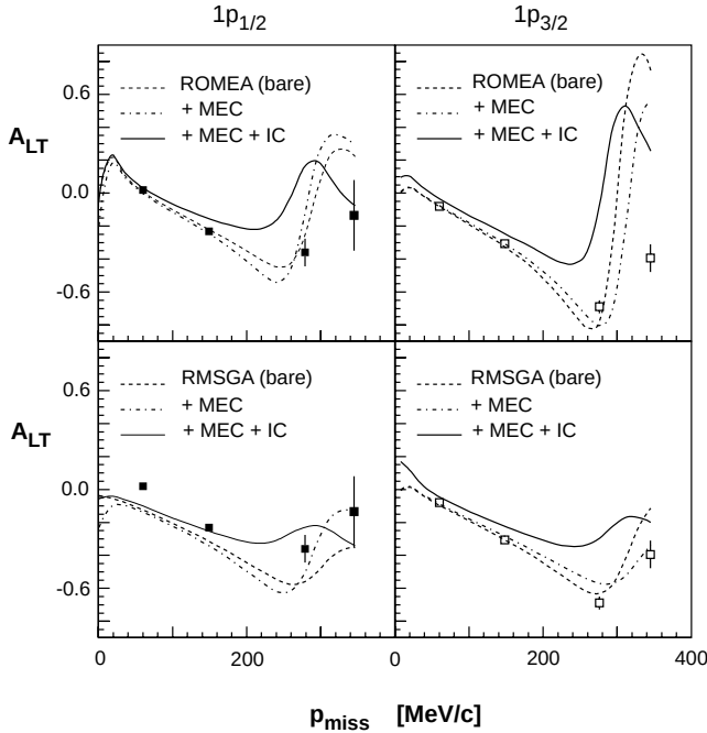
FIG. 18: Left-right asymmetry A_{LT} together with calculations by the Ghent Group of the A_{LT} asymmetry for the removal of protons from the 1p -shell of ^{16}\text{O} as a function of p_{\text{miss}} for E_{\text{beam}} = 2.442 GeV. Error bars are statistical (see Table XXV for the associated systematic uncertainties). The curves labelled ‘bare’ are identical to those shown in Fig. 15.
