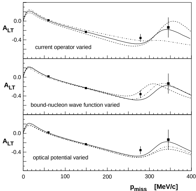
FIG. 13: Left-right asymmetry A_{LT} together with RDWIA calculations for the removal of protons from the 1p_{1/2} -state of ^{16}\text{O} as a function of p_{\text{miss}} for E_{\text{beam}} = 2.442 GeV. Uncertainties are statistical (see Table XXV for the associated systematic uncertainties). The solid curves in all three panels are the same and are identical to those shown for the removal of protons from the 1p_{1/2} -state of ^{16}\text{O} in Figs. 12 and 15.
